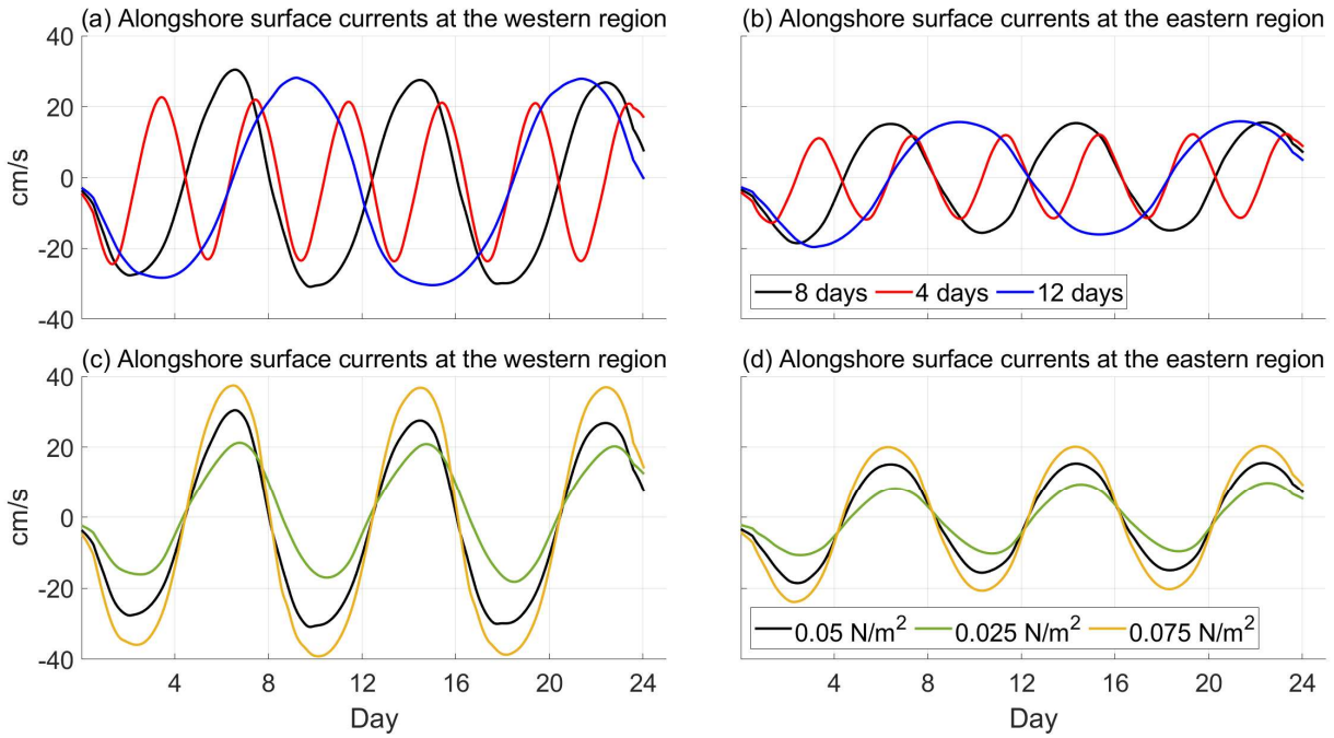
290 Figure 13: Alongshore surface currents at the (a, c) western and (b, d) eastern regions (blue and orange crosses in Fig. 1b) from 300 sensitivity experiments under (a, b) varying wind periods and (c, d) varying wind stress amplitudes.
