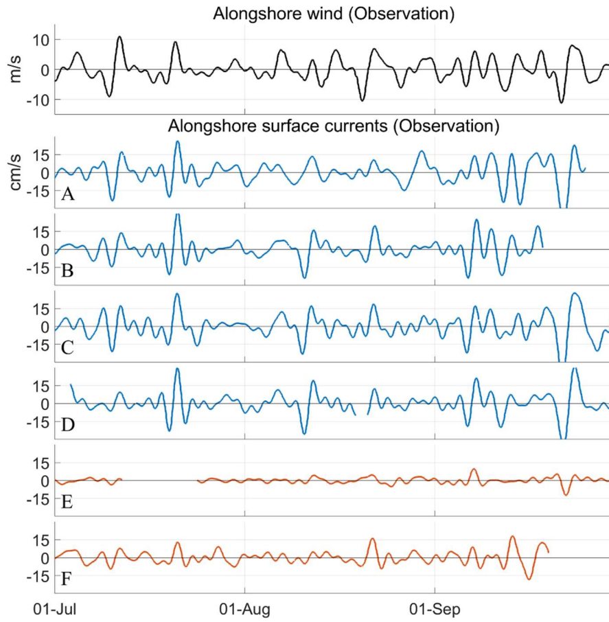
Figure 2: Alongshore wind velocity (black line) and alongshore surface currents observed at the stations shown in Fig. 1a. Stations A–F correspond to the dots in Fig. 1a from west to east. Blue and orange colors indicate stations located in the western and eastern regions of the bank, respectively.
