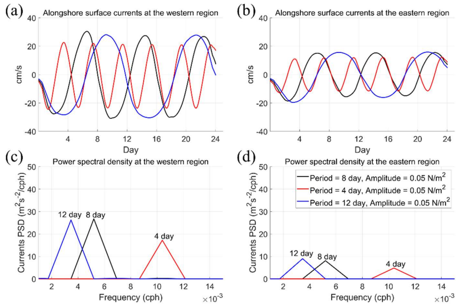
Figure 13: Alongshore surface currents at the (a) western and (b) eastern regions (blue and orange crosses in Fig. 1b), and power spectral densities at the (c) western and (d) eastern regions (blue and orange crosses in Fig. 1b) under various wind periods.
