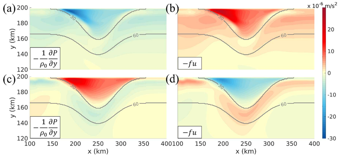
195 Figure 7: Cross-shore depth-averaged momentum balances calculated from the idealized model results during (top) westward winds on day 18 and (bottom) eastward winds on day 22. Gray contours represent the bottom topography, with depths indicated in meters.
