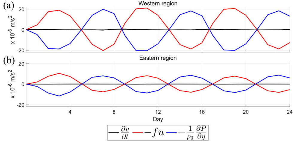
200 Figure 8: Time series of cross-shore depth-averaged momentum balance terms from the idealized model results at the (a) western and (b) eastern regions (blue and orange crosses in Fig. 1b).
