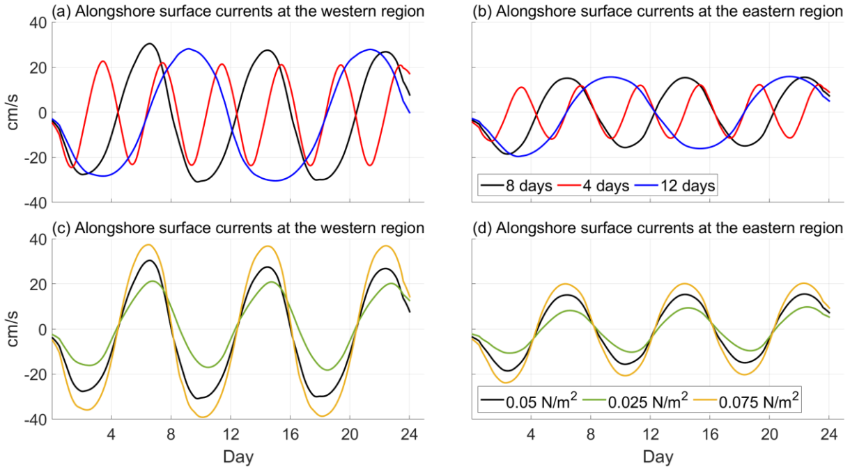
Figure 13: Alongshore surface currents at the (a, c) western and (b, d) eastern regions (blue and orange crosses in Fig. 1b) from sensitivity experiments under (a, b) varying wind periods and (c, d) varying wind stress amplitudes.
