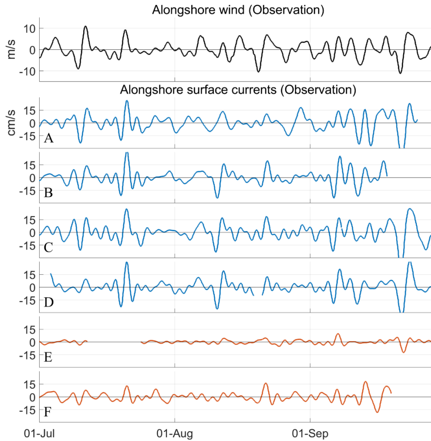
Figure 2: Alongshore wind velocity (black line) and alongshore surface currents observed at the stations shown in Fig. 1a in the year 2019 . Stations A–F correspond to the dots in Fig. 1a from west to east. Blue and orange colors indicate stations located in the western and eastern regions of the bank, respectively.
