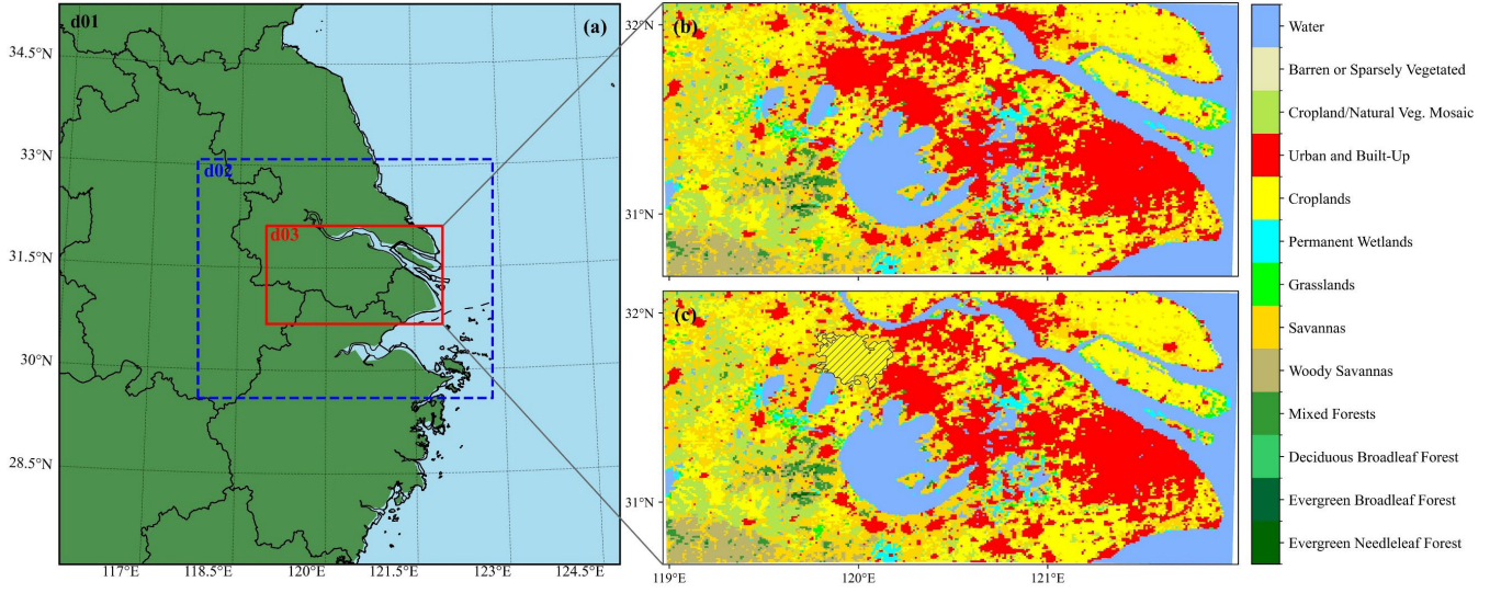
Figure 2. (a) The setup of the nested domain over the study area. Land use and land cover within the innermost domain for (b) control simulation and (c) sensitivity experiment. In (c), the solid black lines and diagonal hatching represent the areas where the land use and land cover were modified.
