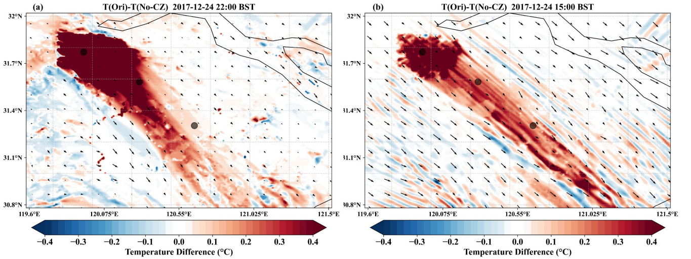
Figure 10. Spatial distribution of the 2-meter temperature difference between the control simulation and the sensitivity experiment (CTRL minus EXP) at (a) 22:00 BST and (b) 15:00 BST. Vector arrows indicate the 10-meter wind field of the CTRL. The three marked locations from northwest to southeast correspond to downtown areas of Changzhou (U2), Wuxi (U4), and Suzhou (U6), respectively.
