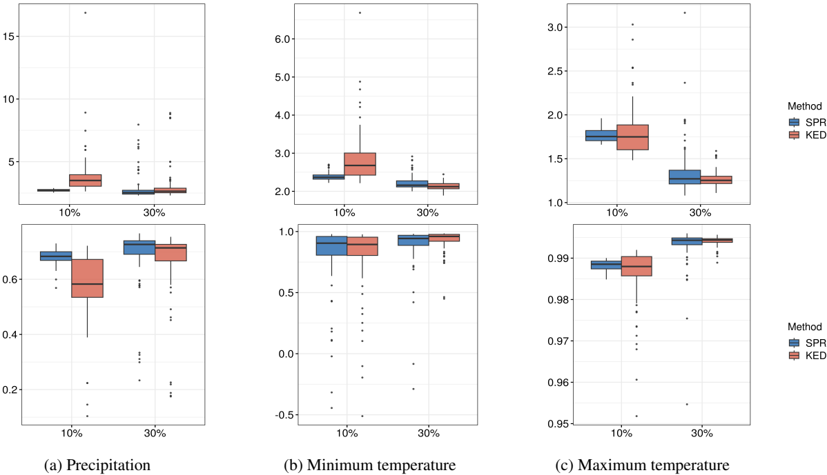
Figure 7. Validation with real observations: distribution of mean daily RMSE (first row) and SSIM (second row) across 100 independent random station samplings for SPR and KED, for each variable. Each box shows the median, interquartile range, and whiskers extending to 1.5 times the interquartile range. Lower RMSE and higher SSIM indicate better performance. Note that 10% density corresponds to 2–4 stations in a region of 70,000 km 2 .
