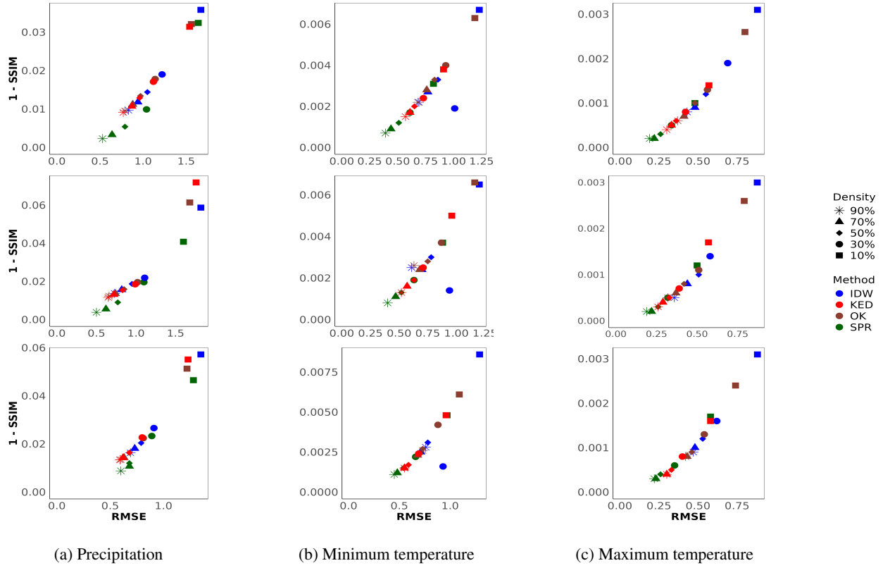
Figure 3. Synthetic data experiments: Comparison of the three baseline methods and SPR in the southern region, in terms of averaged RMSE (x-axis) and averaged 1-SSIM (y-axis). Each column represents a specific meteorological variable, while each row corresponds to a region size—ranging from the largest at the top to the smallest at the bottom. Each color represents a different interpolation method, and each plotting symbol corresponds to a specific network density. The closer a symbol is to the origin, the better the performance.
