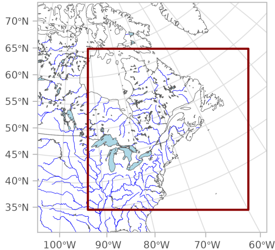
(a) North American domain of the ClimEx project (dark red rectangle).
