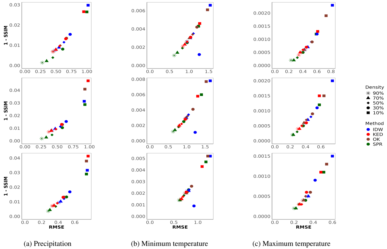
Figure 4. Synthetic data experiments: Comparison of the three baseline methods and SPR in the northern region, in terms of RMSE (x-axis) and 1-SSIM (y-axis). Each column represents a specific meteorological variable, while each row corresponds to a region size—ranging from the largest at the top to the smallest at the bottom. Each color represents a different interpolation method, and each plotting symbol corresponds to a specific network density. The closer a symbol is to the origin, the better the performance.
