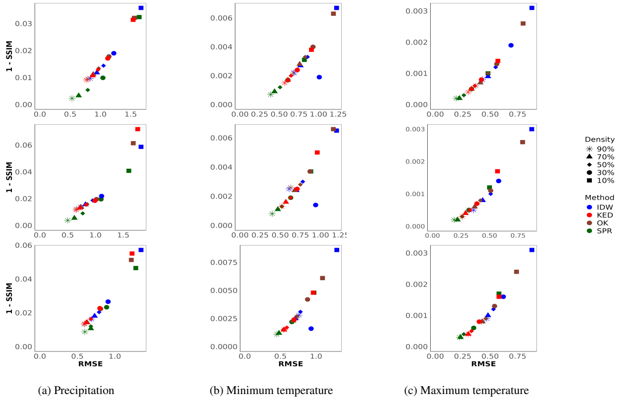
Figure 3. Synthetic data experiments : Comparison of the three baseline methods and SPR in the southern region, in terms of averaged RMSE (x-axis) and averaged 1-SSIM (y-axis). Each column represents a specific meteorological variable, while each row corresponds to a region size—ranging from the largest at the top to the smallest at the bottom. Each color represents a different interpolation method, and each plotting symbol corresponds to a specific network density. The closer a symbol is to the origin, the better the performance.
