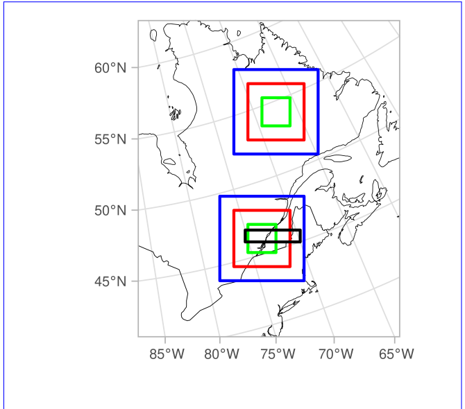
(b) Two study regions—referred to as the south and north regions—within the domain outlined in Fig. 1a, shown at three different sizes (in different colours). The black rectangle indicates the spatial domain of the real-data experiments.
