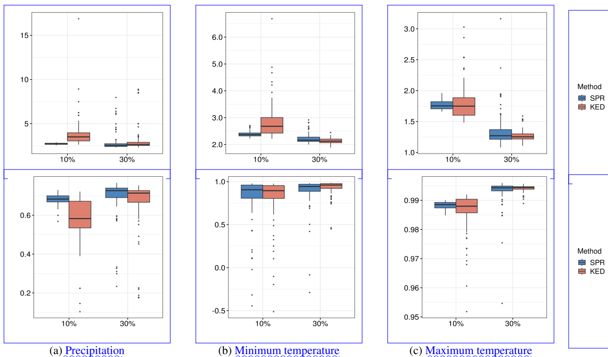
Figure 7. Validation with real observations: distribution of mean daily RMSE statistics -(mean, median, standard deviation (SD) first row) and 2.5%-and-97.5%-quantiles SSIM (second row) across 100 independent random station samplings for SPR and average SSIM values-KED , for each variable. Each box shows the median, interquartile range, and interpolation-method whiskers extending to 1.5 times the interquartile range . Lower RMSE and higher SSIM values indicate better performance. Note that 10% density correspond-corresponds to 2-4 station-2-4 stations in a region of 70.000km 2 70.000 km 2 .
