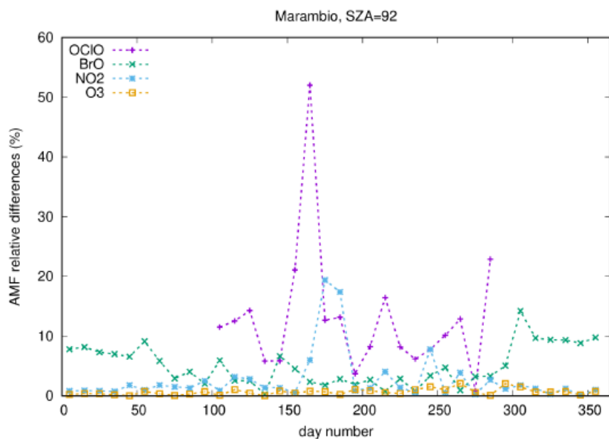
Figure 7: Top panel: OCIO (violet), BrO (green), NO 2 (blue) and O 3 (yellow) stratospheric AMFs computed for Marambio, for SZA=92°, and surface albedo=0. Continuous lines correspond to monthly averaged values; dashed lines correspond to 10-day averaged values. Bottom panel: Relative difference between monthly and 10-day averaged AMFs: OCIO (violet), BrO (green), NO 2 (blue) and O 3 (yellow). Note that for OCIO only the period in which it is observed is shown in the figure.
