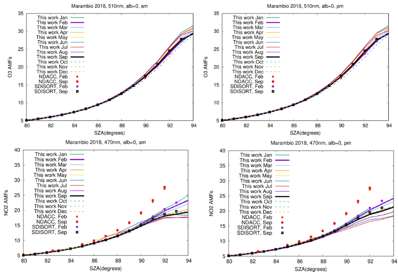
Figure 8: Total Visible AMFs: O 3 (first row), NO 2 (second row) computed for Marambio 2018, for surface albedo=0: Sunrise values at left and sunset values at right. Red symbols correspond to NDACC AMFs for O 3 and NO 2 [Hendrick et al, 2011]. 2D-DISORT AMFs for February (violet crosses) and September (black squares) are also shown.
