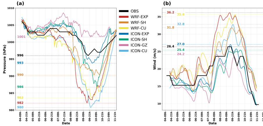
Figure 5. Timeseries of the cyclone variables: (a) CSLP every 6h for observation and 1h for the simulations; (b) Maximum wind speed within a radius of 150 km from cyclone center every 6 h for observation and 1 h for simulations using a 6 h running mean. WRF-EXP in red, WRF-SH in orange, WRF-CU in yellow; ICON-EXP in blue, ICON-SH in green, ICON-GZ in magenta, ICON-CU in light-blue. Reference behaviour of the observations in black
