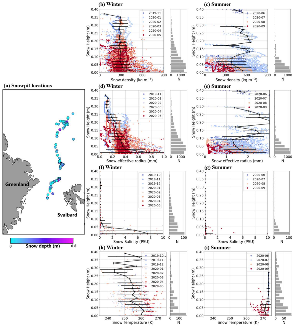
Figure 2: Stratified measurements of snow properties collected during the MOSAiC expedition. (a) snowpit locations (b-c) snow density; (d-e) Snow effective radius; (f-g): Snow salinity; (h-i): Snow temperature. Color points indicate measurements for each month, and black lines represent the ensemble central tendency of the corresponding profiles. The horizontal bars represent the standard deviation. The grey histograms on the right indicate the number of observations within each snow-height layer.
