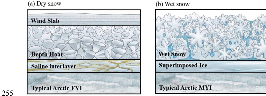
Figure 1: Conceptual diagrams of dry snow and wet snow layering over Arctic sea ice.
