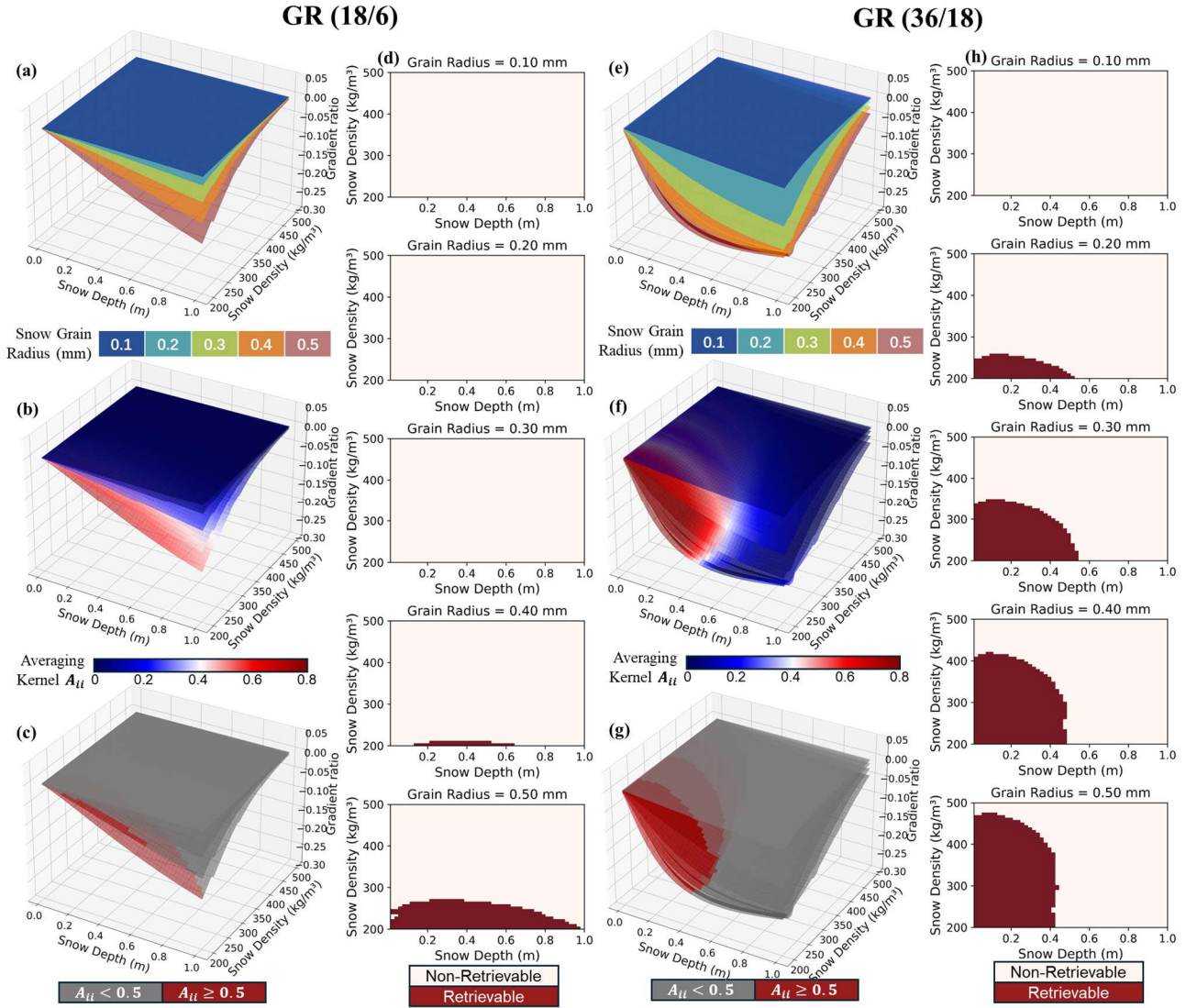
555 Figure 7: Retrieval of snow depth with GR(18/6) (a-d) and GR(36/18) (e-h) on different snow density and grain radius (Snow temperature = 260 K, Stickiness = 0.1).
