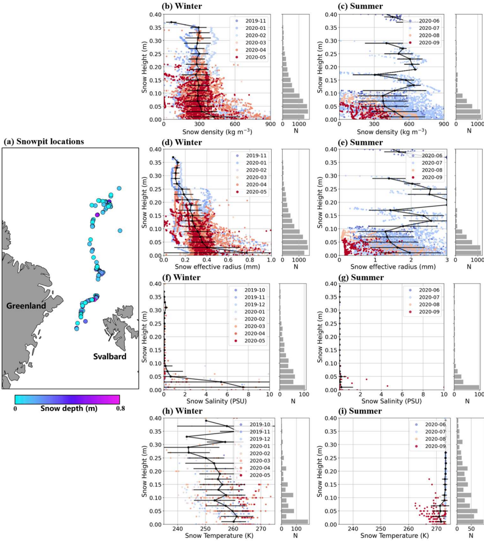
Figure 2: Stratified measurements of snow properties collected during the MOSAiC expedition. (a) locations of snowpit (b-c) snow density; (d-e) Snow effective radius; (f-g): Snow salinity; (h-i): Snow temperature. Color points indicate measurements for each month, and black lines represent the ensemble central tendency of the corresponding profiles. The horizontal bars represent the standard deviation. The grey histograms on the right indicate the number of observations within each snow-height layer.
