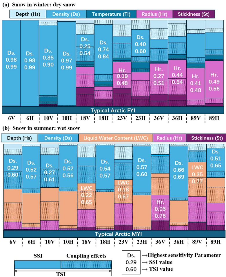
Figure 3: EFAST sensitivity result of single-layer Arctic snow parameters for the AMSR2 channels under dry snow (a) and wet snow (b) conditions. Solid segments indicate the SSI of each parameter, while dotted extensions show the coupling effects captured by the TSI. For each channel (column), the strongest single sensitivity and the total sensitivity are also given numerically.
