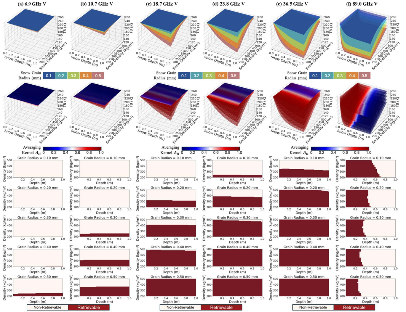
505 Figure 6: Retrieval of snow depth at 6 - 89 GHz V-pol channels. Top row: TB as a function of snow depth and density for different snow grain radius. Second row: corresponding diagonal averaging kernel element A_{ii} for snow depth. Bottom rows: retrievable ranges for discrete snow grain radius, defined as the projection onto the X-Y plane of the corresponding radius layers where the A_{ii} exceeds 0.5.
