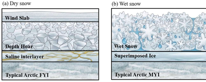
Figure 1: Conceptual diagrams of dry snow and wet snow layering over Arctic sea ice.
