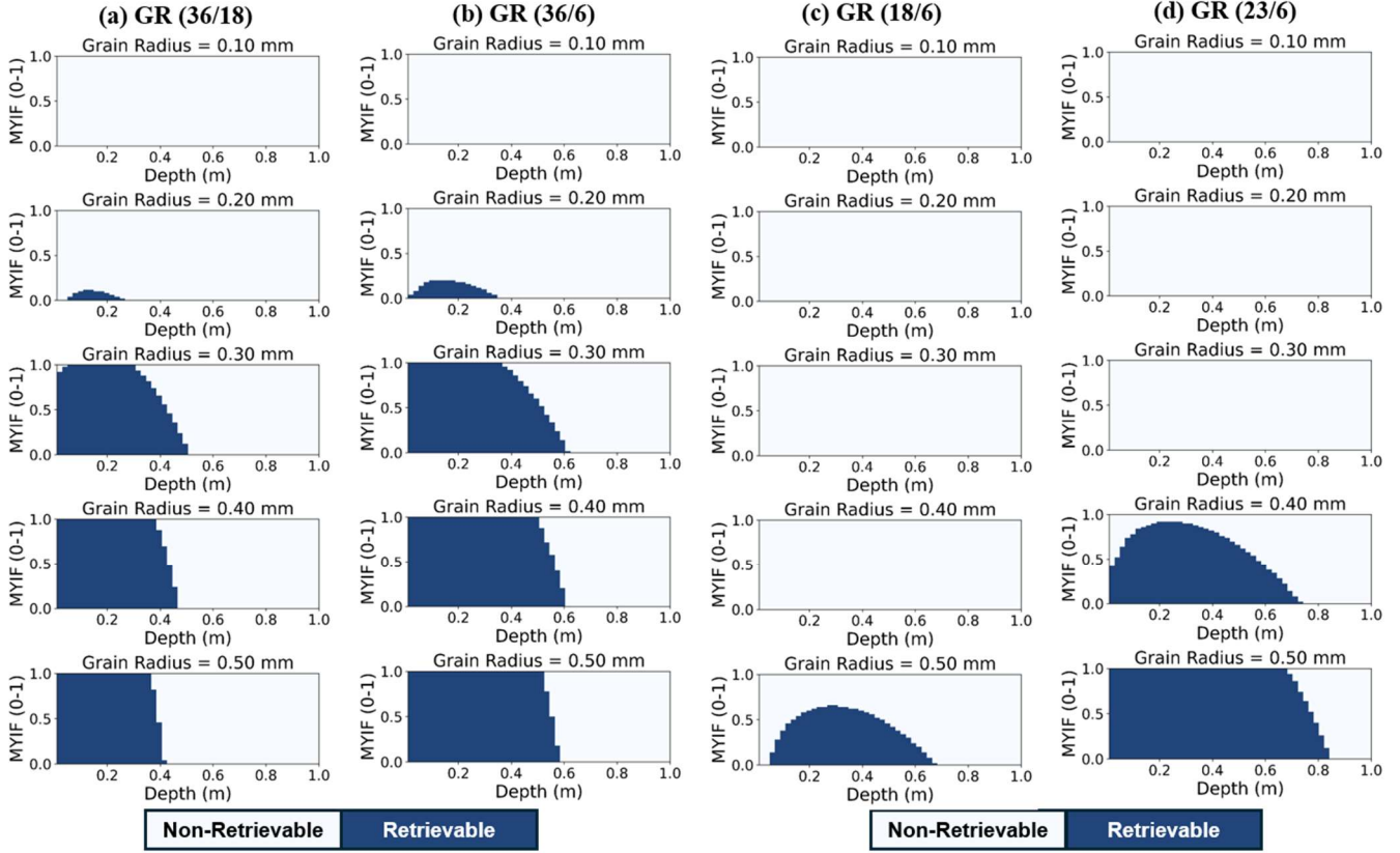
Figure 9: Retrievability of snow depth with GR(36/18), GR(36/6), GR(18/6) and GR(23/6) on different MYIF and grain radius. The corresponding 3D TB plots can be found in the Supplementary Materials.
