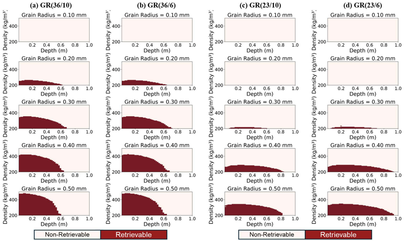
Figure 8: Retrieval of snow depth with GR(36/10), GR(36/6), GR(23/10) and GR(23/6) on different snow density and grain radius (Snow temperature = 260 K, Stickiness = 0.1). The corresponding 3D TB plots can be found in the Supplementary Materials.
