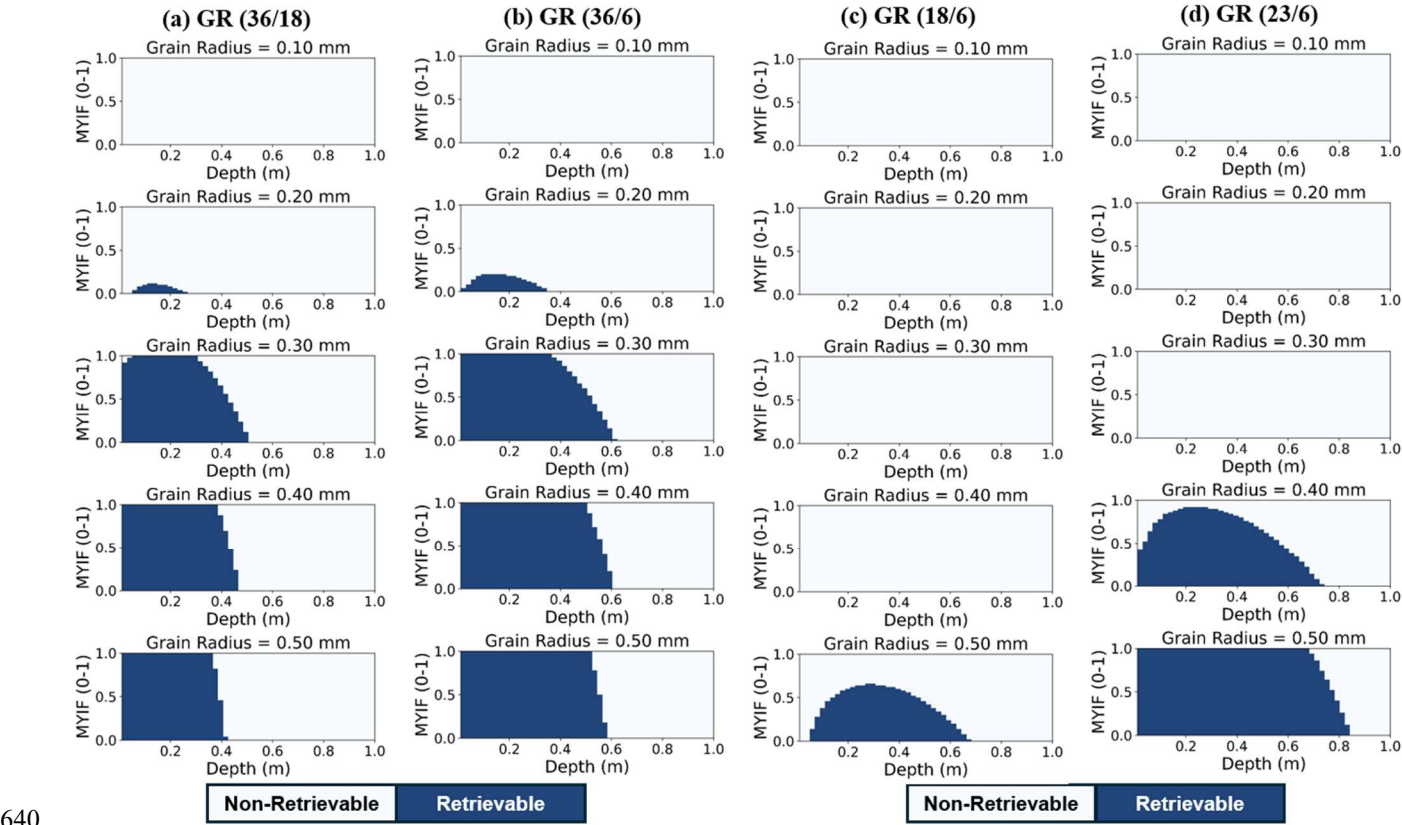
Figure 9: Retrieval of snow depth with GR(36/18), GR(36/6), GR(18/6) and GR(23/6) on different MYIF and grain radius. The corresponding 3D TB plots can be found in the Supplementary Materials.
