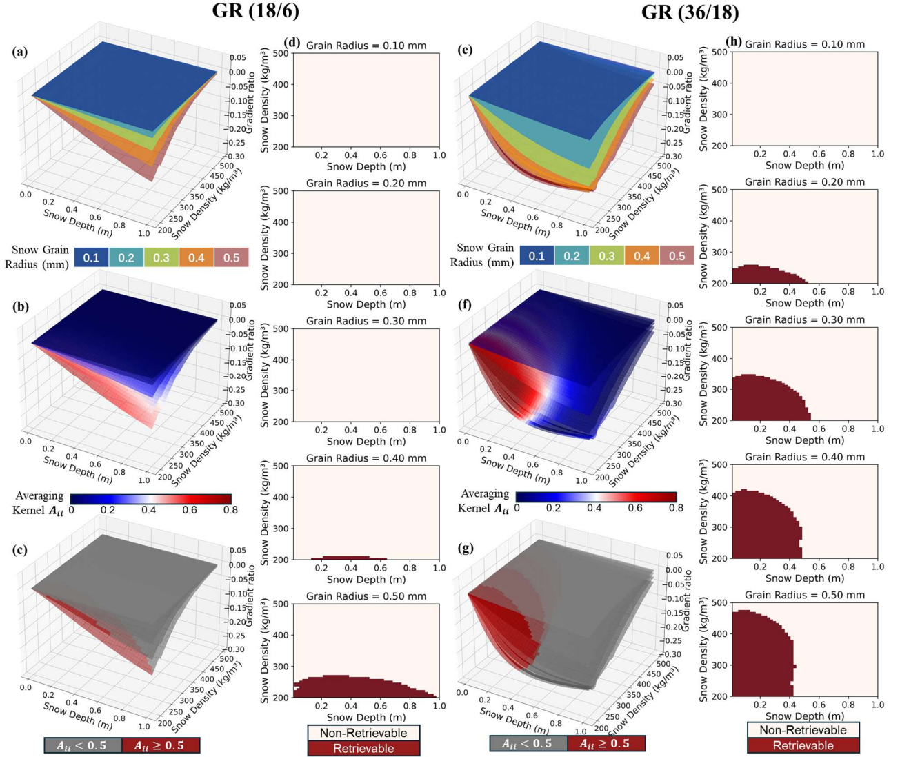
575 Figure 7: Retrieval of snow depth with GR(18/6) (a-d) and GR(36/18) (e-h) on different snow density and grain radius (Snow temperature = 260 K, Stickiness = 0.1).
