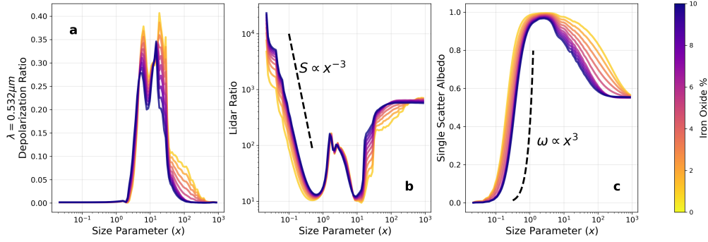
Figure 3. Single-particle backscattering properties for spheroidal dust particles with aspect ratio 1.5 calculated via the triaxial ellipsoid database at 532 nm. Panels show the evolution of (a) depolarization ratio, (b) lidar ratio, and (c) single-scattering albedo as a function of size parameter.
