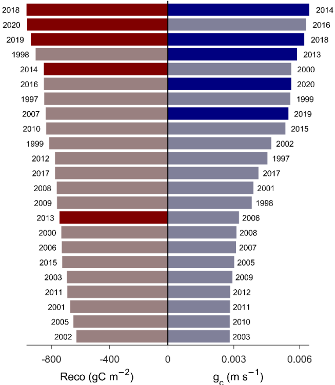
Figure 7: Cumulative ecosystem respiration (Reco, left side) and canopy conductance (g c , right side) integrated over the IPeak integration period (SOS to SOS+120). Years are ranked independently for each variable in decreasing order of magnitude. Each horizontal bar represents a single year, with labels positioned on the corresponding side of the axis. Extreme-summer years (2013, 2014, 2018, 2019 and 2020) are highlighted using darker colors, whereas all other years are shown with lighter shades. A vertical line separates the two variables for clarity.
