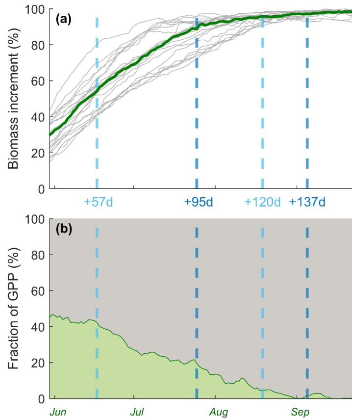
405 Figure 5: Effect of precipitation on tree physiological responses. Vertical dashed lines indicate the long-term correlation windows for P with IPeak (SOS+57 to SOS+120, light blue) and IRise (SOS+95 to SOS+137, dark blue). Average calendar dates marking the start of each month (computed across all years) are shown in green. (a) Temporal evolution of median daily biomass accumulation expressed as a proportion of total annual storage. Individual yearly trajectories are shown in grey and the multi-year median is shown in green. (b) Daily fraction of GPP allocated to biomass storage (light green) versus other metabolic or structural processes (dark gray).
