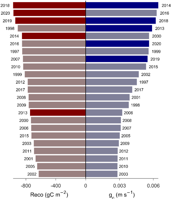
455 Figure 7: Cumulative ecosystem respiration (Reco, left side) and canopy conductance (g c , right side) integrated over the IPeak integration period (SOS to SOS+120). Years are ranked independently for each variable in decreasing order of magnitude. Each horizontal bar represents a single year, with labels positioned on the corresponding side of the axis. A vertical line separates the two variables for clarity.
