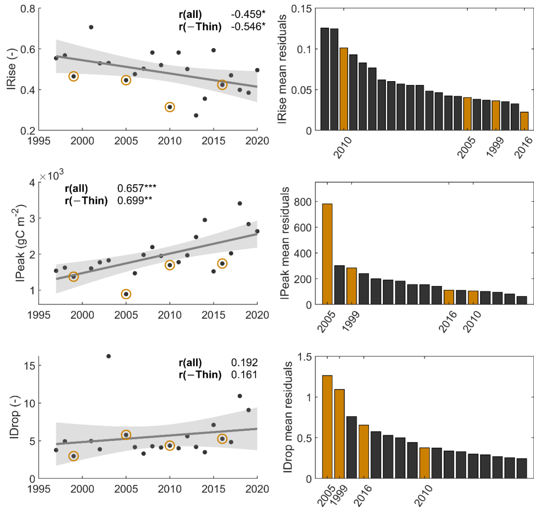
Figure 3: Left panels: Temporal trajectories of the three GPP phenological indicators (IRise, IPeak, IDrop) over the 24-year observation period. Each panel shows the fitted linear regression (solid line) with its 95 % confidence interval (shaded area). Years during which thinning operations were conducted are highlighted with yellow circles. Correlation coefficients are reported both for the full time series and for the subset excluding thinning years. Statistical significance is denoted by one, two or three stars for p \leq 0.05 , 0.01 and 0.001 , respectively. Indicators represent wavelet-derived metrics and should be interpreted comparatively. Right panels: Mean residuals from significant linear relationships between each indicator and its associated environmental drivers. Residuals represent deviations from expected forest functional responses based on these relationships. Thinning years are shown as yellow bars. Years are ordered by decreasing mean residual importance. Extreme years for IPeak (2013, 2014, 2018, 2019, 2020) and IDrop (2003, 2015, 2018, 2020) were removed prior to computing residual means.
