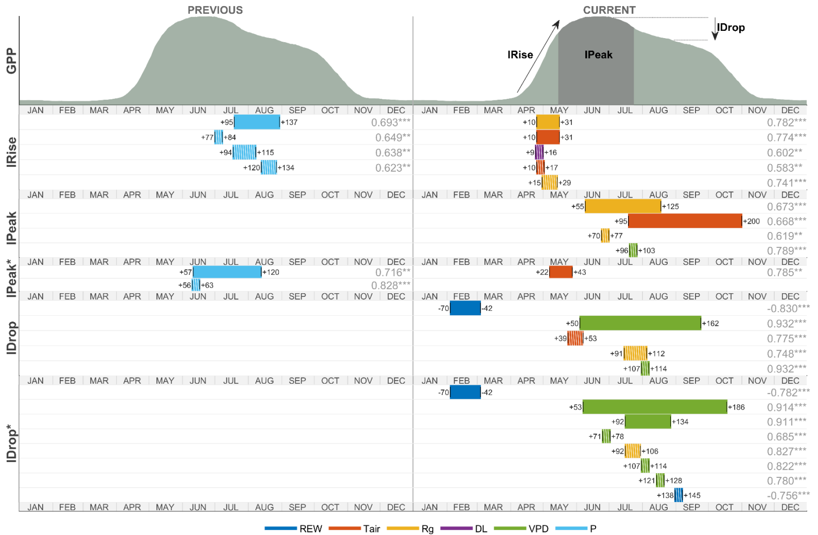
Figure 4: Influence of environmental drivers on GPP seasonal dynamics. The upper panel shows modelled GPP (following Bitton et al., 2026) for the previous and current year, together with a schematic representation of the three seasonal indicators. The lower panels depict, for each indicator and its modified variants (IPeak* excluding thinning and extreme-summer years; IDrop* excluding the exceptional 2003 drought year), the time windows during which each environmental driver is most strongly correlated with the indicator. Windows are presented in chronological order, with long-scale effects (filled bars) displayed above short-scale effects (hatched bars). Window boundaries are expressed in days relative to SOS. Colors represent the different drivers and correlation coefficients with their significance levels (stars indicating p \leq 0.05 , p \leq 0.01 and p \leq 0.001 ) are shown next to each bar. Previous-year effects appear to the left of the vertical divider and current-year effects to the right.
