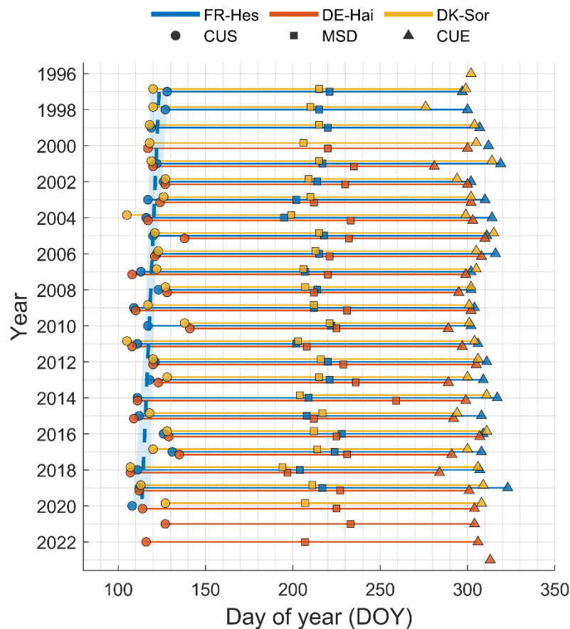
555 Figure 10: Phenological markers for the three forest sites (FR-Hes, DE-Hai and DK-Sor). Years are displayed on the vertical axis (in reversed chronological order) and day of year (DOY) on the horizontal axis. Marker shape differentiates three phenological events: carbon uptake start (CUS, circle), mid-season drop (MSD, square) or carbon uptake end (CUE, triangle). Horizontal segments connect events within each year. Linear temporal trends are shown (in dashed lines) only when the regression slope is statistically significant ( p \leq 0.05 ). Shaded bands represent 95 % confidence intervals around significant regression lines.
