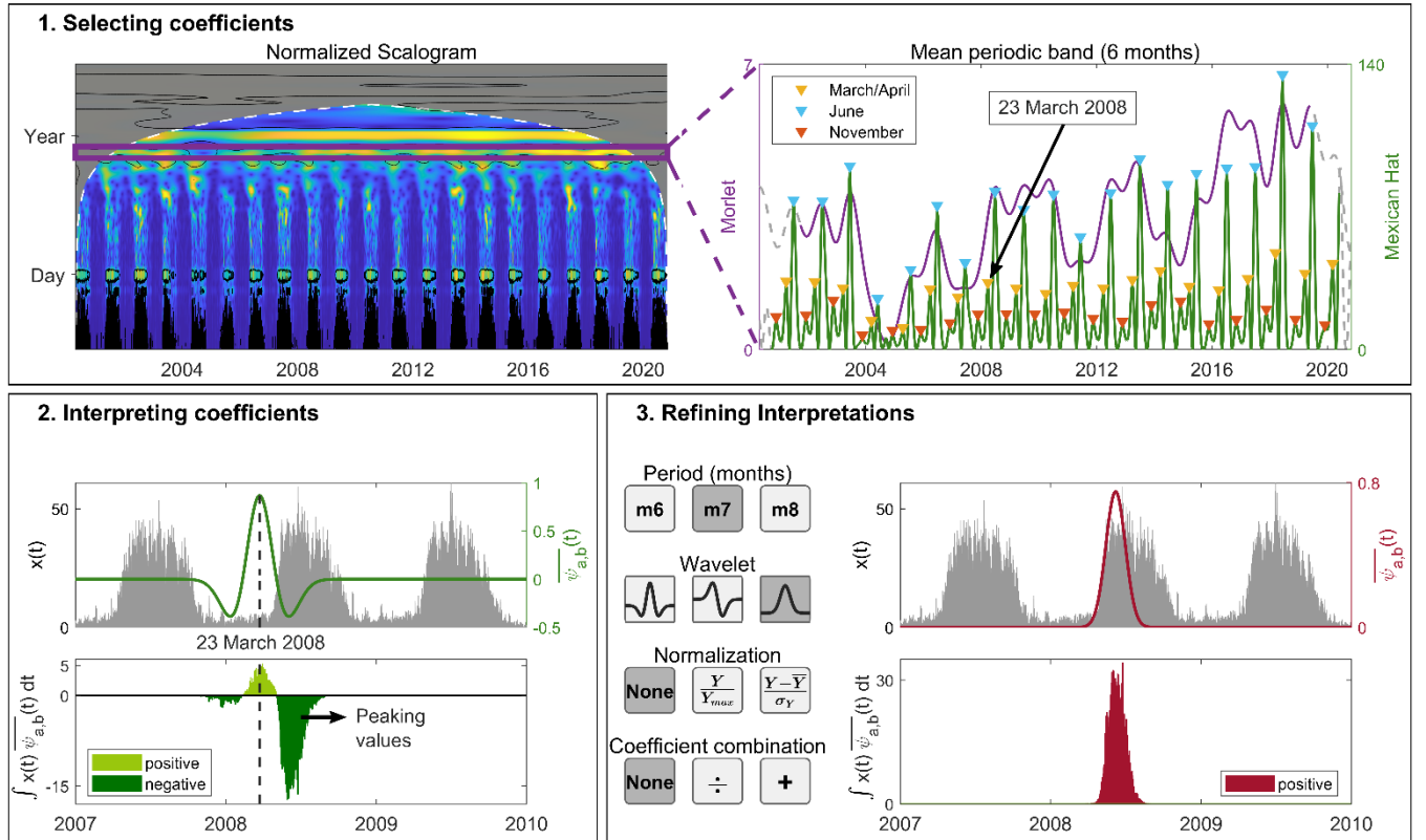
Figure 3: Schematic view of the 3-step workflow used to identify and interpret meaningful wavelet coefficients. Step 1 (selection): relevant coefficients are first identified by analyzing the temporal evolution of period-band amplitudes. Local maxima (peaks) in these signals indicate time windows where recurrent seasonal features are present. Step 2 (interpretation): selected coefficients are
