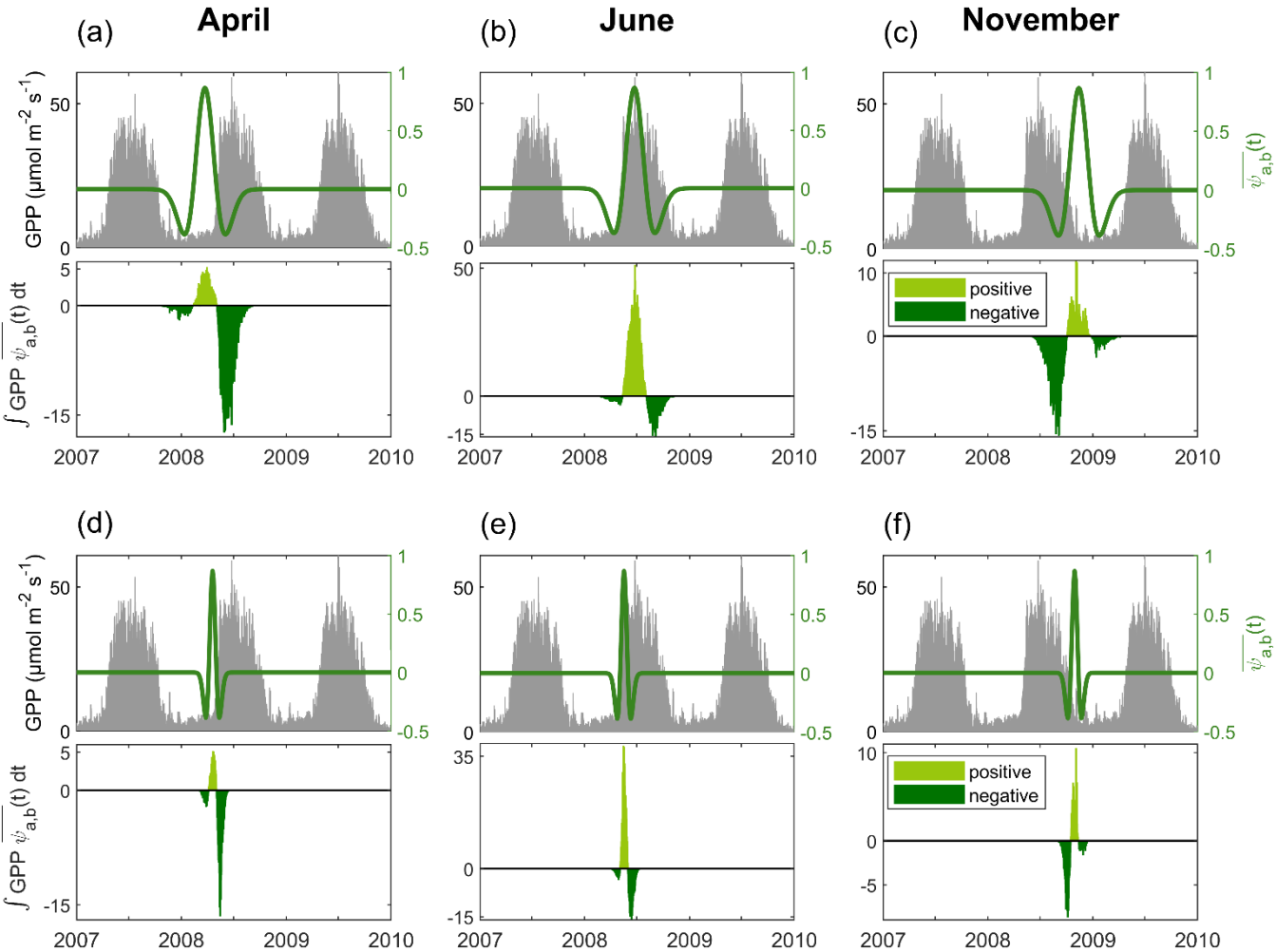
235 Figure 5: Computation steps for wavelet coefficients, (a-c) at a 6-month period for the three annual peaks observed with the Mexican Hat wavelet (see Fig. 4, zoom), and (d-f) at a 2-month period for their low-period counterpart.
