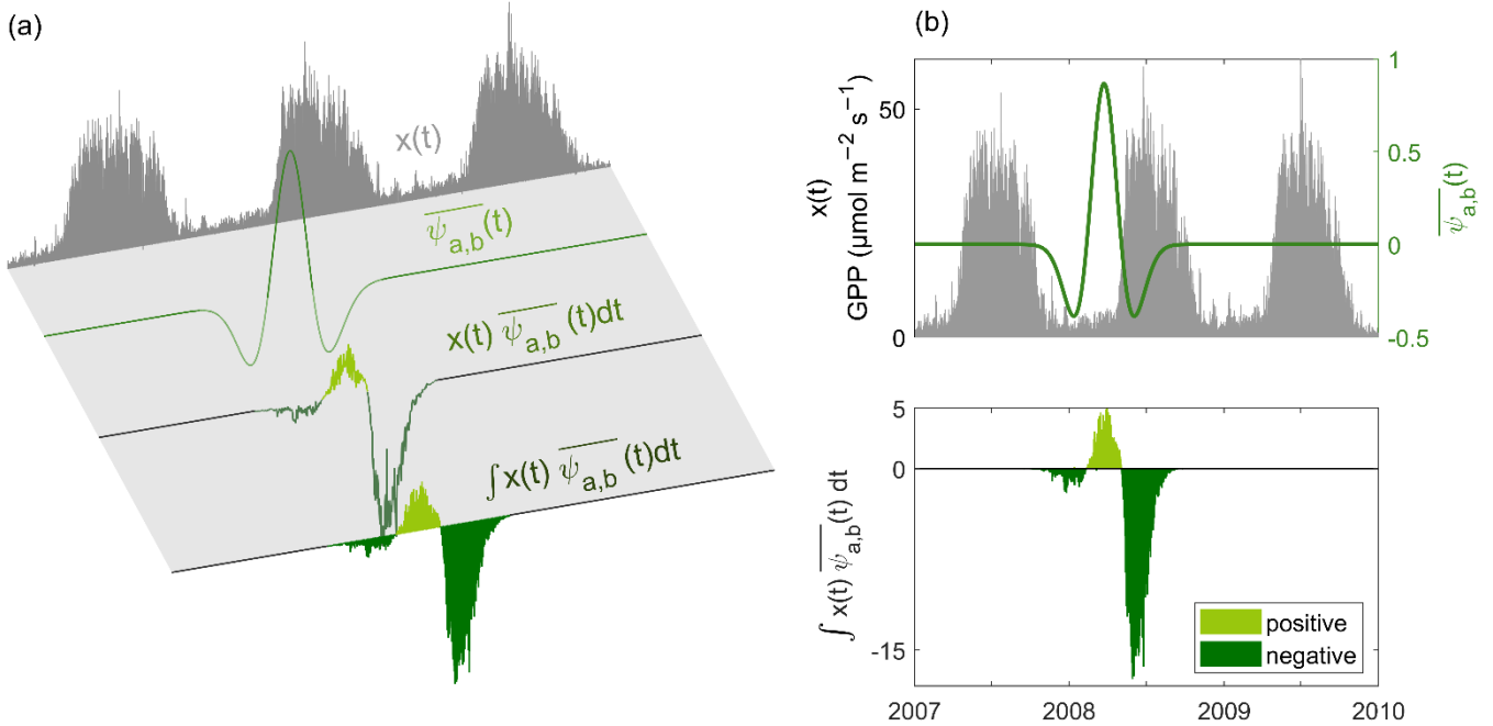
180 Figure 2: (a) Detailed computation of a wavelet coefficient following the mathematical definition of the CWT. (b) Condensed view of the computation process. The top graph displays the Mexican Hat wavelet at a chosen scale (corresponding to a 6-month period) and time (start of April) with the GPP signal in the background (restricted to positive values for readability). The graph below illustrates the area under the product curve of the wavelet and the signal. The algebraic sum of the three contributing areas, each linked to a lobe of the wavelet, corresponds to the wavelet coefficient yielded by the WT at the selected scale and time, after normalization.
