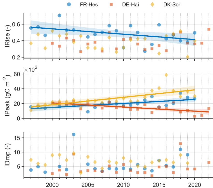
Figure 9: Temporal evolutions of the three indicators for the three forest sites (FR-Hes, DE-Hai, DK-Sor). Each panel corresponds to a different GPP indicator: initial slope (IRise, top), peaking values (IPeak, middle) and mid-season drop intensity (IDrop, bottom). Data points represent observed annual values for each indicator. When site-specific slopes were significant ( p \leq 0.05 ), linear trends (solid line) alongside 95 % confidence intervals (shaded areas) are displayed. Note that indicator units are not directly interpretable, as they reflect wavelet-derived features rather than absolute physical quantities.
