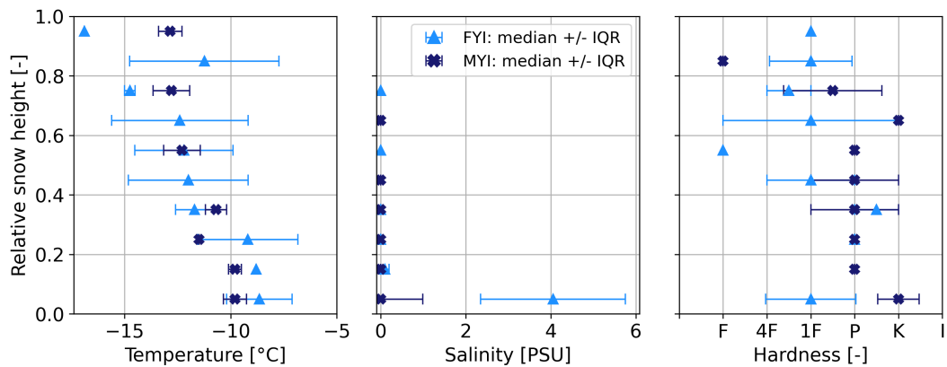
Figure 4. In situ snow properties averaged across all snow pits in 10% height intervals: temperature, salinity, and hardness. The hardness letter codes are: fist (F), 4 fingers (4F), 1 finger (1F), pencil (P), knife (K), ice (I) (Fierz et al., 2009). Profiles are shown in relative snow height, with 0 the bottom and 1 the top of the snow pit.
