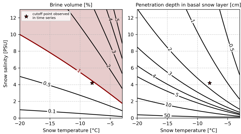
Figure 11. Modeled brine volume and Ku-band radar penetration depth into the basal snow layer (bottom 10% of snow pack) for a range of typical Arctic snow temperature and salinity values, assuming a snow density of 310 kg/m³ (the median snow density for the FYI study sites in mid-May). Red shading is applied where combinations of temperature and salinity lead to a brine volume exceeding 1%, which is empirically associated with high likelihood of biased radar freeboards. The cutoff point observed in the time series that led to this threshold is marked with a star.
