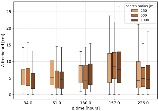
Figure A1. Absolute difference in laser freeboards for all intersections found when using the 100 km search distance for lead tie points, for three different search radii at five different time lags.
