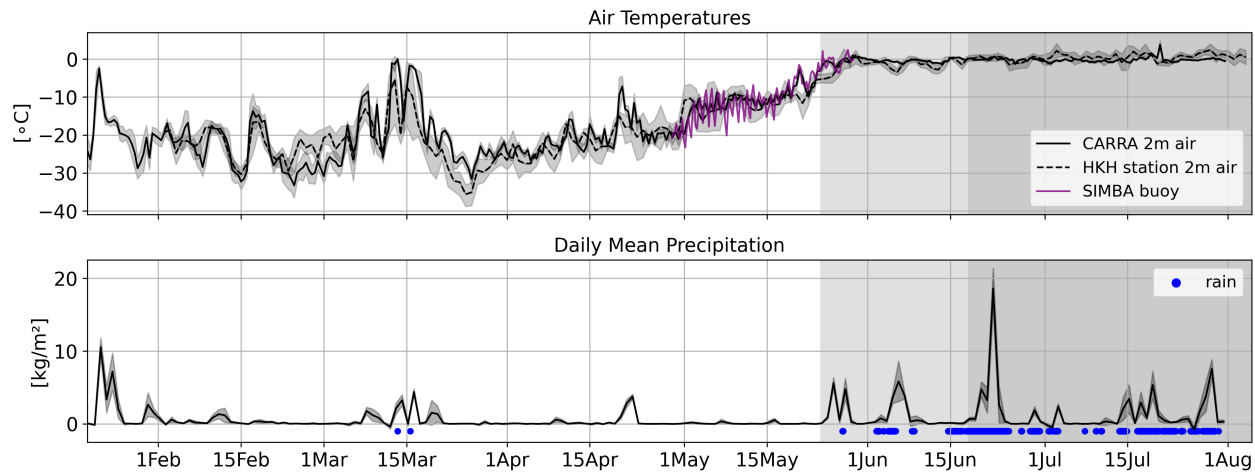
Figure 2. Air temperature and daily mean precipitation over the Øer Ice Barrier in Spring 2022. Air temperatures are shown for different data sources: CARRA reanalysis, Henrik Krøyer Holme (HKH) weather station, and SIMBA. Precipitation is only available from reanalysis (CARRA).
