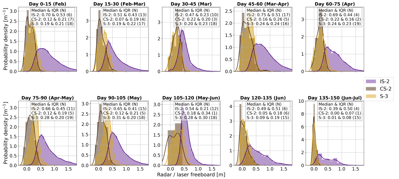
Figure 8. The evolution of laser and radar freeboard distributions at 15-day intervals for MYI. Note the scale difference on the x-axis compared to the FYI distributions in Fig. 87. Distributions are estimated using all along-track freeboards samples inside the ROIs, i.e. before any spatial averaging is performed. N stands for the number of tracks feeding into the distribution.
