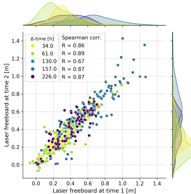
Figure 3. Comparison of mean laser freeboards for pairs of intersecting IS-2 beams, colour-coded color-coded by time lag. Spearman's correlation coefficient (R) is reported per time lag and kernel density estimated PDF's are shown on the sides.
