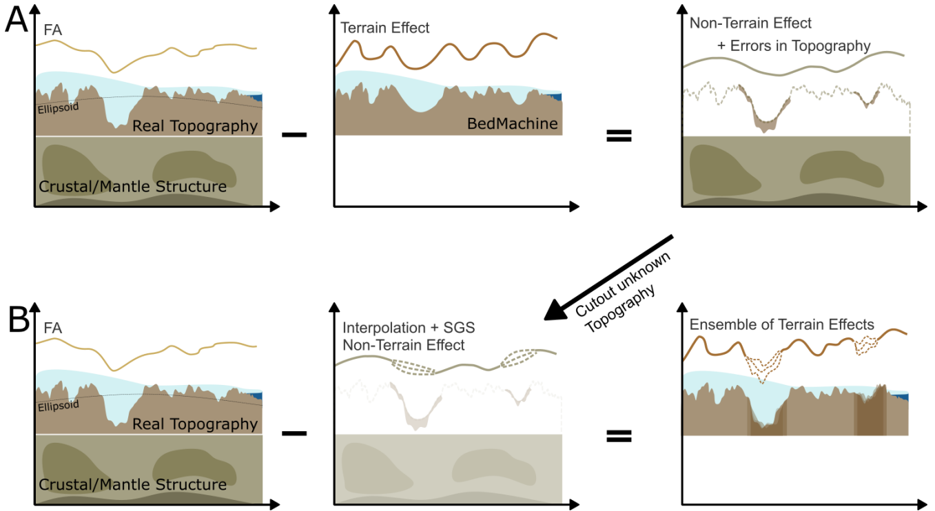
Figure 2. Schematic of the isolation process of non-terrain and terrain gravity effects and propagating uncertainties in subsurface geology. (A) Subtracting the terrain correction based on BedMachine from the Free-Air Anomaly (FA) yields a non-terrain effect field, but errors or biases in the prescribed topography map directly into the residual signal. (B) Instead of relying on a fixed bed, we interpolate and stochastically simulate (with SGS) the non-terrain component. Regions with unknown or poorly constrained topography are cut out and replaced with ensembles of plausible background gravity fields. Removing this from the FA, we obtain an ensemble of terrain effects, capturing the uncertainty arising from unknown regional background gravity effects. More details and step-by-step descriptions are in the text.
