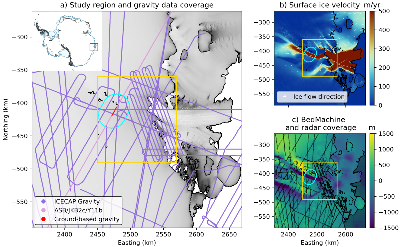
Figure 1. Overview of the Denman Glacier region. (a) Gravity survey coverage and outlines of target areas for regional (yellow rectangle) and local (light blue oval) inversion. (b) Surface velocity and flow directions from MEaSURES (Rignot et al., 2019b). (c) Bed topography from BedMachine v3 (Morlighem et al., 2020) with ICECAP RES bed pics and bathymetry in light gray including grounding line and ice shelf outlines. (d)
