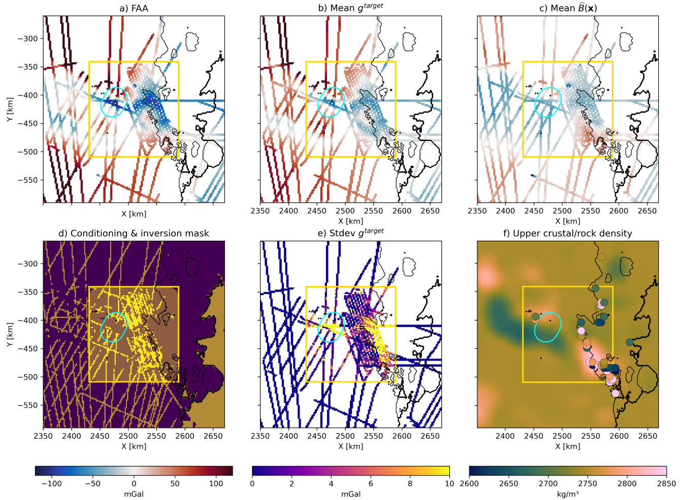
Figure 3. Overview of the input grids and masks used in the inversion. (a) Free-air anomaly (FAA); (b) mean trend-eliminated (TE) target; (c) mean Bouguer disturbance; (d) conditioning data (yellow lines/areas) in- and outside of inversion masks (regional: golden rectangle, local: cyan contour); (e) standard deviation of the TE target from sequential Gaussian simulation; and (f) spatially-variable rock-density field with 5 km binned sample locations (Löising et al., 2024). Inversion masks are shown for regional (golden rectangle) and local trough (cyan contour) inversions.
