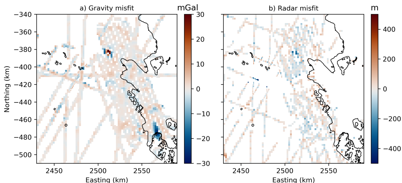
Figure 7. (a) Gravity misfit for the best-fitting realization (target - modeled). (b) Radar misfit for the best-fitting realization (target - modeled). Black contours indicate major geographic boundaries.
