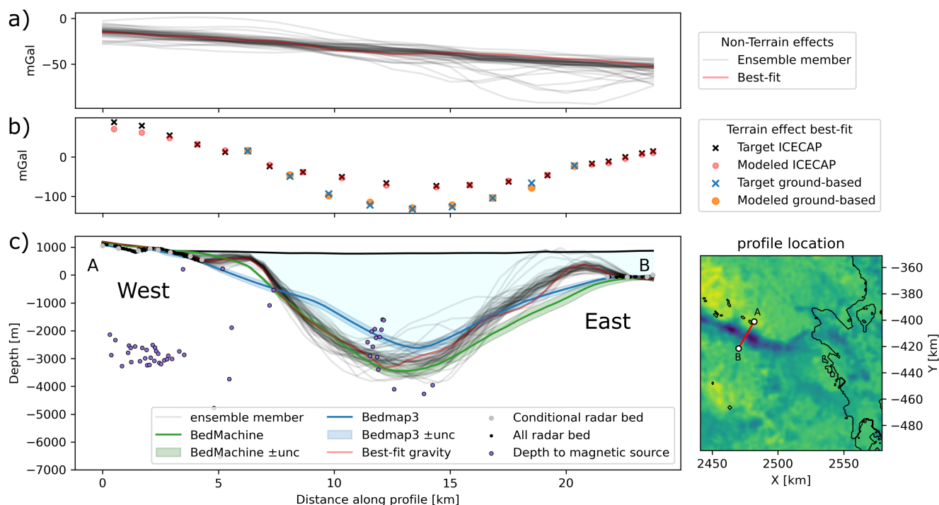
Figure 9. Along-transect cross-section A–B of the Denman Glacier trough. (a) Non-terrain gravity effects (mGal). (c) Comparison of bedrock interface estimates, showing radar-derived bed picks (black dots), conditional radar points (silver dots), ensemble results (grey lines), and the best-fit inverted bed (light red). For reference, Bedmap3 \pm uncertainty (blue ribbon), BedMachine \pm uncertainty (dark green ribbon), and DMS estimates (purple dots) are included alongside the ice surface (black).
