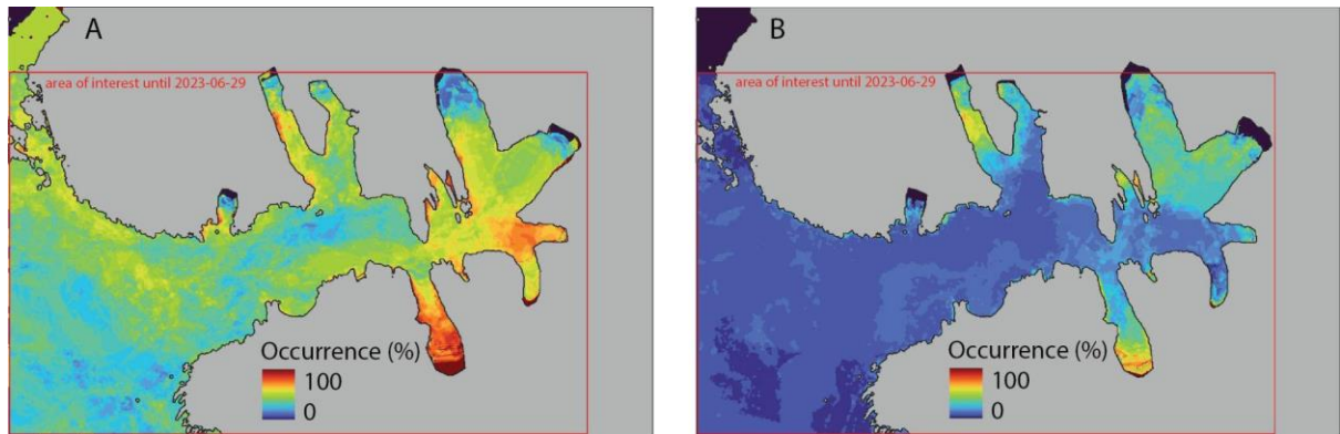
Figure 4. Mean distribution of ice on the (a) freeze-up and (b) break-up of the landfast ice in Hornsund over the 23 seasons from 2002–2025.
