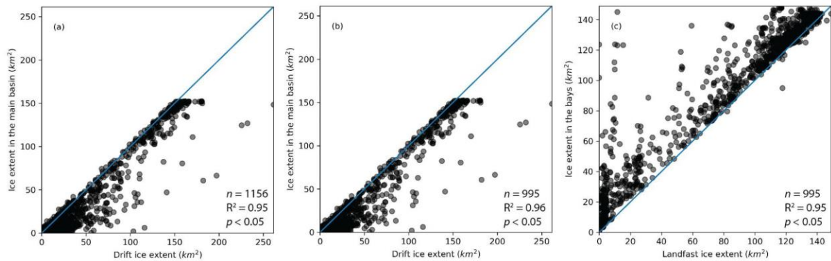
Figure 10. Spatial extent of the drift and landfast ice in Hornsund from Swirad et al. (2026b) and the ice extent in the main basin and the bays from our study on individual days between 2012-01-02 and 2023-06-29. Panel (a) represents the sea ice season and panels (b-c) – the landfast ice season.
