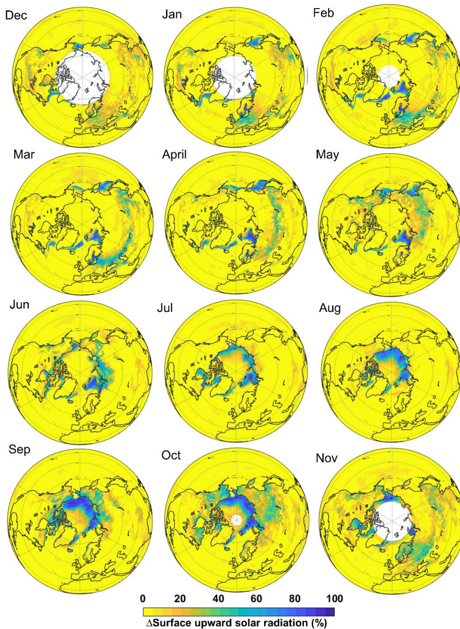
Figure 10. Changes in annual -ERA5 annual surface upward solar radiation (in percent) in the Northern hemisphere, obtained by comparing the rates of differences in mean values (in percent) of the periods 1979-2014-1988-2023 and 1979-2014-2023-1988 divided by mean values of the former period. No data are available during the polar night, denoted with white colour.
