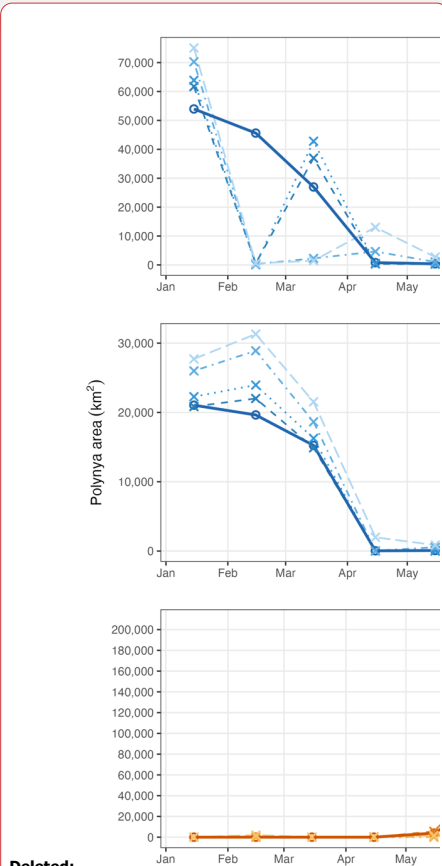
Figure 8: Polynya area estimates for the Amundsen Sea Polynya and Pine Island Polynya in 2020 and the Weddell Sea in 2017, derived using the geomorphon algorithm and four sea ice concentration thresholds ( \leq 0.2 , \leq 0.3 , \leq 0.6 and \leq 0.8 ). Symbols represent individual daily estimates calculated from the sea ice concentration field on the 15th day of each month and are not monthly mean values. Lines connect corresponding estimates only to aid visual tracking of each method through the annual cycle. Expanded April–October panels are shown for the Amundsen Sea polynyas to highlight the smaller winter area estimates. Colours distinguish study regions and threshold values, while symbols and line types distinguish the geomorphon and threshold-based approaches.
