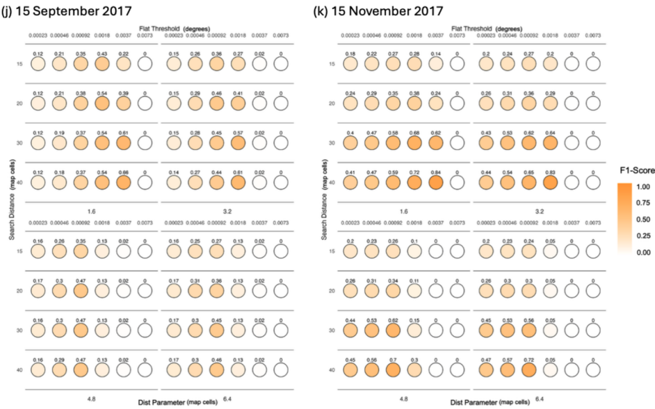
Figure D8: Seasonal performance of all valid geomorphon parameter combinations during austral spring (September–November) for the Weddell Sea (2017), evaluated using daily sea ice concentration fields from the 15th day of each month. Bubble colour indicates the F1-score for months containing one or more reference polynya pixels and the False Positive Rate (FPR) for months in which no reference polynya pixels were present. Bubble size is proportional to the corresponding performance metric. Parameter combinations are arranged according to the search parameter (map cells), flat threshold (degrees), and dist parameter (map cells). The representative parameter tuning case study, 15 October 2017 for the Weddell Sea, is presented separately in Figure 4.
