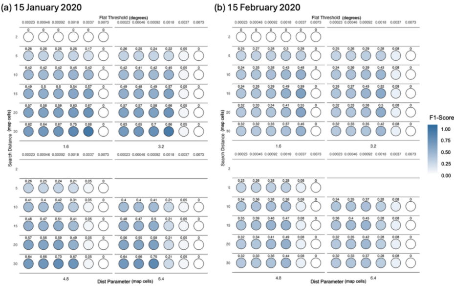
1110 Figure D1: Seasonal performance of all valid geomorphon parameter combinations during austral summer (December-February) for the Amundsen Sea (2020), evaluated using daily sea ice concentration fields from the 15th day of each month. Bubble colour indicates the F1-score for months containing one or more reference polynya pixels and the False Positive Rate (FPR) for months in which no reference polynya pixels were present. Bubble size is proportional to the corresponding performance metric. Parameter combinations are arranged according to the search parameter (map cells), flat threshold (degrees), and dist parameter (map cells). The representative parameter tuning case study, 15 December 2020 for the Amundsen Sea, is presented separately in Figure 5.
