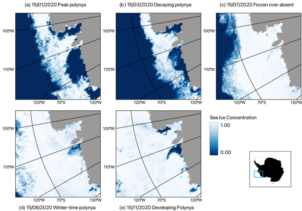
1035 Figure A1: Representative sea ice concentration fields for the five Amundsen Sea 2020 scenarios. Daily data was obtained from the University of Bremen Archive, AMSR2 ASI sea ice concentration, version 5.4 (Melsheimer and Spreen, 2019).
