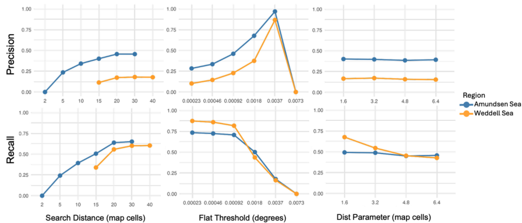
Figure C2: Precision (top row) and recall (bottom row) scores for different parameter values ( search , flat , dist ) used in iterations of the geomorphon algorithm in the Amundsen (blue) and Weddell (orange) Seas. Precision and recall scores are calculated as averages for each parameter value, considering its combination with all values from the other two parameters in each iteration.
