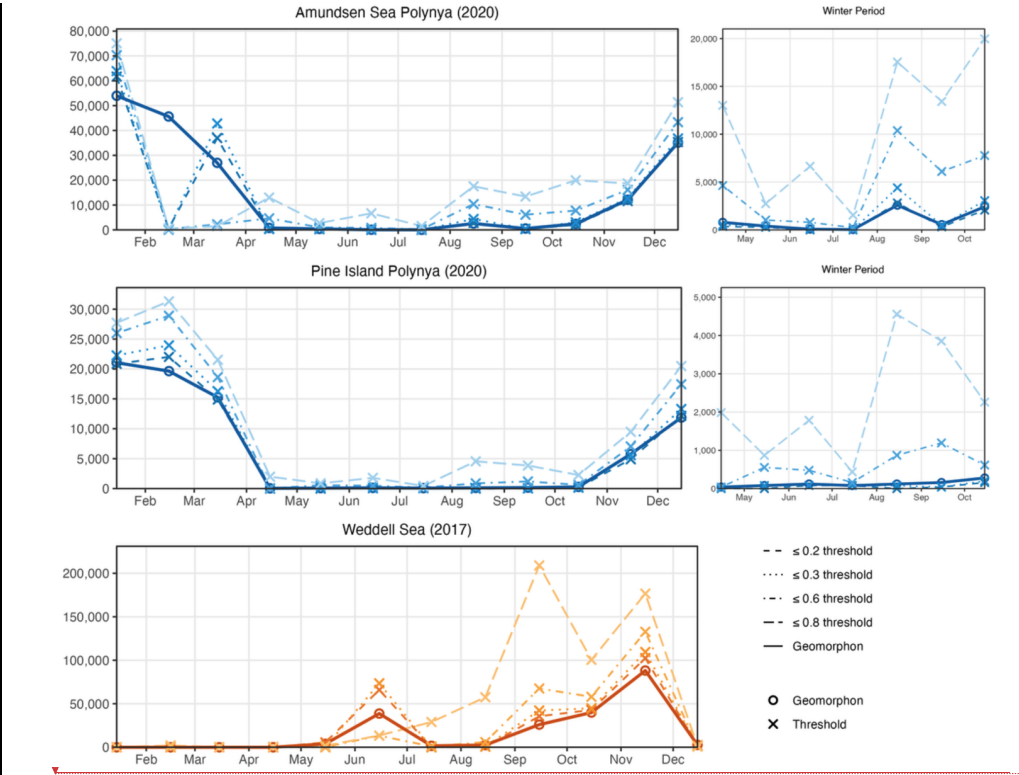
Figure 8: Polynya area estimates for the Amundsen Sea Polynya and Pine Island Polynya in 2020 and the Weddell Sea in 2017, derived using the geomorphon algorithm and four sea ice concentration thresholds ( \leq 0.2 , \leq 0.3 , \leq 0.6 and \leq 0.8 ). Symbols represent individual daily estimates calculated from the sea ice concentration field on the 15th day of each month and are not monthly mean values. Lines connect corresponding estimates only to aid visual tracking of each method through the annual cycle. Expanded April–October panels are shown for the Amundsen Sea polynyas to highlight the smaller winter area estimates. Colours distinguish study regions and threshold values, while symbols and line types distinguish the geomorphon and threshold-based approaches.
