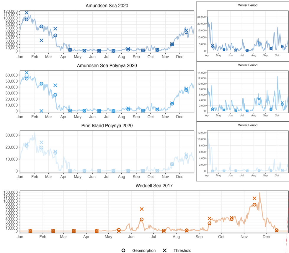
Figure 7: Polynya area estimates for the whole Amundsen Sea, Amundsen Sea Polynya, and Pine Island Polynya (2020) and Weddell Sea (2017). Pale solid lines show the complete daily geomorphon-derived polynya area time series using the final parameter combinations (Amundsen Sea: flat = 0.0037°, search = 30 map cells, dist = 1.6 map cells; Weddell Sea: flat = 0.0037°, search = 40 map cells, dist = 1.6 map cells). Open circles indicate the geomorphon-derived polynya area for the daily sea ice concentration field corresponding to the 15th day of each month used in the seasonal consistency assessment; these symbols represent individual daily estimates rather than monthly mean values. Crosses indicate the corresponding daily polynya area estimates derived using the \leq 0.3 sea ice concentration threshold method for the same dates. Insets show the April-October period using an expanded y-axis to highlight the smaller winter polynya areas in the Amundsen Sea.
