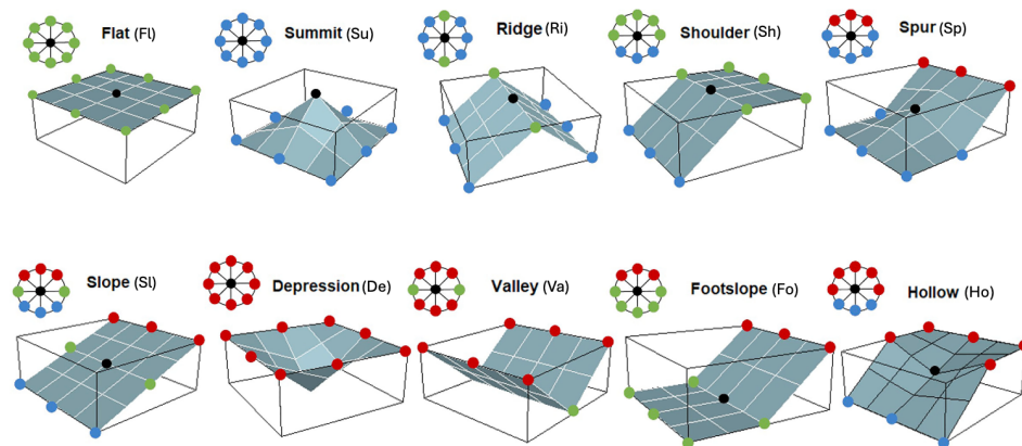
420 Figure 2: Symbolic 3D morphologies and their coordinating geomorphons (ternary patterns) for the 10 most common landform elements (adapted from Jasiewicz and Stepinski, 2013 and Wyles et al., 2022). Coloured points demonstrate if the cells surrounding the central cell (black) are lower (blue), higher (red), or the same elevation (green) as the central cell.
