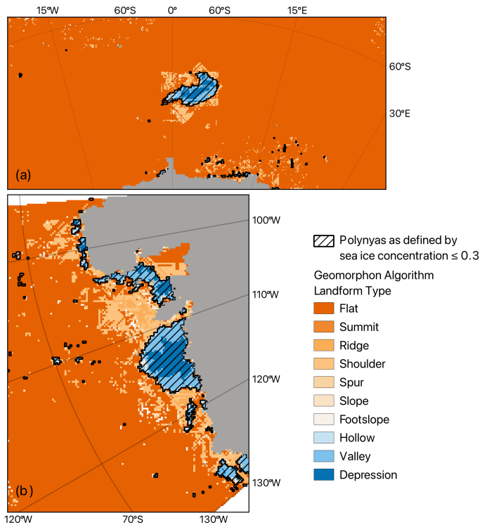
Figure 6: Geomorphon landform classifications for the representative parameter tuning case studies in the (a) Weddell Sea (15 October 2017) and (b) Amundsen Sea (15 December 2020). The Weddell Sea classification was generated using the best-performing 655 parameter combination for that region ( flat = 0.0037^\circ , search = 40 map cells, dist = 1.6 map cells), while the Amundsen Sea classification used flat = 0.0037^\circ , search = 30 map cells, and dist = 1.6 map cells. Areas identified as polynyas using the sea ice concentration threshold ( \leq 0.3 ) are outlined in black hatching. Geomorphon landforms associated with polynya detection (hollow, depression and valley) are shown in shades of blue, whereas the remaining landform classes are shown in shades of orange.
