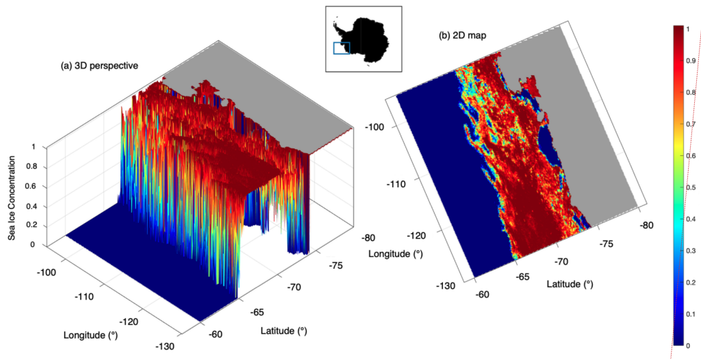
Figure 3: Example of daily sea ice concentration for the Amundsen Sea, 15 th December 2020 (same as shown in Fig. 1b). (a) Shows the three-dimensional perspective view of sea ice concentration, with (b) representing the two-dimensional map view of the same data. The dark blue steep declines in sea ice concentration seen near the coastline in (a) represent areas of coastal polynyas. Daily data was obtained from the University of Bremen Archive, AMSR2 ASI sea ice concentration, version 5.4 (Melsheimer and Spreen, 2019).
