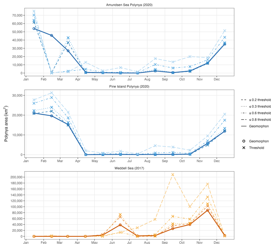
Figure 8: Monthly polynya area estimated using the geomorphon algorithm (solid lines, circles) and four sea ice concentration threshold-based methods ( \leq 0.2 , \leq 0.3 , \leq 0.6 and \leq 0.8 ; dashed lines, crosses) for the (a) Amundsen Sea Polynya 2020, (b) Pine Island Polynya 2020, and (c) Weddell Sea during 2017, respectively. The figure illustrates how estimated polynya extent varies with the choice of sea ice concentration threshold relative to the morphology-based geomorphon approach.
