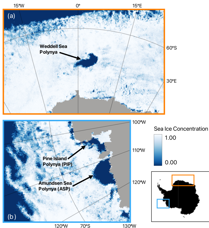
Figure 1: Daily sea ice concentration for the (a) Weddell Sea, 15 th October 2017, and (b) Amundsen Sea, 15 th December 2020. Insert shows the location of the Weddell Sea (orange) and Amundsen Sea (blue) on a larger scale. The Weddell Sea Polynya is labelled in (a), while the Amundsen Sea Polynya (ASP) and Pine Island Polynya (PIP) are labelled in (b). Daily data was obtained from the University of Bremen Archive, AMSR2 ASI sea ice concentration, version 5.4 (Melsheimer and Spreen, 2019).
