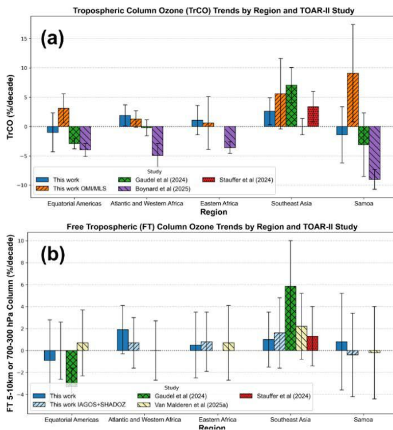
FIG 16 in Thompson, Stauffer et al. https://acp.copernicus.org/articles/25/18475/2025/
