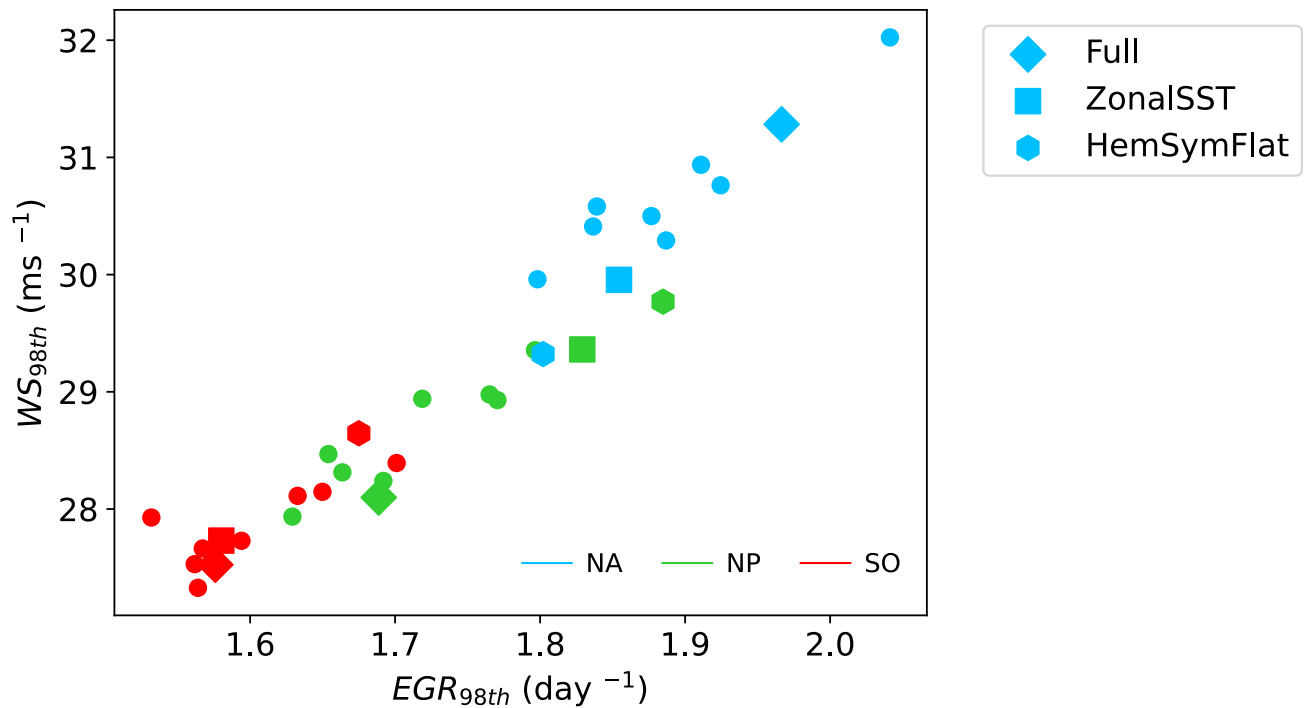
Figure 7. Scatterplot of winter basin-wide 98th percentiles of near-surface wind speed (y-axis) versus winter basin-wide 98th percentiles of mid-tropospheric Eady growth rates (x-axis) across 11 different ISCA experiments with varying boundary conditions. Different colors represent different basins (same colors as in Fig. 1c, 5, 6a), while shapes different than simple dots represent experiments chosen for the analysis. ERA5 values are shown in Fig. S3.
