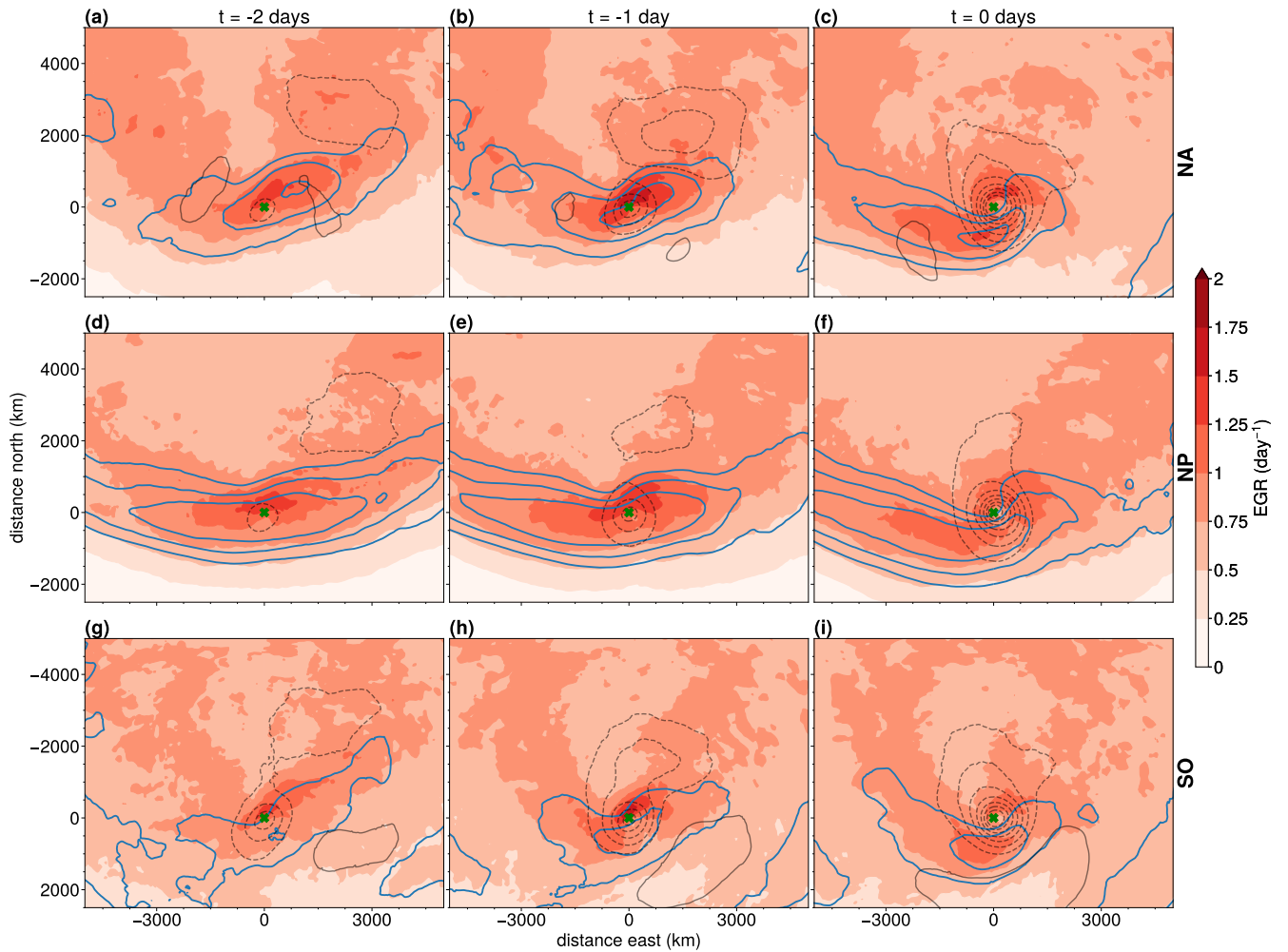
Figure 4. Composites of mid-tropospheric EGRs for top 100 extremes in the NA (a-c), NP (d-f) and SO (g-i) centered on the cyclone locations from t = -2 days to t = 0 days. Green crosses have the same meaning as in Figures 2, 3. Dark blue contours show the values of 250 hPa wind speeds, starting from 35 \text{ ms}^{-1} and increasing in steps of 10 \text{ ms}^{-1} . Black contours show MSLP anomalies relative to the 1979-2020 climatology, every \pm 5 \text{ hPa} and starting from \pm 5 \text{ hPa} (dashed for negative anomalies).
