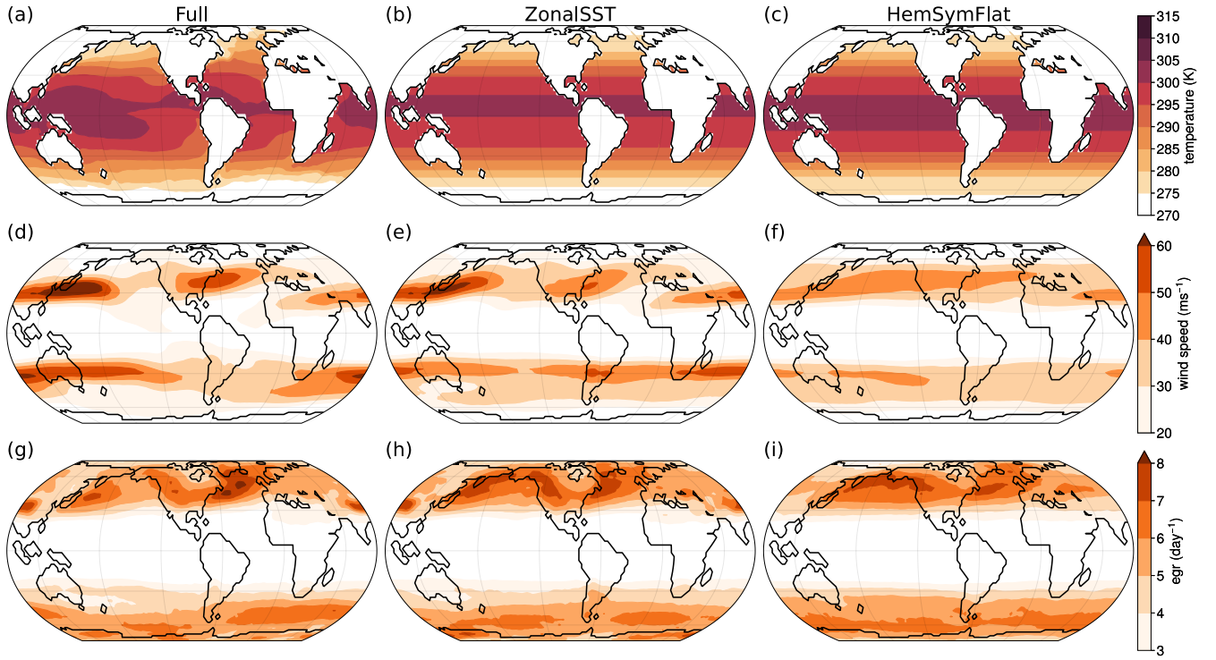
Figure 8. Climatologies of SSTs (a-c), medians of wind speed between 200 and 300 hPa (d-f) and EGR (g-i) during respective winter seasons across ISCA experiments. (a), (d), (g) show the results from Full, (b), (e), (h) ZonalSST and (c), (f), (i) HemSymFlat experiments.
