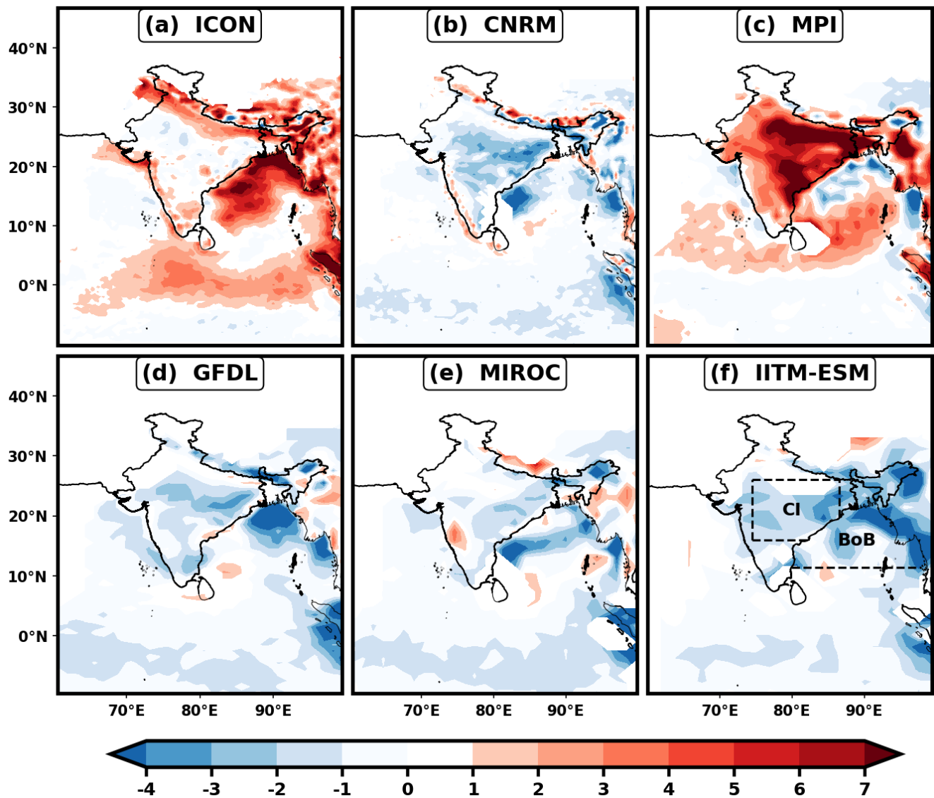
Figure 2. Spatial distribution of JJAS climatological mean diurnal precipitation amplitude bias ( mm day -1 ) relative to IMERG for (a-f) ICON, CNRM, MPI, GFDL, MIROC and IITM-ESM. The two representative regions Central India (CI), and the Bay of Bengal (BoB) used for regional bias analysis (Table 2) are indicated in panel (f). The boxes are bounded by land boundaries and dashed outlines such that CI excludes oceanic grid points and BoB excludes land grid points.
