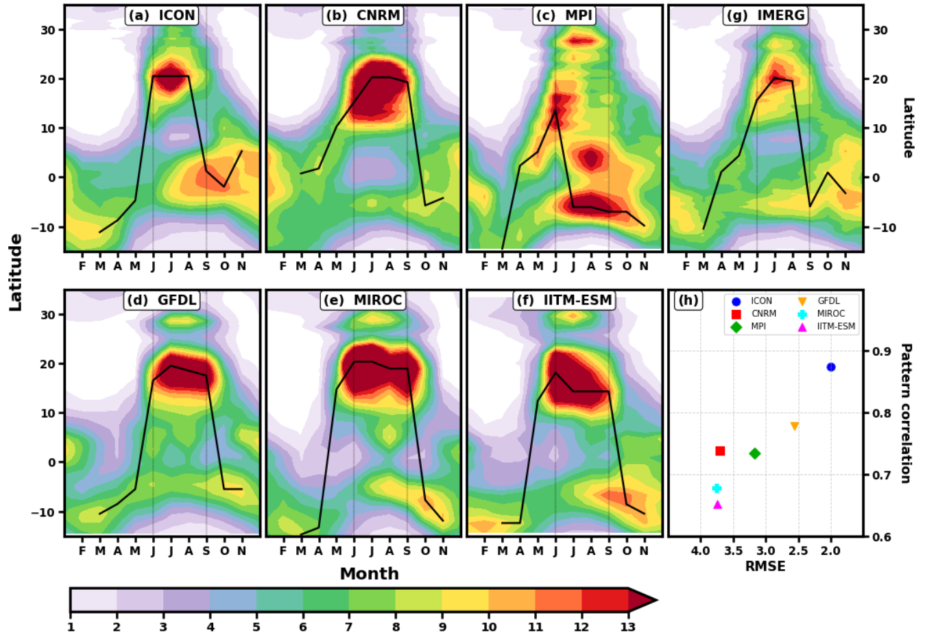
Figure 12. Latitude–time evolution of the climatological mean annual cycle of precipitation ( \text{mm day}^{-1} ) averaged zonally over the Indian monsoon region ( 70^{\circ} – 90^{\circ}\text{E} ) from (a–f) ICON, CNRM, MPI, GFDL, MIROC, and IITM-ESM model simulations, with (g) IMERG as observational reference. The overlaid black curve denotes the latitude of maximum precipitation, illustrating the seasonal migration of the monsoon rainband. The faint black dotted lines mark the monsoon season (JJAS). Panel (h) presents the scatter of pattern correlation coefficient (PCC) versus root-mean-square error (RMSE) for all models relative to IMERG.
