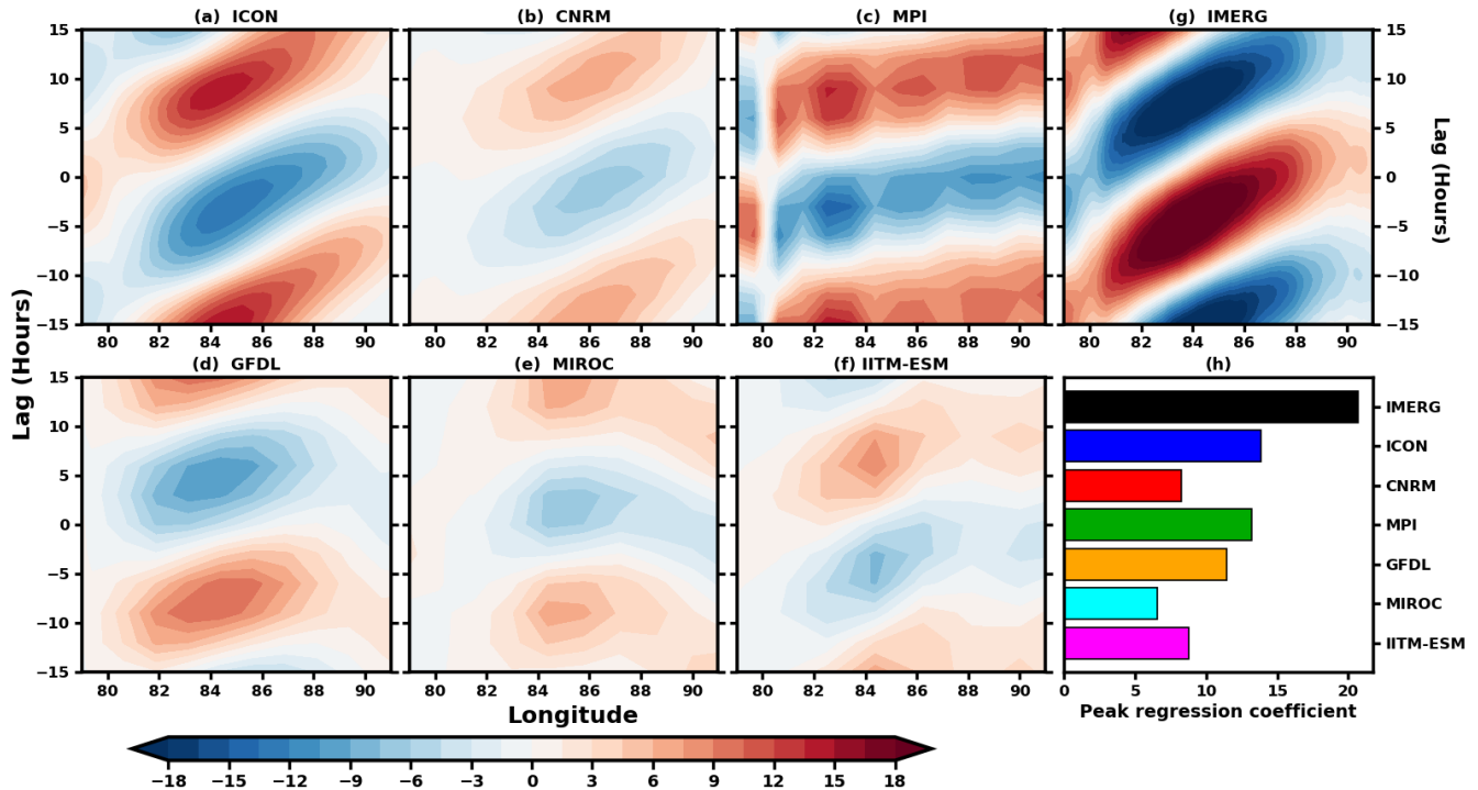
Figure 7. Eastward propagation of diurnal convective systems inferred from lead-lag regression (-15 to +15 h) between EOF2 principal component (PC2) and diurnal rainfall anomalies averaged over 8^{\circ} – 16^{\circ} N. Results are shown for (a–f) ICON, CNRM, MPI, GFDL, MIROC, and IITM-ESM, with (g) IMERG as the observational reference. Panel (h) summarizes the peak regression coefficients for IMERG and all models.
