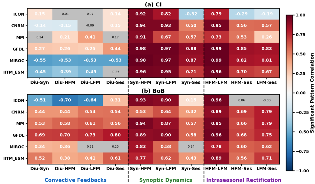
Figure 15. Heatmap of spatial pattern correlation coefficients among the relative bias fields of different scales. Correlations significant at the 95% confidence level are highlighted in bold white font, while non-significant cells are masked in gray (small black font). For clarity, the heatmap is divided into three scale-dependent regimes: convective, synoptic, and intraseasonal. The abbreviations Diu, Sys, HFM, LFM, and Ses represent the diurnal, synoptic, high-frequency MISO (10–20 days), low-frequency MISO (20–100 days), and seasonal scales, respectively.
