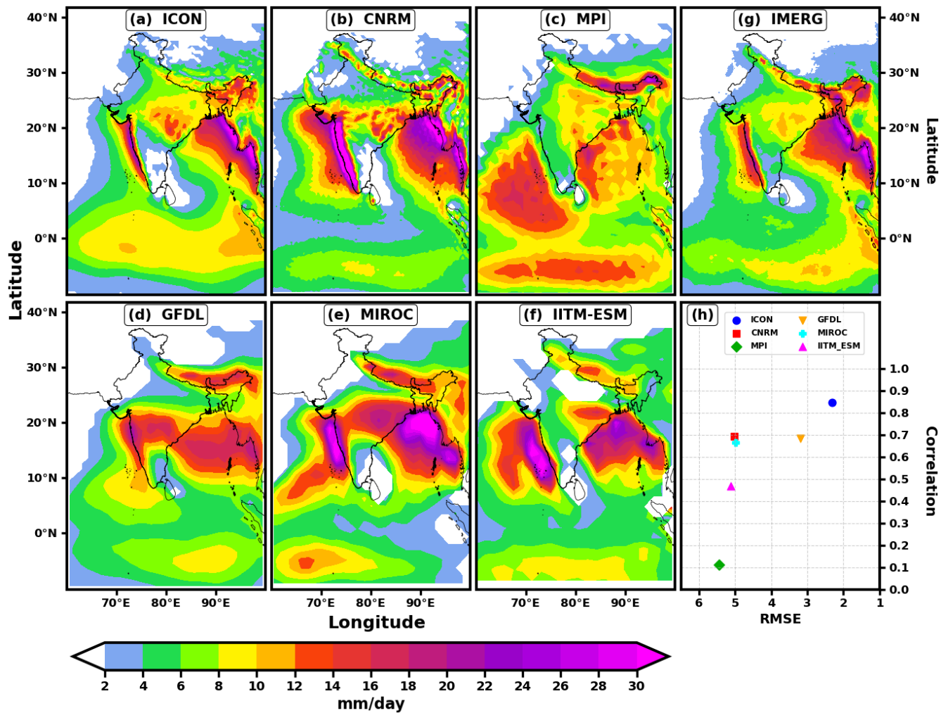
Figure 11. Seasonal (JJAS) averaged climatological mean rainfall (in \text{mm day}^{-1} ) from (a) ICON, all the participant CMIP6 (b-f: CNRM, MPI, GFDL, MIROC, and IITM-ESM) model simulations, and IMERG (g) as observational reference. Panel (h) shows the scatter between pattern correlation and RMSE.
