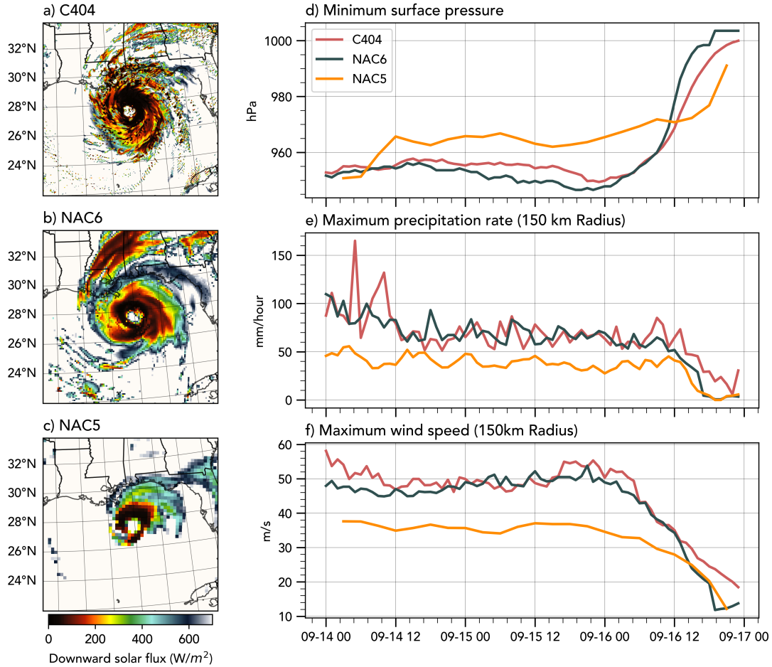
Figure 12. Shortwave radiation flux revealing cloud structure of the simulated TC on 2004-09-15 at 18:00 UTC in all three simulations (a-c). The right column shows the minimum surface pressure (d), maximum precipitation rate (e), and maximum wind speeds (f) within 150-km radius of the minimum surface pressure value.
