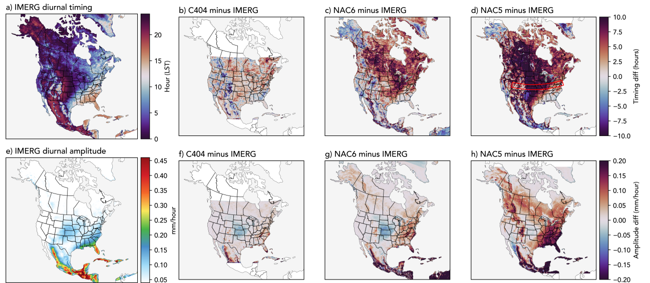
Figure 5. Diurnal precipitation peak time (top row) and magnitude (bottom row) for IMERG (a,e), C404 (b,f), NAC6 (c,g) and NAC5 (d,h) estimated using a second order harmonic fit of hourly precipitation for June, July and August. The domain for the longitude and time Hovmöller diagrams in the next figure is shown in panel (d)
