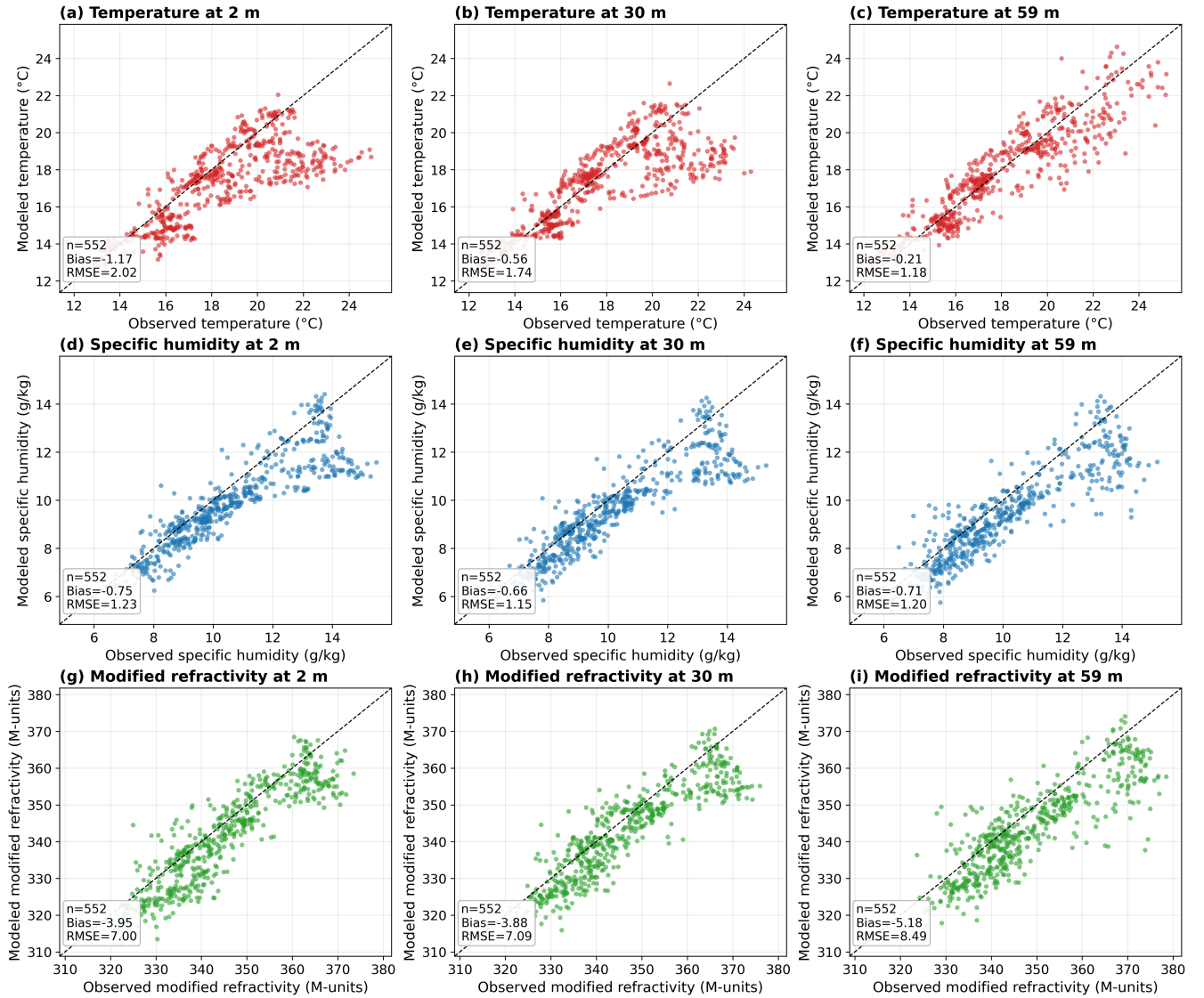
Figure 5. Scatterplots of modeled versus observed near-surface atmospheric variables at Utö for experiment EXP = 2500L65. Panels (a–c) show temperature ( T , red °C), panels (d–f) specific humidity ( q , blue g/kg), and panels (g–i) modified refractivity ( M , green M-units), each evaluated at 2 m, 30 m, and 59 m above ground level. Model-In all panels, observations are on the x-axis and model values (on the y-axis). The dashed line represents the theoretical perfect forecast. For each panel: sample size ( n ) are plotted against observations, mean bias ( x -axis model - observation), and RMSE are presented.
