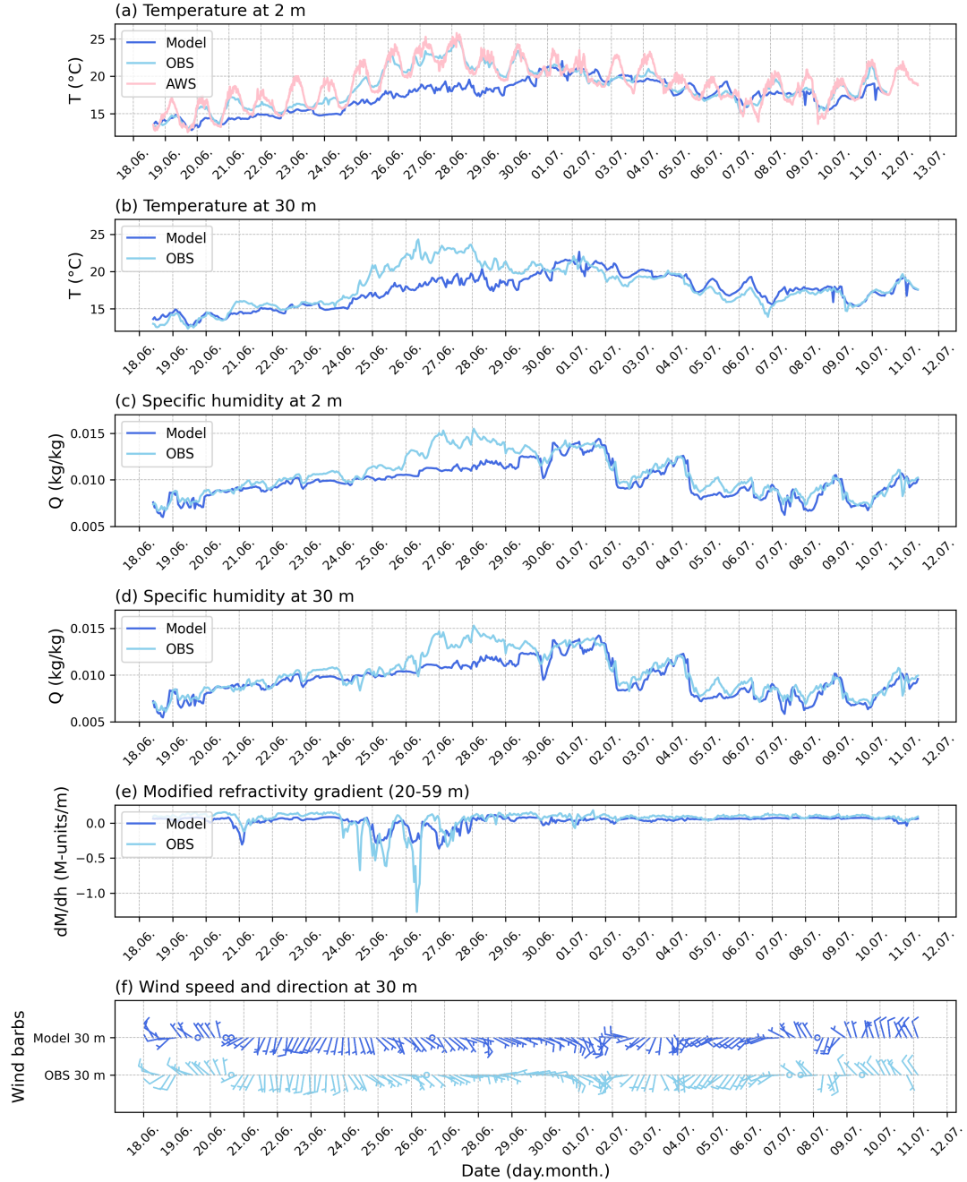
Figure 4. Time series of temperature (T), specific humidity (Q), modified refractivity gradient (dM/dh), and wind speed (WS) and direction (WD) at 2 m and 30 m at the Utö mast location. Dark blue curves show indicate model results from the operational model configuration, while light blue curves show observations from the Utö mast observations. In panel (a), and the pink curve in the top panel represents 2 m temperature from the nearest Automatic Weather Station (AWS), located further farther inland on Utö Island.
