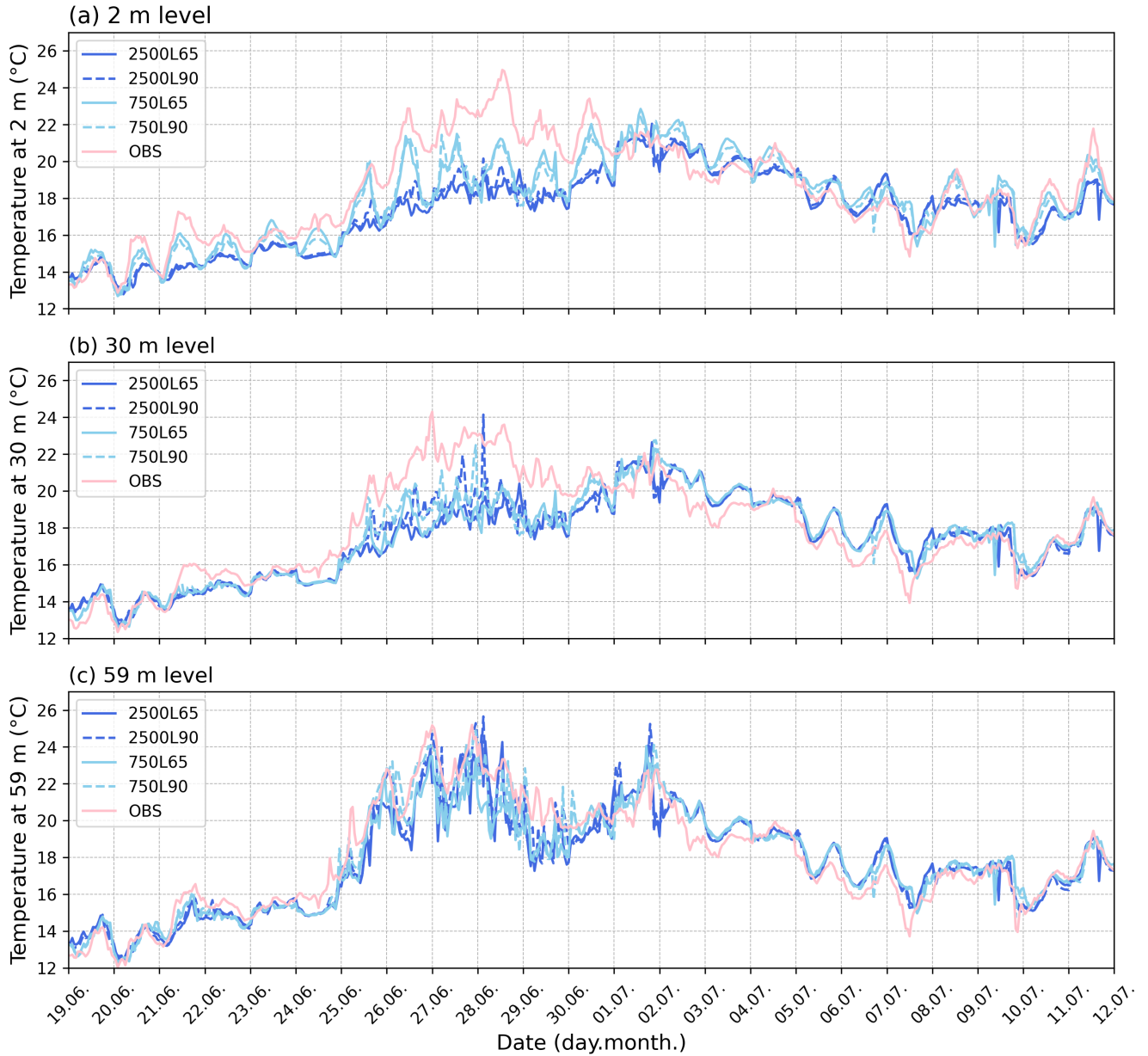
Figure 6. Time series of air temperature at Utö mast location at three levels heights: (a) 2 m (top), 30 m (middle), and 59 m (bottom) 59 m. Colors indicate Model results are shown for two horizontal resolutions of, 2500 m (dark blue) and 750 m (light blue), and are compared with observations in (pink). Vertical resolutions are shown resolution is indicated by line style: solid lines (denote 65 model levels) and dashed lines (denote 90 model levels).
