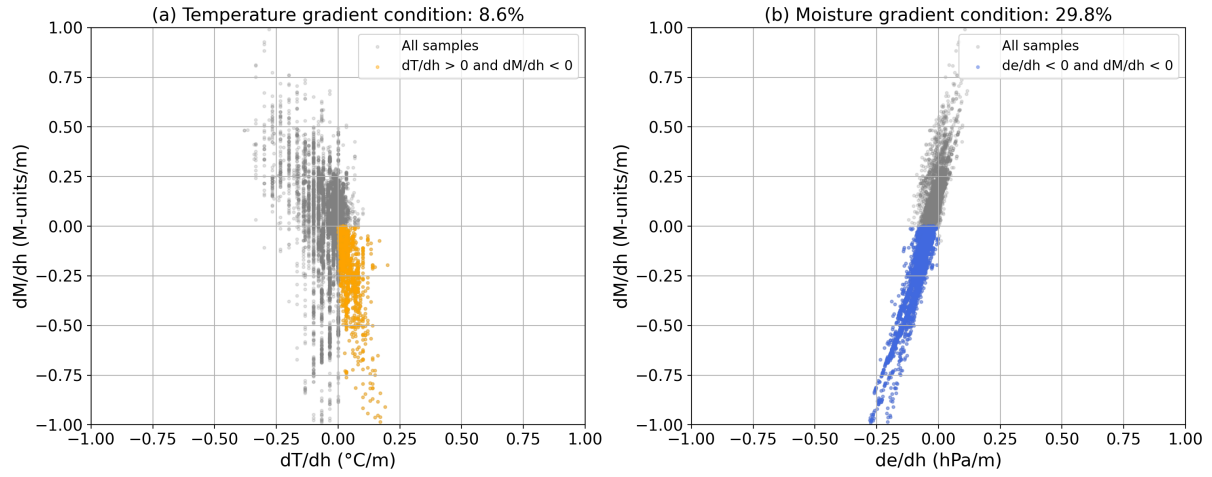
Figure 2. Scatter plots of observed vertical gradients of temperature ( dT/dh ; orange) and water vapor pressure ( de/dh ; blue) gradients versus against the modified refractivity gradient ( dM/dh ; gray) at different vertical across all analyzed levels between 2m to 60m. Orange and blue points highlight cases satisfying the ducting-related conditions dT/dh > 0 and dM/dh < 0 , based on observations and de/dh < 0 and dM/dh < 0 , respectively. The proportion of such cases are given is shown in the title each panel title.
