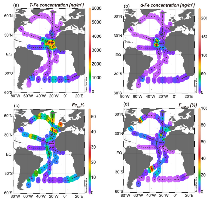
Figure 9. Spatial distributions of (a) T-Fe concentration, (b) d-Fe concentration, (c) Fe_{sol}\% , and (d) F_{anthro} in the Atlantic aerosols.
