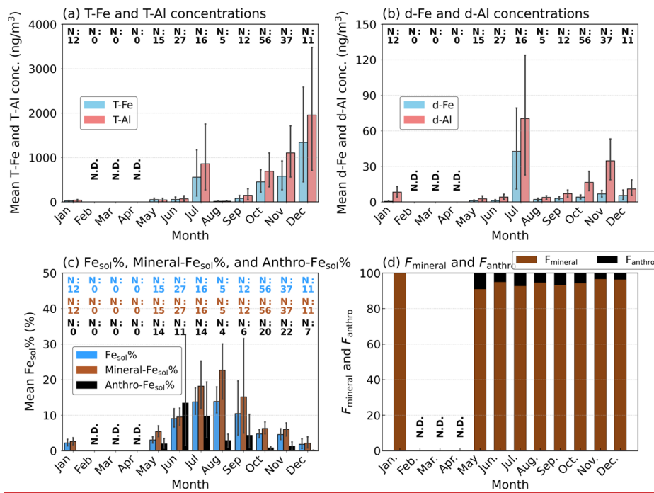
Figure 10. Monthly variations of (a) T-Fe and T-Al concentrations, (b) d-Fe and d-Al concentrations, (c) Fe sol %, mineral-Fe sol %, and anthro-Fe sol %, and (d) F_{\text{mineral}} and F_{\text{anthro}} in the Atlantic aerosols.
