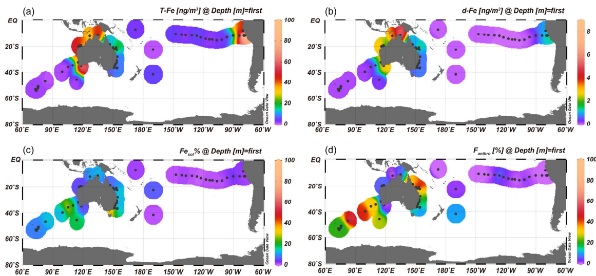
Figure 12. Spatial distribution of (a) T-Fe concentration, (b) d-Fe concentration, (c) Fe_{sol}\% , and (d) F_{anthro-dFe} in the South Pacific aerosols. (e) inverse relationship between Fe concentration and its Fe_{sol}\% .
