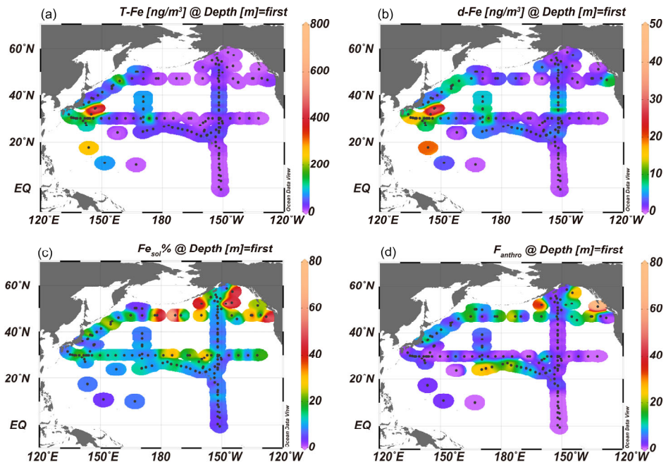
450 Figure 6. Spatial distributions of (a) T-Fe concentration, (b) d-Fe concentration, (c) Fe_{sol}\% , and (d) F_{anthro} in the North Pacific TSP samples.
