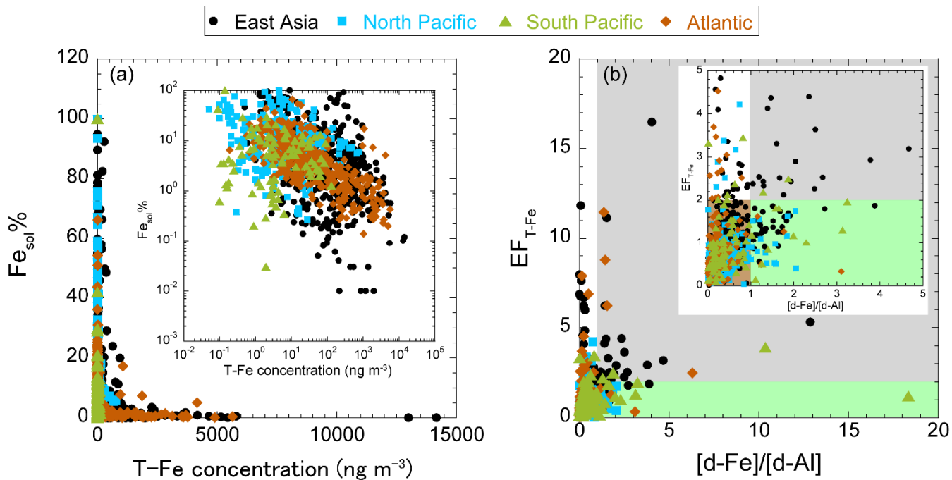
230 Figure 2. (a) Inverse plot of T-Fe concentration with Fe sol % and (b) [d-Fe]/[d-Al]-EF T-Fe diagram in aerosol samples compiled by this study.
