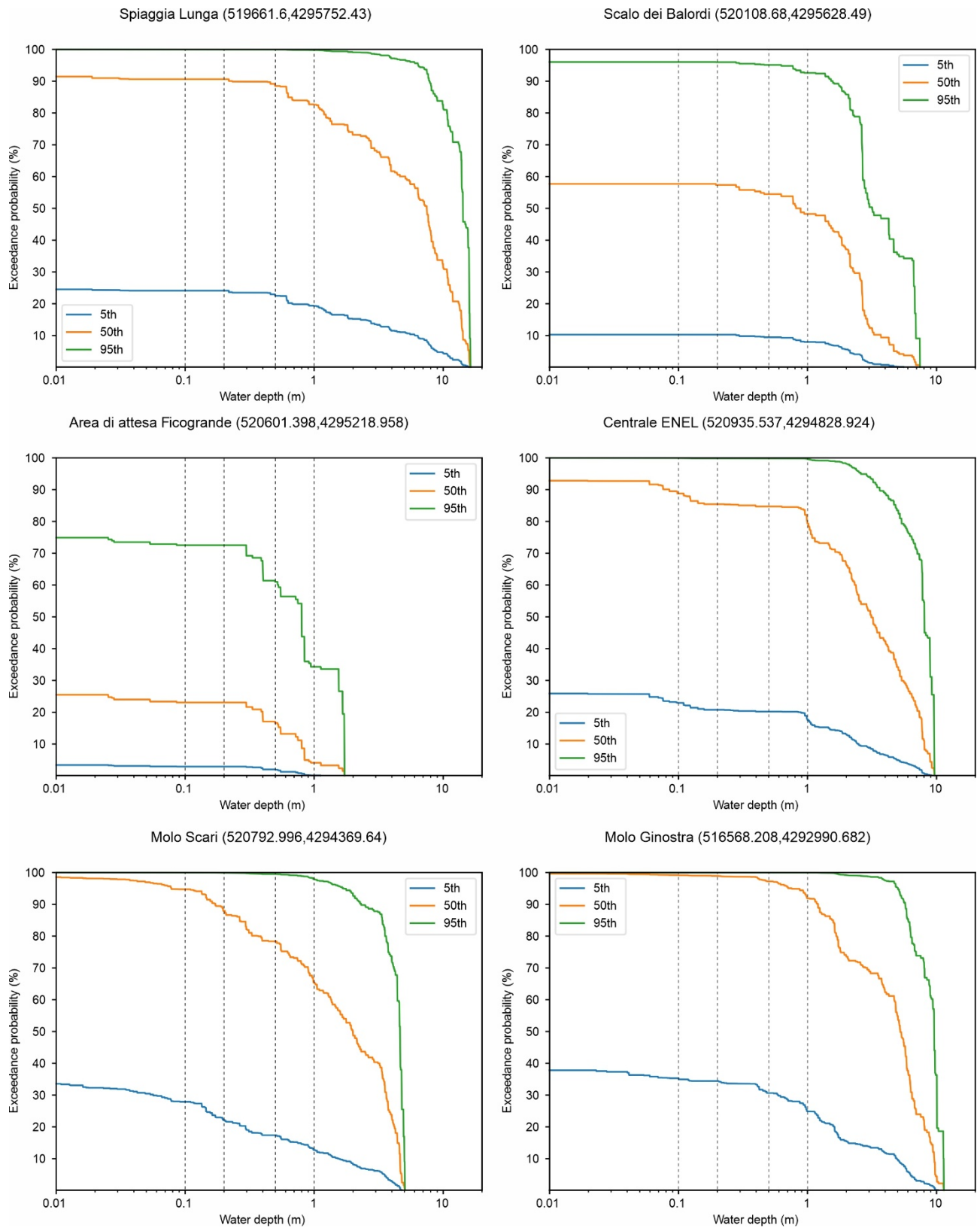
Figure S12. Hazard curves for the 6 sites of Fig. 1 (main manuscript) for Database A, volumes \geq 1 \times 10^6 \text{ m}^3 . Each panel shows the 50-year exceedance probability as a function of water depth for the 5 th , 50 th , and 95 th percentiles of the hazard distribution. Vertical grey dashed lines correspond to the water depth thresholds used for map production (0.1, 0.2, 0.5 and 1 m).
