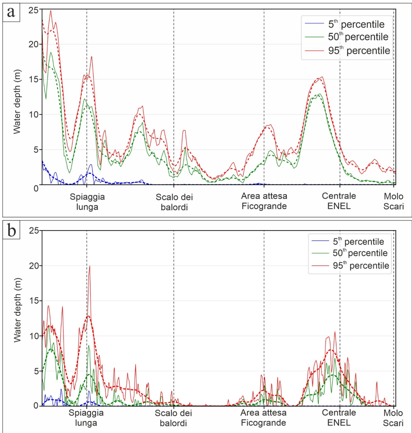
Figure 14 Profiles along the 15 m isoline of the 20m DEM ( 5^{\text{th}} - 50^{\text{th}} - 95^{\text{th}} ) for maps with probability 10% for a) Database A and b) Database B. Vertical dashed lines correspond to the closest point along the 15 m isoline to 5 out of 6 sites where hazard curves have been developed (see Section 3.2.4).
