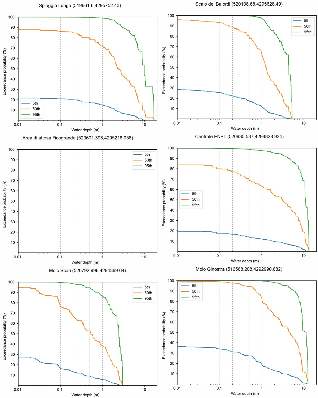
Figure S10. Hazard curves for the 6 sites of Fig. 1 (main manuscript) for Database B, volumes \geq 1 \times 10^6 \text{ m}^3 . Each panel shows the 50-year exceedance probability as a function of water depth for the 5 th , 50 th , and 95 th percentiles of the hazard distribution. Vertical grey dashed lines correspond to the water depth thresholds used for map production (0.1, 0.2, 0.5 and 1 m).
