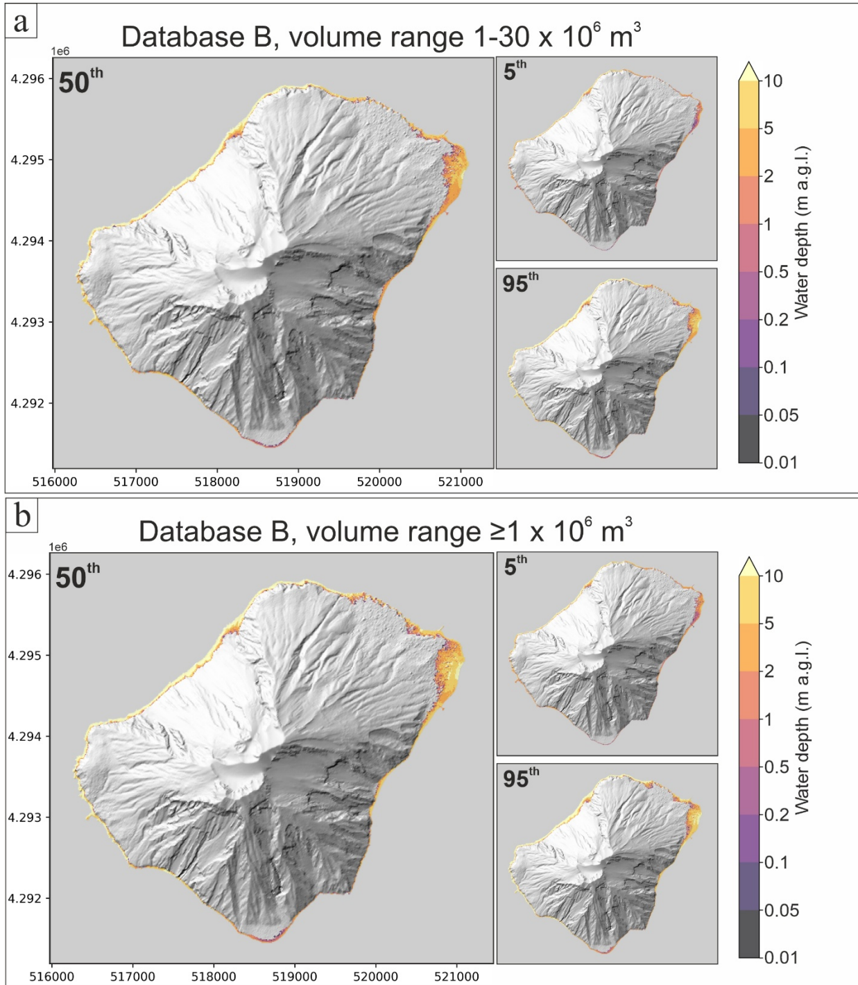
Figure 9. Probabilistic maps showing the inundation water depth corresponding to a 10% exceedance probability over a 50-year horizon for the Database B. (a) Volume range 1\text{--}30 \times 10^6 \text{ m}^3 ; (b) volume range \geq 1 \times 10^6 \text{ m}^3 .
