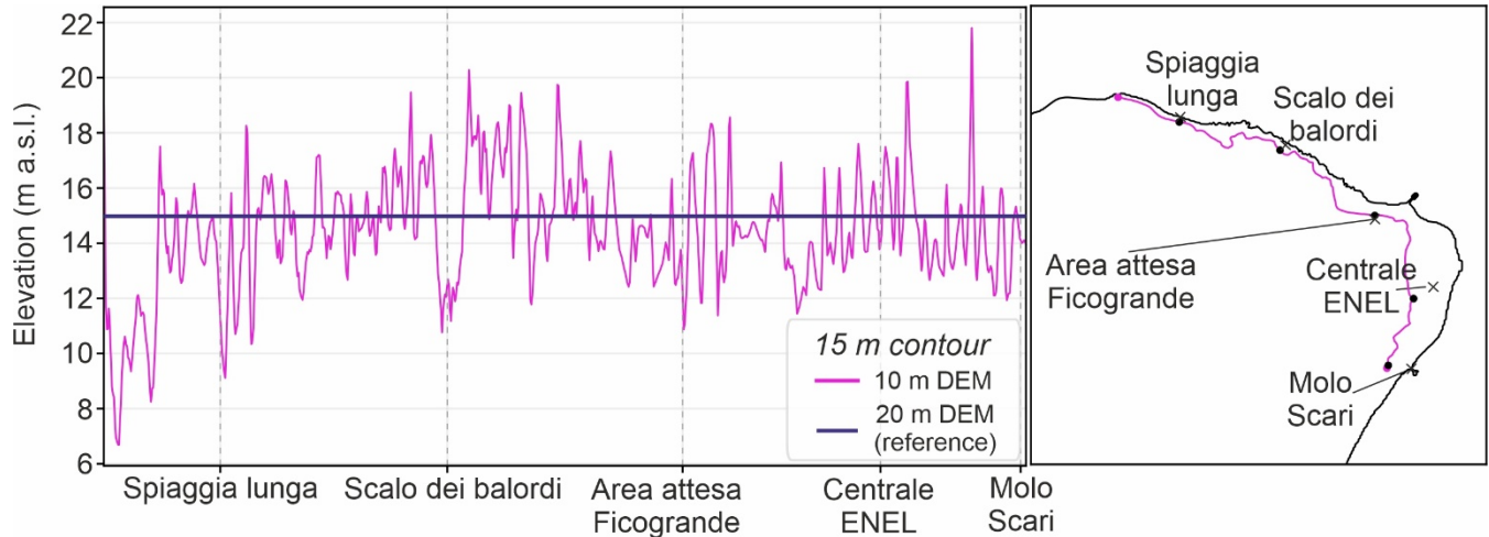
Figure 2. Left: elevation sampled from the 10 m DEM (purple line) along the planimetric path of the 15 m isohypse extracted from the 20 m DEM. The blue horizontal line represents the constant 15 m elevation of the reference contour in the 20 m DEM. Left: Topographic profile extracted from the 10m DEM (purple line) along the 15 m isohypse of the 20m DEM (blue line). Vertical dashed lines correspond to the closest point along the 15 m isohypse (black dots in the map to the right) to 5 out of 6 sites where hazard curves have been developed (black crosses in the map to the right).
