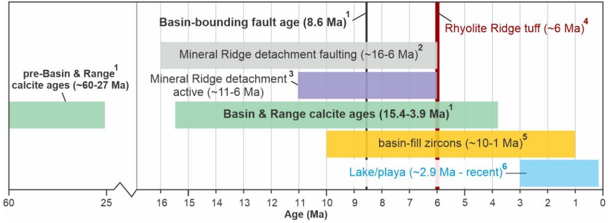
Figure 9. Time plot of U-Pb calcite ages from this study and published constraints on regional tectonic, volcanic, and basin evolution. Data sources (superscripts): 1—this study; 2—Diamond and Ingersoll (2002); 3—Oldow et al. (1994); 4—Darin et al. (2025); 5—Rangel et al. (2025); 6— Coffey et al. (2021) and Gagnon et al. (2023).
