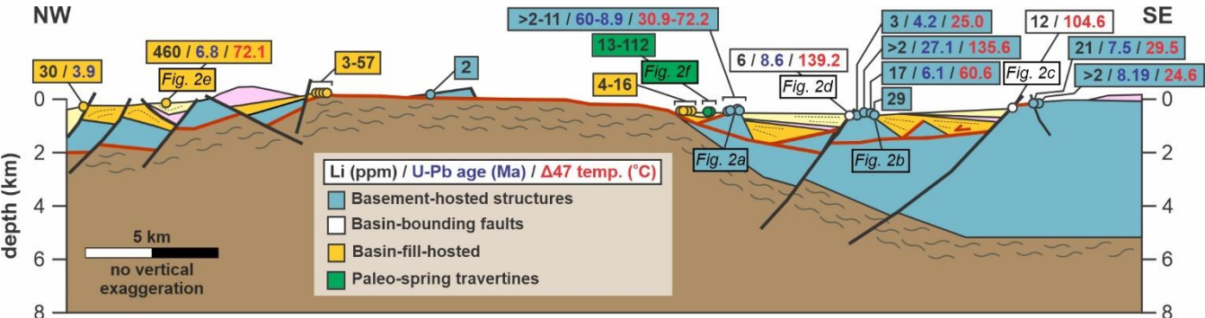
Figure 7. NW-SE cross section across study area (location shown in Fig. 1) showing projected sample locations and lithium concentrations, U-Pb ages, and clumped isotope temperatures. Modified from Cawood et al. (2025) and Rangel et al. (2025). Analytical uncertainties are omitted for clarity (see Fig. 5 and Supplemental Material item 2 for full suite of data and uncertainties).
