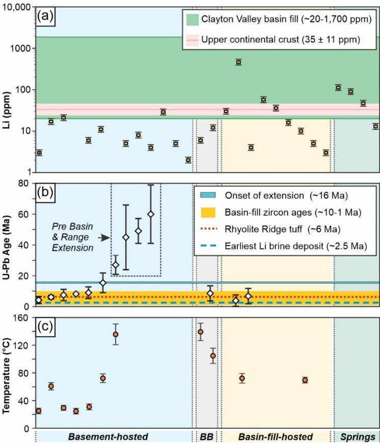
295 Figure 5. Geochemical data for calcite veins and travertine spring deposits. (a) Lithium concentrations (ppm); vertical error bars represent ±10% analytical uncertainty (ALS, 2025). The dark pink horizontal reference bar shows average upper continental
