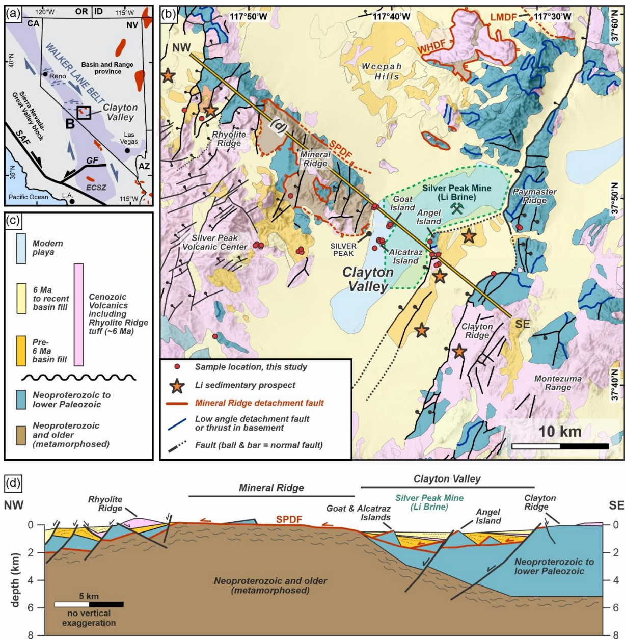
95 Figure 1. Geologic map of Clayton Valley, Nevada. (a) Regional tectonic provinces of the southwestern United States, adapted from 100 Darin et al. (2025). Red polygons mark the position of exposed metamorphic core complexes in the region, including the Mineral Ridge detachment system in Clayton Valley; modified from Davis et al. (2023). (b) Geologic map of the greater Clayton Valley region, modified from Albers and Stewart (1972), U.S. Geological Survey (2024), and Darin et al. (2025). (c) Generalized stratigraphy. Formation names and approximate ages after Diamond and Ingersoll (2002). (d) Schematic NW-SE cross section across the study area (location shown in part b), illustrating the first-order tectonostratigraphic framework of Clayton Valley. Cross-section geometry is based on Diamond and Ingersoll (2002), Ogilvie et al. (2023), Darin et al. (2025), and subsurface constraints from Coffey et al. (2021). Abbreviations: OR, Oregon; ID, Idaho; NV, Nevada; CA, California; AZ, Arizona; SAF, San Andreas Fault; GF, Garlock Fault; L.A., Los Angeles; ECSZ, Eastern California Shear Zone; SPDF, Silver Peak detachment fault; WHDF, Weepah Hills detachment fault; LMDF, Lone Mountain detachment fault.
