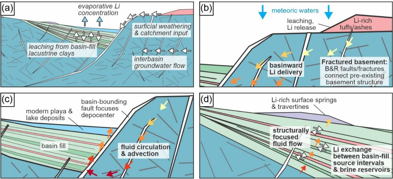
505 Figure 11. Conceptual model of structurally focused lithium transport and redistribution. (a) Previous workers' concepts of lithium transport and delivery at Clayton Valley (e.g., Coffey et al., 2021; Darin et al., 2025). (b) Linkage between basement and basin structures, leaching of lithium from silicic volcanic units, fault-controlled delivery of lithium-bearing fluids into developing basin accommodation space. (c) Advective circulation involving downwelling cooler fluids and upwelling warmer fluids. (d) Lithium exchange between basin-fill source intervals and brine reservoirs. B&R = Basin and Range.
