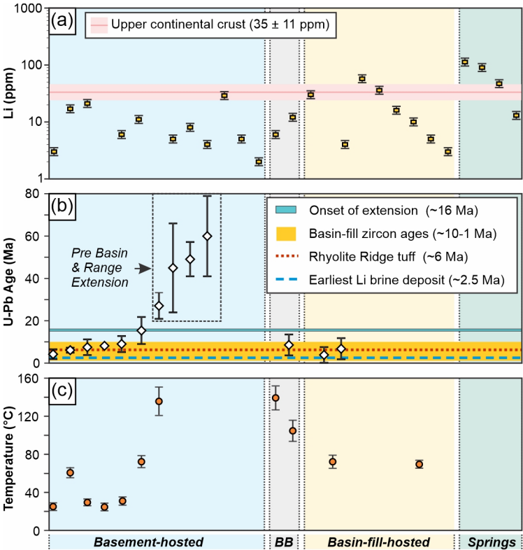
Figure 5. Geochemical data for calcite veins and travertine spring deposits. (a) Lithium concentrations (ppm); vertical error bars represent \pm 10\% analytical uncertainty (ALS, 2025). The dark pink horizontal reference bar shows average upper continental crust lithium concentration of 35 ppm from Teng et al. (2004), and the light pink band shows the reported \pm 11 ppm uncertainty, corresponding to 24–46 ppm. (b) U–Pb calcite ages (Ma); vertical error bars indicate 2\sigma uncertainty. Horizontal bars indicate onset of Basin and Range extension in the Clayton Valley–Silver Peak region (Diamond and Ingersoll, 2002), basin-fill zircon ages (Rangel
