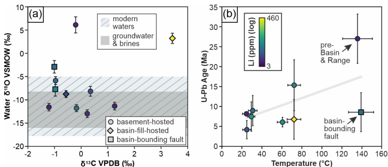
Figure 8. (a) Reconstructed fluid \delta^{18}\text{O} (VSMOW) versus carbonate \delta^{13}\text{C} (VPDB). Shaded fields show representative ranges of modern meteoric recharge and groundwater/brines for Clayton Valley (Gagnon et al., 2023). (b) U-Pb calcite age versus clumped-isotope temperature.
