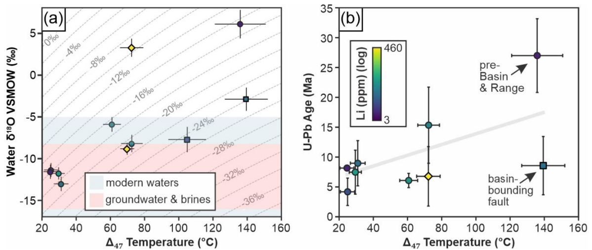
Figure 8. (a) Reconstructed fluid \delta^{18}\text{O} (VSMOW) versus \Delta_{47} temperature. Dashed contours show equilibrium calcite \delta^{13}\text{C} (‰) (VPDB) calculated using the fractionation relationship of Kim and O'Neil (1997). Shaded fields show representative ranges of modern meteoric recharge and groundwater/brines for Clayton Valley (Gagnon et al., 2023). (b) U-Pb calcite age versus clumped-isotope temperature. Symbols in both panels indicate structural setting (circles = basement-hosted structures; diamonds = basin-fill-hosted structures; squares = basin-bounding faults). Symbol colours indicate calcite lithium concentration.
