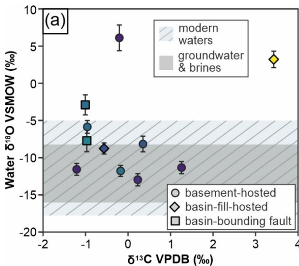
Figure 68. (a) Reconstructed fluid \delta^{18}\text{O} (VSMOW) versus carbonate \delta^{13}\text{C} (VPDB). Shaded fields show representative ranges of modern meteoric recharge and groundwater/brines for Clayton Valley (Gagnon et al., 2023). (b) U-Pb calcite age versus clumped-isotope temperature.
