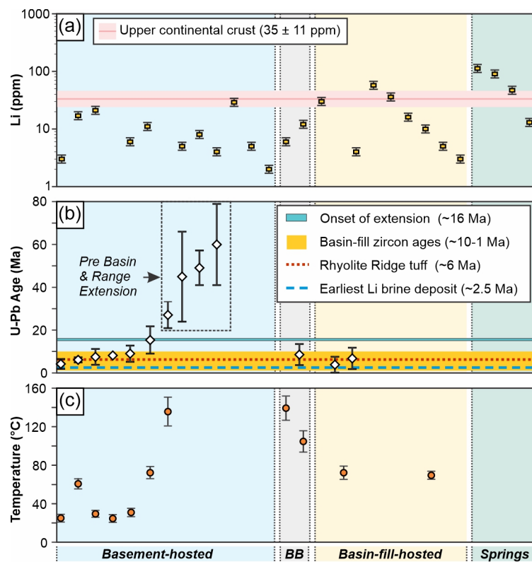
Figure 35. Geochemical data for calcite veins and travertine spring deposits. (a) Lithium concentrations (ppm); vertical error bars represent \pm 10\% analytical uncertainty (ALS, 2025). The dark pink horizontal bars show average upper continental crust lithium concentrations (Watts, 2025) and published bulk vein calcite lithium concentrations (Drake concentration of 35 ppm from Teng et al., 2018), (2004), and the light pink band shows the reported \pm 11 ppm uncertainty, corresponding to 24–46 ppm. (b) U–Pb calcite ages (Ma); vertical error bars indicate 2\sigma uncertainty. Horizontal bars indicate onset of Basin and Range extension in the Clayton Valley–Silver Peak region (Diamond and Ingersoll, 2002), basin-fill zircon ages (Rangel et al., 2025), the Rhyolite Ridge tuff (Darin et al., 2025), and earliest halite deposition in Clayton Valley (Coffey et al., 2021; Gagnon et al., 2023). Ages older than the onset of Basin and Range extension ( \sim 25 Ma; Stewart, 1998) are highlighted. (c) Clumped-isotope temperatures ( ^{\circ}\text{C} ); vertical error bars represent 1\sigma uncertainty. Shaded vertical bands in panels A–C indicate sample setting; BB = basin-bounding faults.
