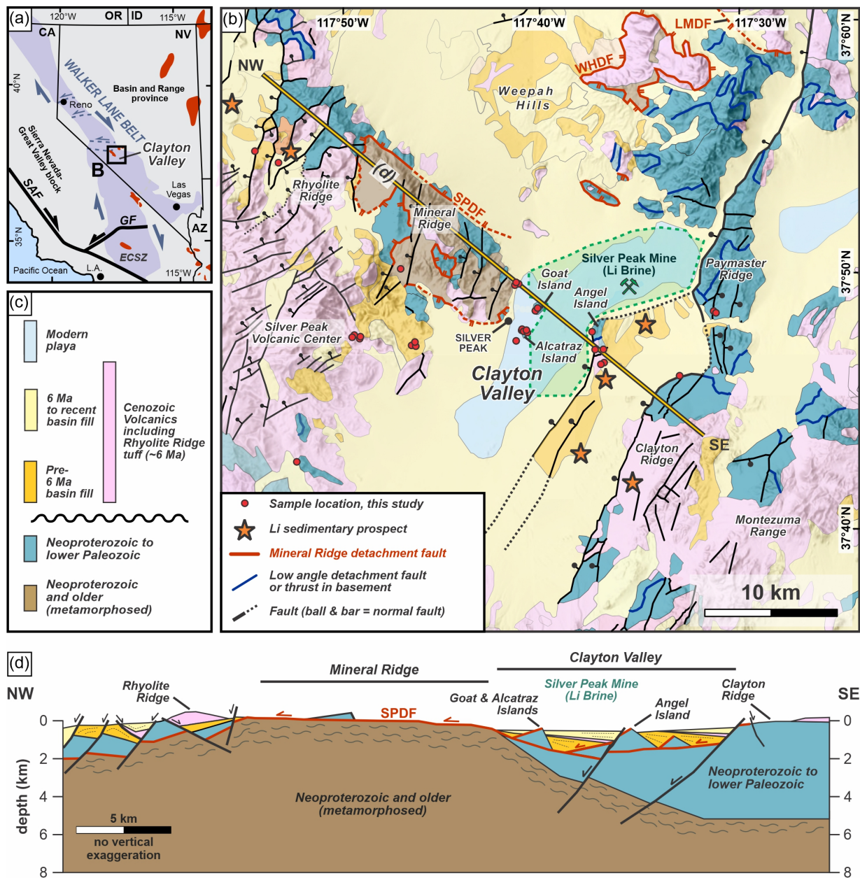
Figure 1. Geologic map of Clayton Valley, Nevada. (a) Regional tectonic provinces of the southwestern United States, adapted from Darin et al., (2025). Red polygons mark the position of exposed metamorphic core complexes in the region, including the Mineral Ridge detachment system in Clayton Valley; modified from Davis et al., (2023). (b) Geologic map of the greater Clayton Valley region, modified from Albers and Stewart (1972), U.S. Geological Survey (2024), and Darin et al. (2025). (c) Generalized stratigraphy. Formation names and approximate ages after Diamond and Ingersoll (2002). (d) NW-SE cross-section across study area (location shown in part b). (d) Schematic NW-SE cross section across the study area (location shown in part b), illustrating the first-order tectonostratigraphic framework of Clayton Valley. Cross-section geometry is based on Diamond and Ingersoll (2002), Ogilvie et al. (2023), Darin et al. (2025), and subsurface constraints from Coffey et al. (2021). Abbreviations: OR, Oregon; ID, Idaho; NV, Nevada; CA, California; AZ, Arizona; SAF, San Andreas Fault; GF, Garlock Fault; L.A., Los Angeles; ECSZ, Eastern
