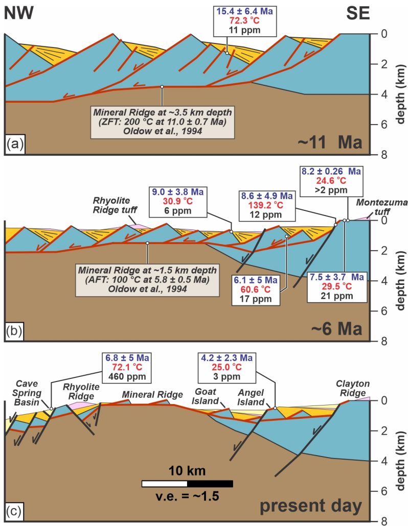
Figure 810. Schematic structural evolution of Clayton Valley at (a) ca. 3–11 Ma to present , (b) ca. 6–5 Ma , (c) ca. 11–1 Ma , and (d) ca. 16 Ma . Modified from Rangel et al. (2025). Vein calcite sample ages (blue), temperatures (red), and lithium concentrations (black) are shown relative to the evolving basin architecture. Samples are plotted at approximate time intervals when they are interpreted, based on U–Pb ages, to have already been present; panels do not imply fault initiation or mineralization at the illustrated times. Approximate paleodepth estimates for Mineral Ridge at ca. 6 Ma and ca. 11 Ma are based on published apatite and zircon fission-track constraints from Oldow et al. (1994) and assume an elevated geothermal gradient of 50 °C km -1 associated with regional extension and crustal thinning.
