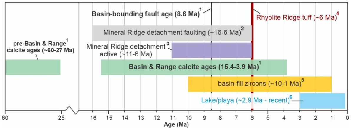
Figure 79. Time plot of U-Pb calcite ages from this study and published constraints on regional tectonic, volcanic, and basin evolution. Data sources (superscripts): 1—this study; 2—Diamond and Ingersoll (2002); 3—Oldow et al. (1994); 4—Darin et al. (2025); 5—Rangel et al. (2025); 6—Coffey et al. (2021) and Gagnon et al. (2023).
