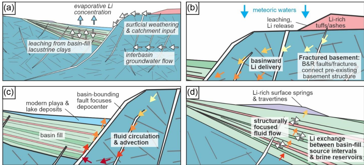
Figure 911. Conceptual model of structurally focused lithium transport and redistribution. (a) Previous workers' concepts of lithium transport and delivery at Clayton Valley (e.g., Coffey et al., 2021; Darin et al., 2025). (b) Linkage between basement and basin structures, leaching of lithium from silicic volcanic units, fault-controlled delivery of lithium-bearing fluids into developing basin accommodation space. (c) Advective circulation involving downwelling cooler fluids and upwelling warmer fluids. (d) Lithium exchange between basin-fill source intervals and brine reservoirs. B&R = Basin and Range.
