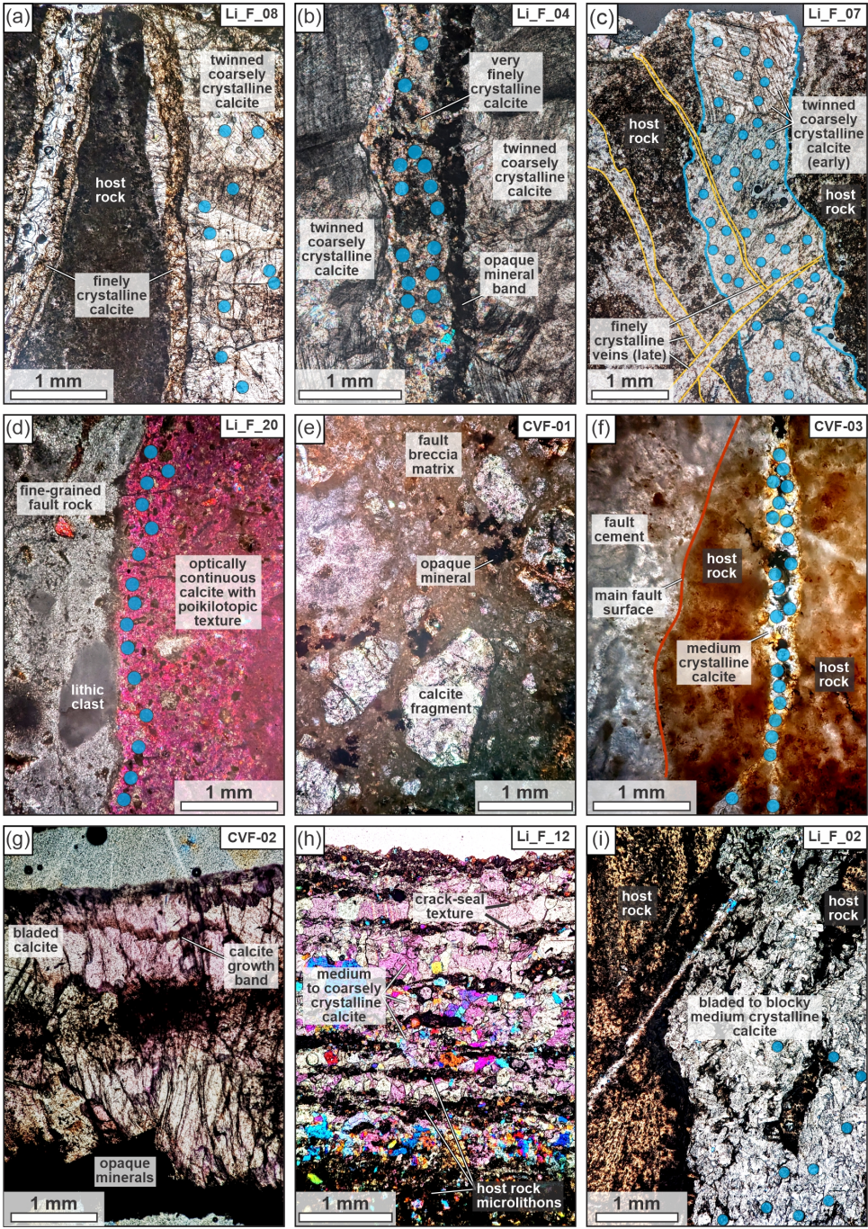
Figure 4. Representative petrographic images of sampled structures. Panels (a-i) correspond directly to the field photographs shown in Figure 3. (a, b) Basement-hosted opening-mode veins. (c, d) Basement-hosted faults and associated mineralization. (e, f) Basin-bounding and major basin-margin faults. (g, h) Opening-mode veins hosted within basin-fill deposits. (i) Basin-fill-hosted normal
