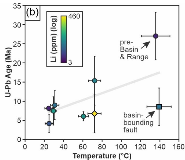
Figure 68. (a) Reconstructed fluid \delta^{18}\text{O} (VSMOW) versus carbonate \delta^{13}\text{C} (VPDB). Shaded fields show representative ranges of modern meteoric recharge and groundwater/brines for Clayton Valley (Gagnon et al., 2023). (b) U-Pb calcite age versus clumped-isotope temperature.
