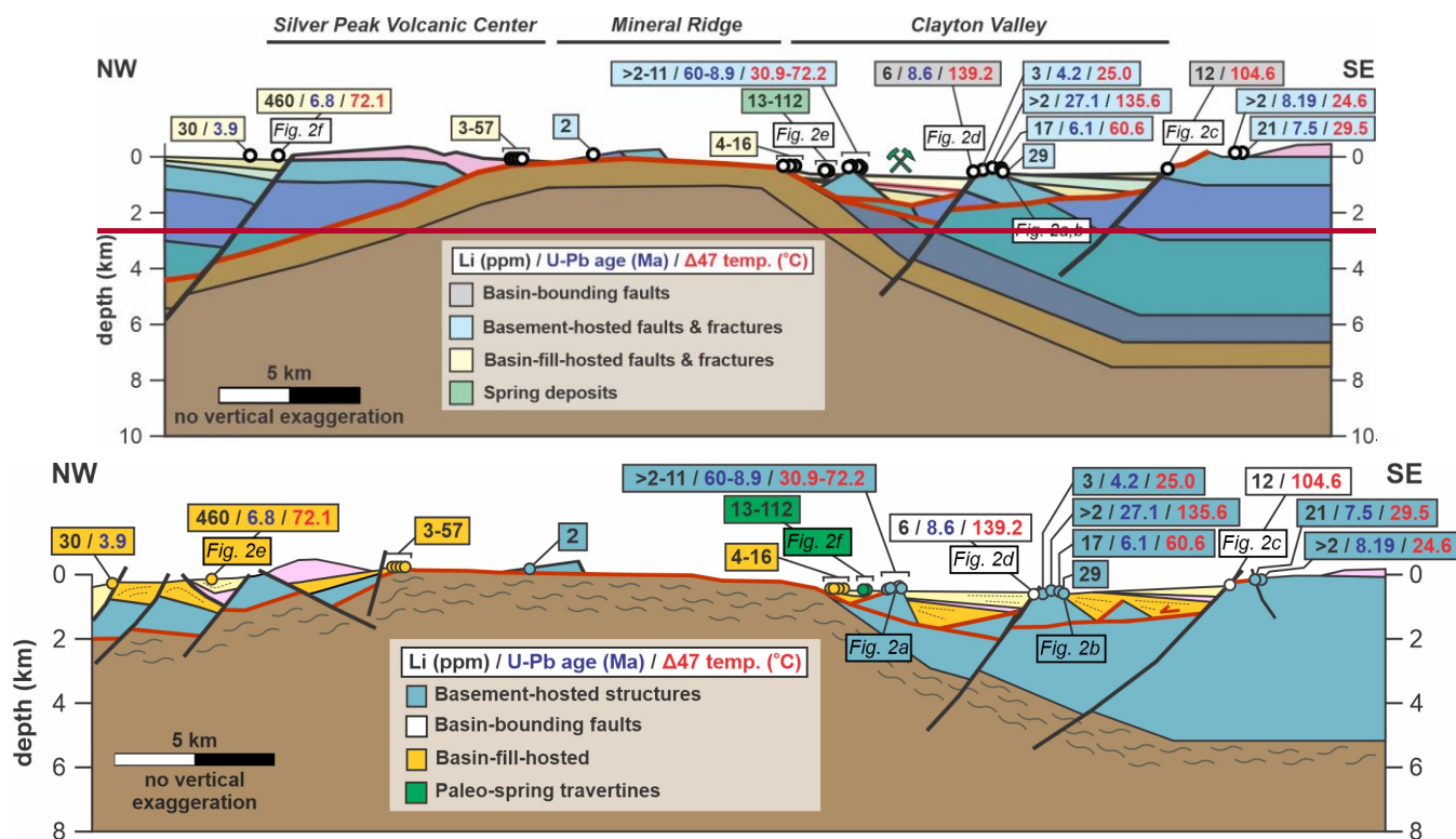
Figure 57. NW-SE cross section across study area (location shown in Fig. 1) showing projected sample locations and lithium concentrations, U-Pb ages, and clumped isotope temperatures. Modified from Cawood et al. (2025) and Rangel et al. (2025). Analytical uncertainties are omitted for clarity (see Fig. 35 and Supplemental Material item 42 for full suite of data and uncertainties).
