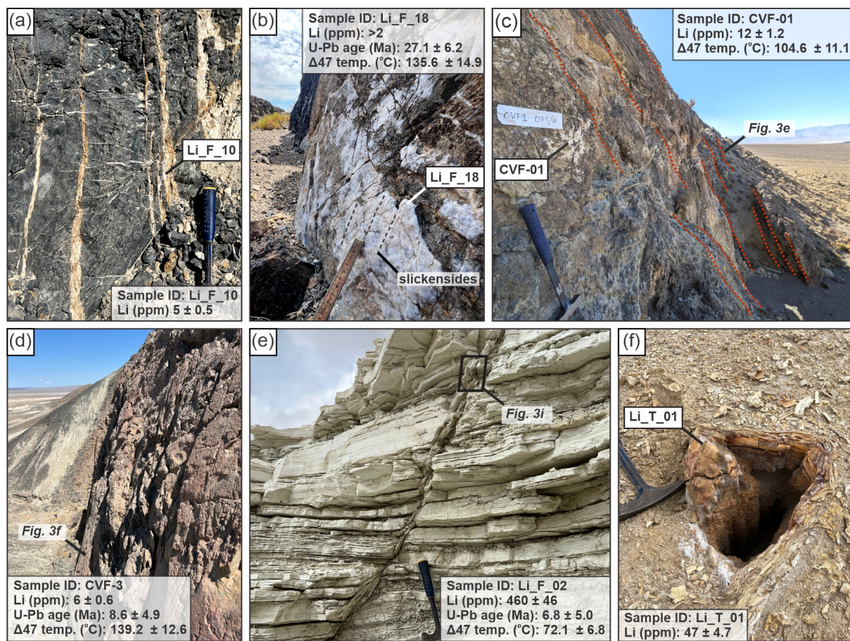
Figure 2. Examples of sample types and settings collected for geochemical analysis. (a) Basement-hosted opening-mode vein; view to the north. (b) Basement-hosted normal fault with cemented breccia fill. This structure is characterised by slickensided calcite mineralization. View to the northeast. (c, d) Basin-bounding faults. (c) A west-dipping normal fault at west side zone that defines the eastern margin of Clayton Ridge Valley. The fault zone includes multiple slip surfaces (red dotted lines) in basement rocks and overlying alluvial fan deposits. View to the south. (d) Major fault on the west flank of Angel Island; view to the north; fault scarp is ca. 15 m high. (e) Calcite-mineralized dilational normal fault hosted within basin-fill sediments; view to the north. (f) Paleohot spring deposit associated with fault-controlled fluid discharge and spring precipitation. (f) Calcite-mineralized fault hosted within basin-fill sediments; view to the north. Red dotted lines in parts a and b delineate structure sampled. Note, in both a and b sampled structures strike approximately N-S and cut across older veins in basement units.
