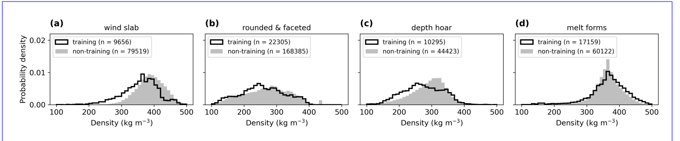
Figure 3. Probability density distribution of snow density for different snow classes derived from SMP profiles. Panels correspond to (a) wind slab, (b) rounded and faceted grains, (c) depth hoar, and (d) melt-freeze forms. For each class, the distributions are shown separately for manually classified samples used in model training (black) and samples not used during training that were automatically classified by the algorithm (grey). Numbers in the legends indicate the number of samples (n) in each subset. The similar distributions between training and non-training data suggest that the training dataset is representative of the overall data distribution.
