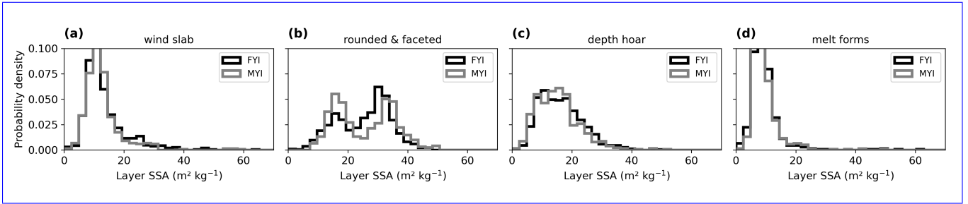
Figure 4. Probability density distributions of the Snow Specific Surface Area (SSA) for different snow classes on first-year ice (FYI, black) and multi-year ice (MYI, grey). Panels show distributions for (a) wind slab, (b) rounded/faceted grains, (c) depth hoar, and (d) melt-freeze forms. SSA values are derived from SMP measurements, and snow classes are obtained from the SMP-based classification. The differences in, and SSA is calculated as a mean value for each individual snow type-layer. SSA differs significantly between ice regimes are generally only for depth hoar, although the difference is small.
