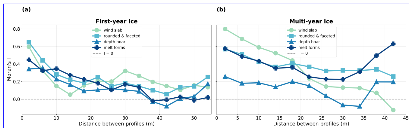
Figure 7. Spatial autocorrelation of fractional snowpack composition for different snow classes. Moran's I is calculated for the fractional occurrence of wind slab, rounded and faceted grains, depth hoar, and melt-freeze forms within individual snow profiles derived from SMP-based classifications. The results are shown separately for (a) FYI and (b) MYI. The x-axis represents the lag distance between pairs of SMP profiles along measurement transects. The dashed horizontal line indicates zero spatial autocorrelation. At larger lag distances, particularly for MYI beyond 45m, too few profile pairs contribute to the estimate, leading to a shortened transect analysis.
