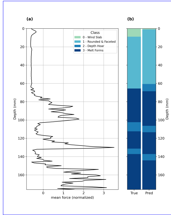
Figure 2. Example SnowMicroPen (SMP) profile and corresponding snow type classification. The left panel shows (a) the mean penetration force averaged over 1 mm depth bins as a function of depth. The right panel: (b) compares the manually assigned snow type classification (“True”) with the algorithm-predicted classification (“Pred”). Colors indicate the four snow classes used in the model: wind slab, rounded/faceted grains, depth hoar, and melt-freeze forms.
