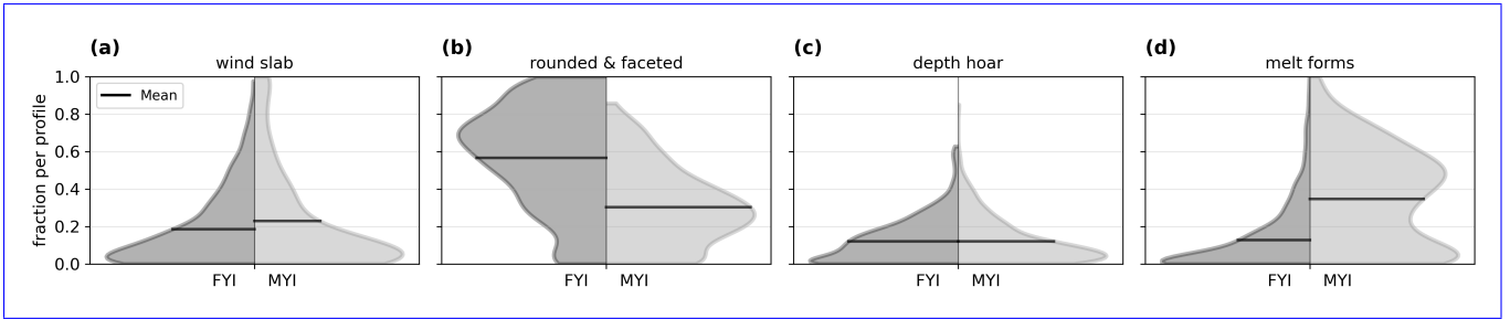
Figure 6. Fractional snowpack composition for different snow classes on first-year ice (FYI, dark grey) and multi-year ice (MYI, light grey). Panels show the fraction of (a) wind slab, (b) rounded and faceted grains, (c) depth hoar, and (d) melt-freeze forms within individual snow profiles. The half-violin plots illustrate the distribution across all profiles, with black bars denoting mean fractions. Snow classes and snow type fractions are derived from the SMP–based classification.
