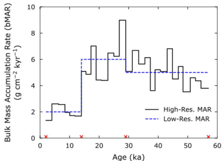
Figure 1: Simple representation of bMAR dependence on the resolution of the available age model. The two lines are separate determinations of bMAR over the last ~60 kyr for a hypothetical marine sediment core using two age models of different resolutions. The red crosses denote four tie-points for the original, low-resolution age model, and the blue dashed line is the sediment bMAR based on this lower-resolution age model. The black line represents a sediment bMAR calculated using a higher resolution age model produced after the original. Note the substantial changes in bMARs that go unrecognized with lower-resolution age model, while still producing the same overall average bMAR for the wider interval.
