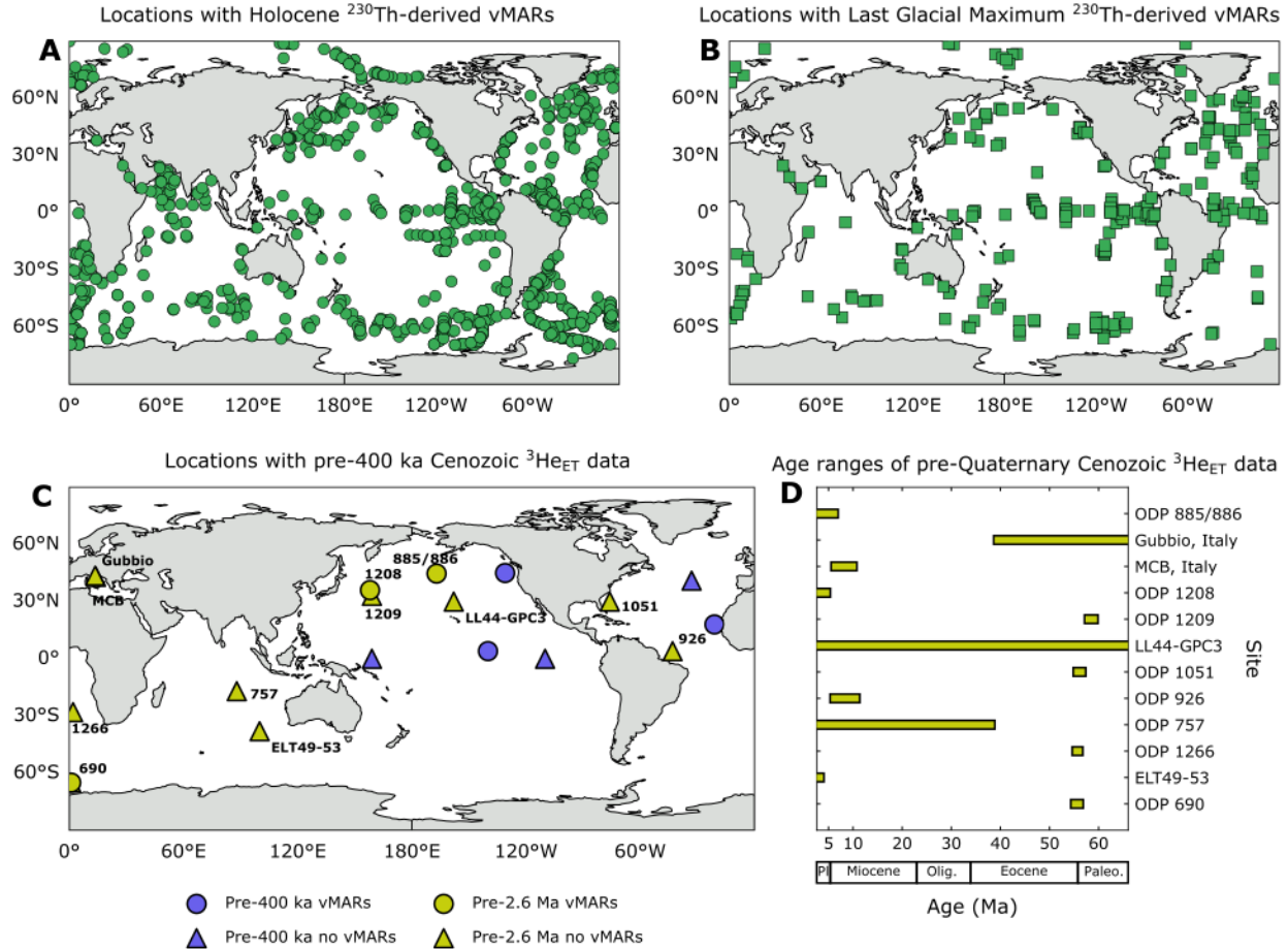
Figure 3: Available constant flux proxy data for various time intervals. A) Locations with Holocene (0-5 ka) ^{230}\text{Th} -normalized sediment vMAR data (Costa et al., 2020). B) Locations of Last Glacial Maximum (18-23 ka) ^{230}\text{Th} -normalized sediment vMARS (Costa et al., 2020). C) Locations with any marine sediment ^3\text{He}_{\text{ET}} (or just ^3\text{He} ) data for the Cenozoic prior to 400 ka. No studies that produced ^3\text{He}_{\text{ET}} data from only 0-400 ka (i.e., the approximate range where ^{230}\text{Th} can be applied) or prior to the Cenozoic are included here. Purple symbols indicate sites with ^3\text{He}_{\text{ET}} data that fall only within the Quaternary prior to 400 ka (Farley and Patterson, 1995; Middleton et al., 2020; O'Mara et al., 2022, 2024; Patterson and Farley, 1998; Winckler et al., 2005a). Yellow symbols represent sites with at least some ^3\text{He}_{\text{ET}} data for the Cenozoic prior to the Quaternary (Abell et al., 2021, 2023; Abell and Winckler, 2023; Farley, 1995; Farley et al., 2006; Farley and Eltgroth, 2003; Graham and Konrad, 2022; Marcantonio et al., 2009; Montanari et al., 2017; Mukhopadhyay et al., 2001b; Murphy et al., 2010). Circles indicate sites where ^3\text{He}_{\text{ET}} data have been used to calculate sediment constituent vMARS (Abell et al., 2021, 2023; Abell and Winckler, 2023; Middleton et al., 2020; O'Mara et al., 2022, 2024; Torfstein et al., 2010). Triangles represent sites where ^3\text{He}_{\text{ET}} data are not used to determine sediment constituent vMARS. These studies either 1) determine an influx of ^3\text{He}_{\text{ET}} using the site's age model (Farley, 1995; Farley et al., 2006; Farley and Patterson, 1995; Graham and Konrad, 2022; Montanari et al., 2017; Mukhopadhyay et al., 2001a; Patterson and Farley, 1998; Winckler et al., 2004) or 2) determine a flux of ^3\text{He}_{\text{ET}} using the site's age model and then calculate sediment accumulation rates and/or event durations using this value (Farley and Eltgroth, 2003;
