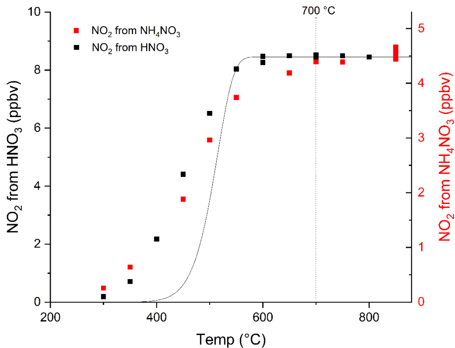
505 Figure 2. Temperature dependent dissociation (thermograms) of HNO 3 and NH 4 NO 3 to NO 2 in the TD-inlet. The vertical, dotted line indicates at which temperature the TD-inlets are operated in normal operation (i.e. in the plateau of the thermogram). The solid curve is the calculated conversion of HNO 3 to NO 2 using a temperature dependent rate coefficient for the thermal dissociation of HNO 3 in the gas-phase (see text for details) and is scaled to match the plateau in the measured signal at high temperatures.
