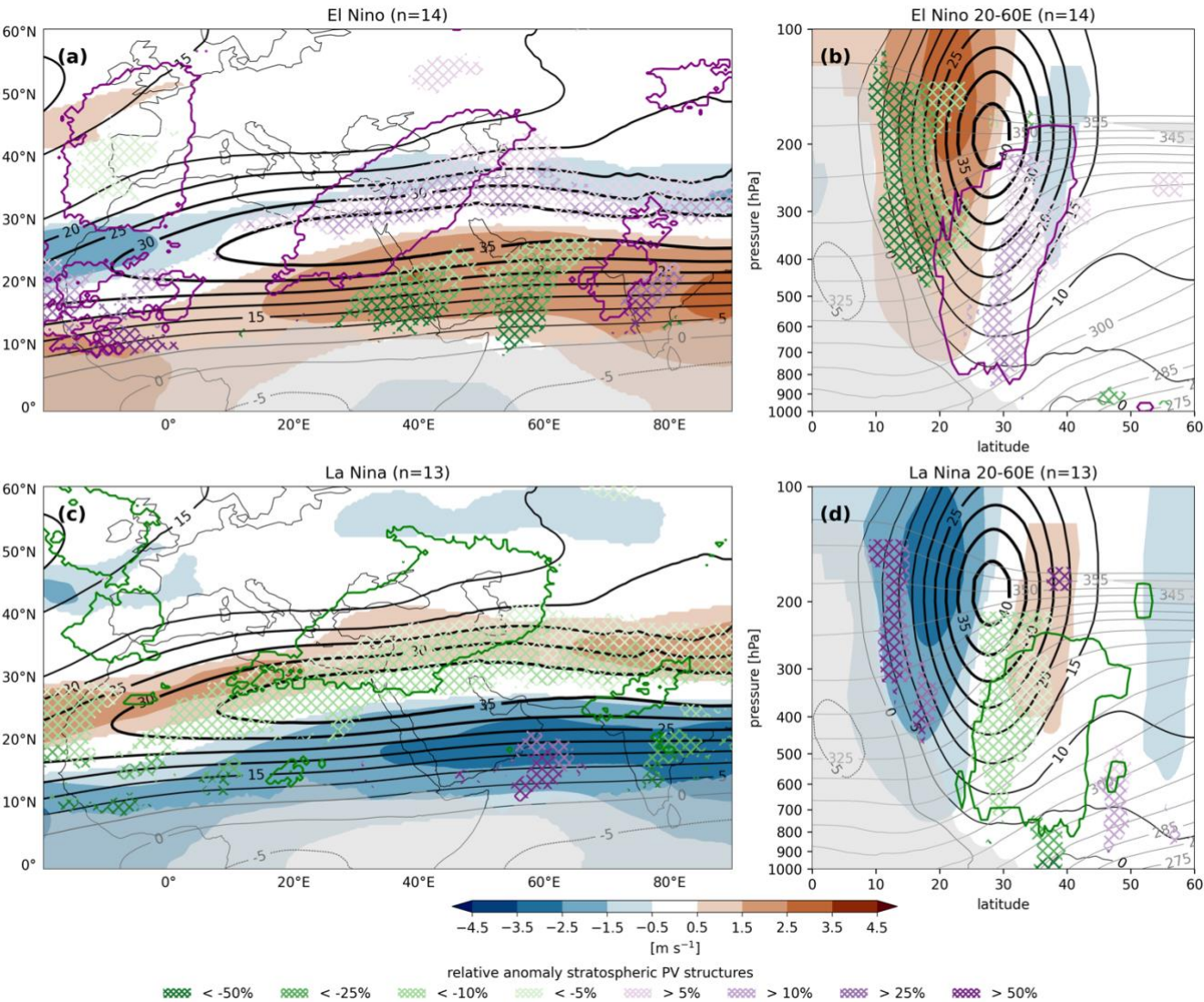
615 Figure 5. Composites of anomalies in cool-season zonal wind and Rossby wave breaking frequencies for (a,b) El Niño and (c,d) La Niña events. (a,c) 250-hPa zonal wind anomalies in colors and relative anomalies of stratospheric PV structure frequencies – aggregated over 300-350K - in hatching, as indicated by the legend. (b,d) The zonal mean (20-60°E) zonal wind anomalies in colors and relative anomalies of stratospheric PV structure frequencies in hatching at pressure levels interpolated from data on isentropic surfaces between 275 and 360 K with 5 K intervals. These isentropic surfaces are plotted in grey contours. Zonal wind and Rossby wave breaking anomalies are only shown where considered significant at p < 0.1 . Gray shading denotes regions where climatological frequencies of vertically aggregated PV structure occurrences over 300-350K in (a,c) are below 25 counts and of PV structure occurrences in (b,d) fall below 5 counts. For reference, regions where relative anomalies in stratospheric PV structure frequencies exceed 10% for precipitation events are outlined in green contours in (a,b), while those falling below -10% for dry-day events are outlined in purple contours in (c,d). 620
