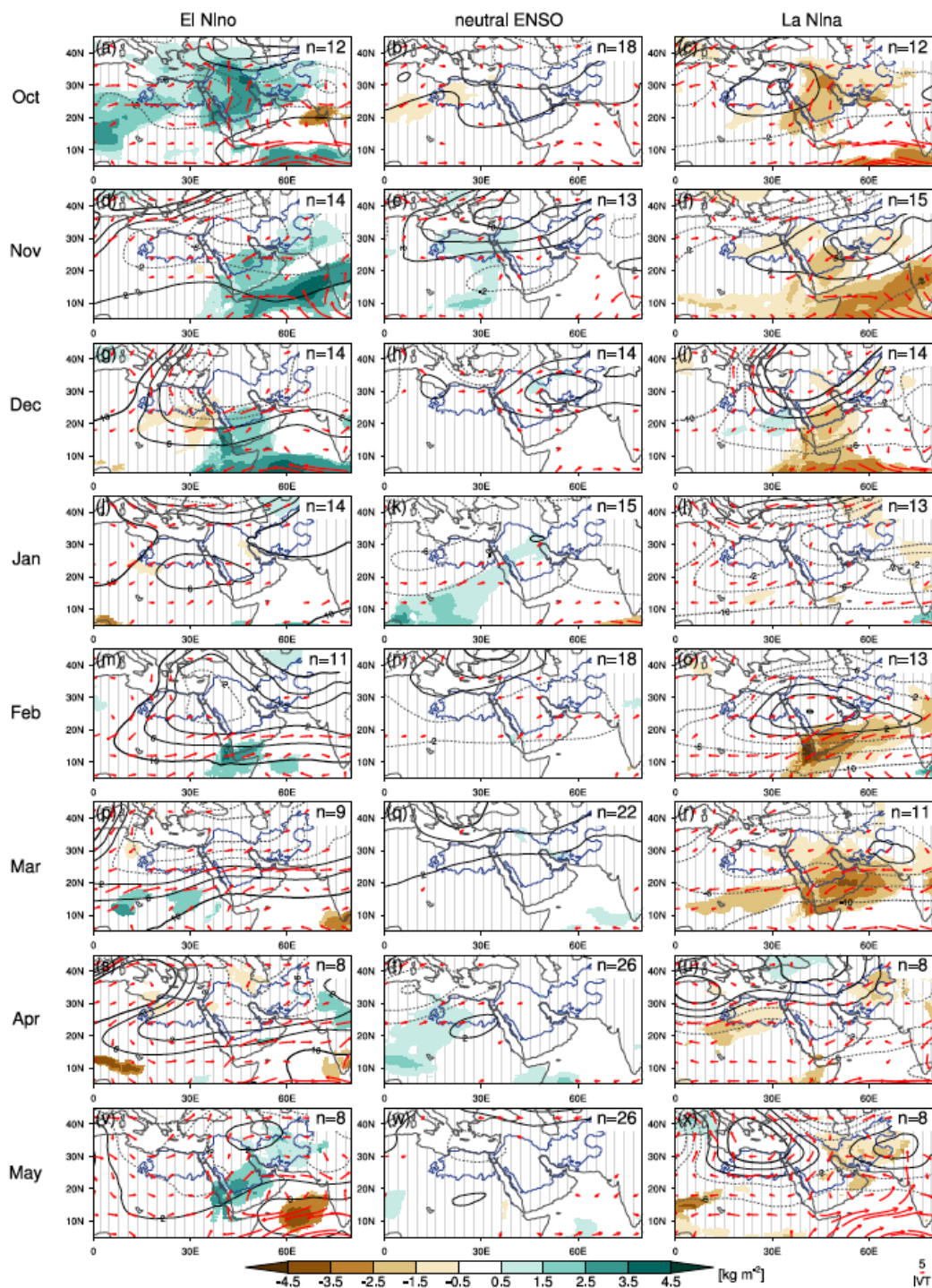
690 Figure A4. As Fig. 7 but for individual months from October to May in rows and the ENSO phases - warm, neutral, and cold - in columns. The ENSO phases are defined based on 3-monthly running mean SST anomalies in the Nino3.4 region. Sample sizes are indicated in text in the top right of each panel.
