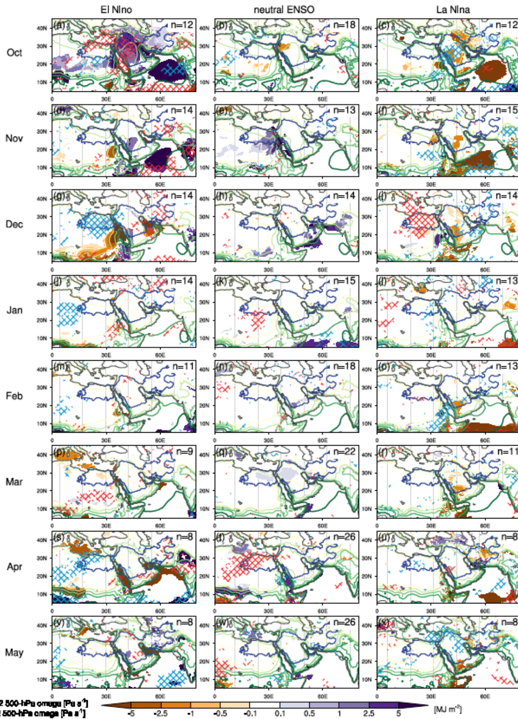
Figure A5. As Fig. 9 but for individual months from October to May in rows and the ENSO phases - warm, neutral, and cold - in columns. The ENSO phases are defined based on 3-monthly running mean SST anomalies in the Nino3.4 region. Sample sizes are indicated in text in the top right corner of each panel.
