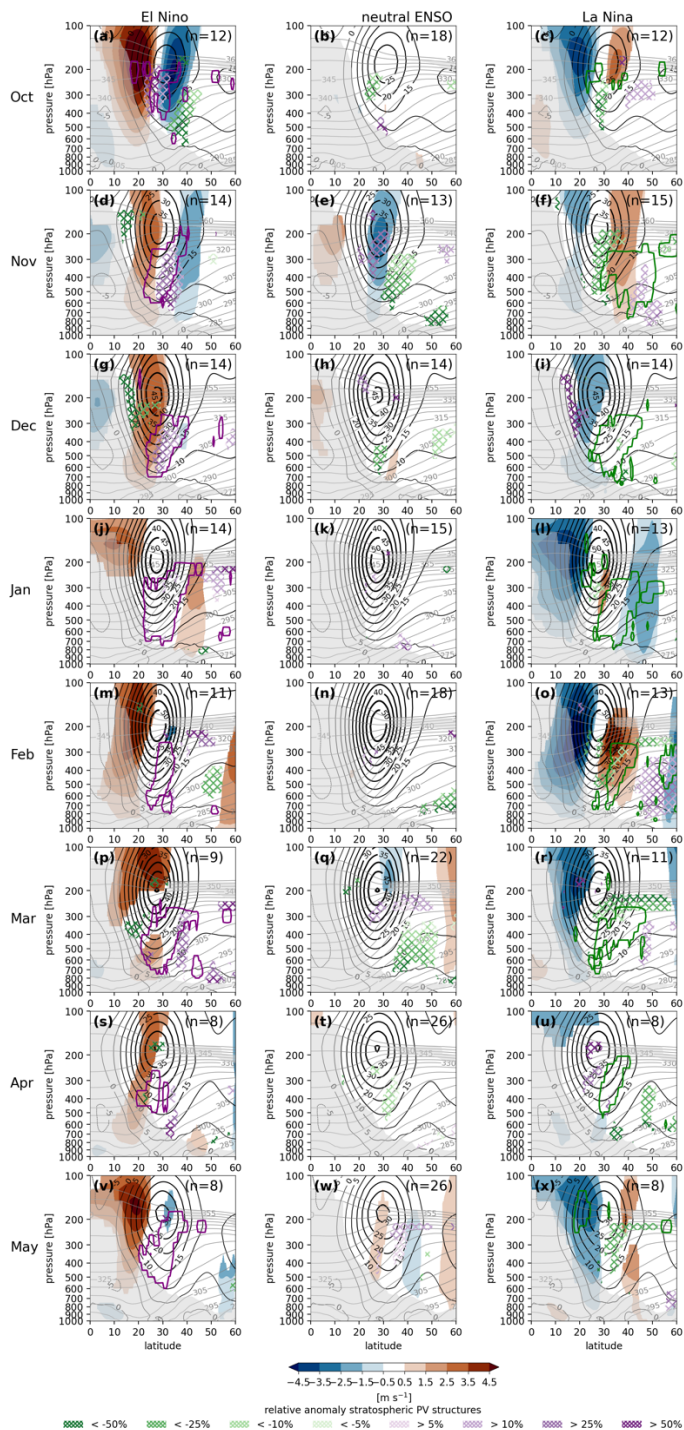
700 Figure A3. As Fig. 5(b,d) but for individual months from October to May in rows and the ENSO phases - warm, neutral, and cold - in columns. The ENSO phases are defined based on 3-monthly running mean SST anomalies in the Nino3.4 region. Sample sizes are indicated in text in the top right corner of each panel.
