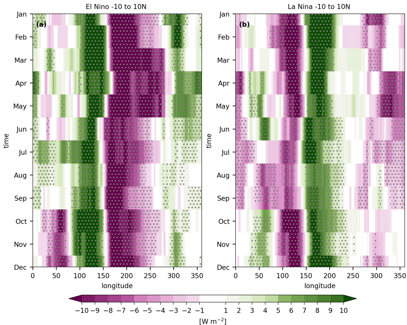
Figure 12. Hovmöller diagrams with anomalies in the Equatorial average ( 10^{\circ}\text{S} - 10^{\circ}\text{N} ) outgoing longwave radiation as a function of longitude and time for (a) El Niño and (b) La Niña conditions with negative anomalies corresponding to enhanced tropical convection and positive anomalies to reduced convection.
