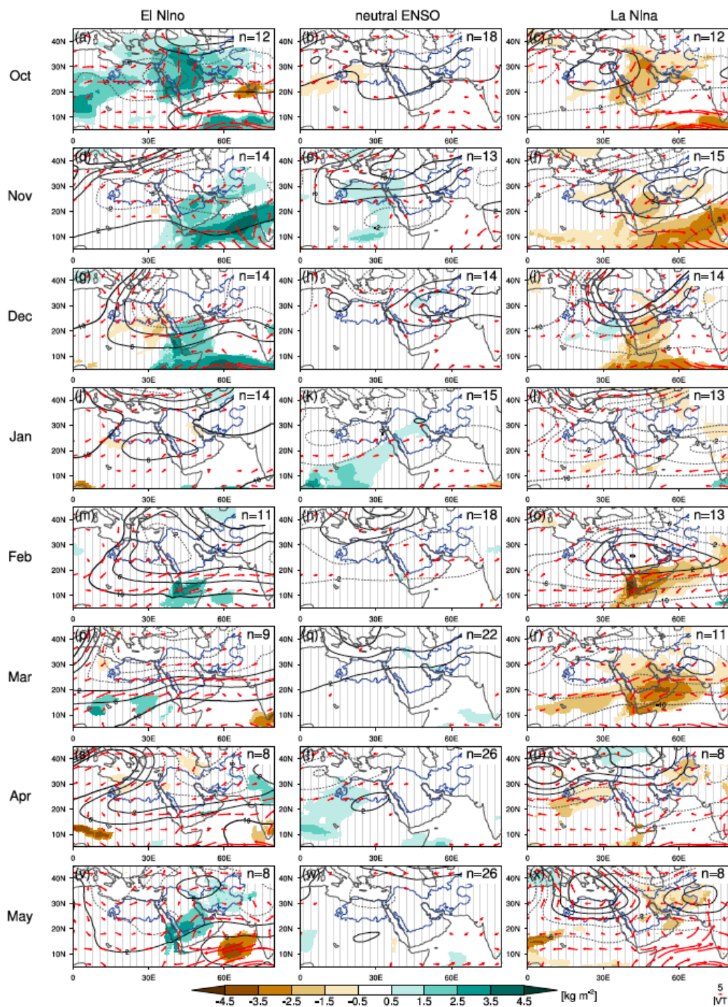
Figure A4. As Fig. 7 but for individual months from October to May in rows and the ENSO phases - warm, neutral, and cold - in columns. The ENSO phases are defined based on 3-monthly running mean SST anomalies in the Nino3.4 region. Sample sizes are indicated in text in the top right corner of each panel.
