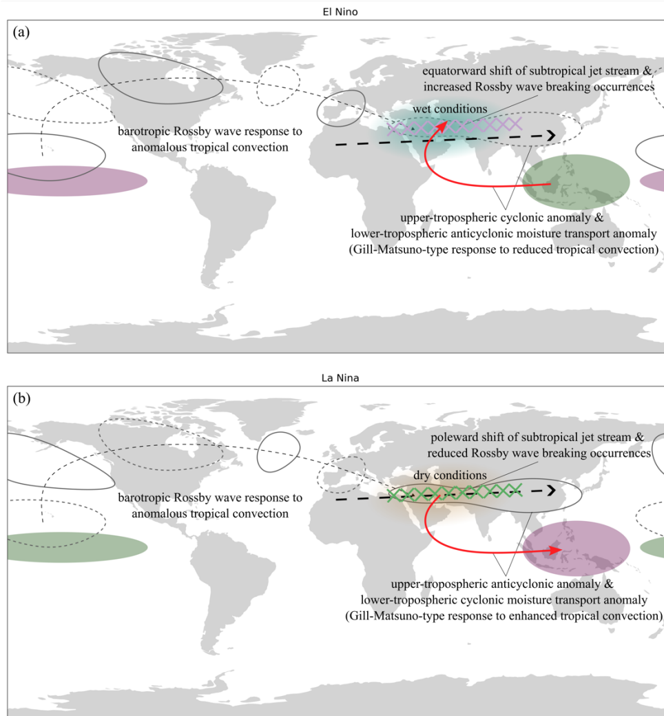
Figure 14.3. A schematic representation of three different mechanism through which ENSO modulates Middle Eastern precipitation variability during the cool season under (a) El Niño and (b) La Niña conditions: (1) a zonally symmetric displacement of the subtropical jet (cf. Kumar et al., 2016; Alizadeh-Choozari et al., 2018; Sandeep and Ajayamohan, 2018; Hoell et al., 2024) alongside modifications in Rossby wave breaking occurrences on the poleward flank and beneath the jet core, (2) a barotropic Rossby wave response arching from the tropical Pacific via the extratropics toward the Middle East (cf. Kumar et al., 2016; Hoell et al., 2013b; Hoell et al., 2015a; Abid et al., 2020)e.g., Wallace and, and (3) a regional baroclinic response in the tropical circulation extending westwards from the tropical Warm Pool, consistent with a Gill-Matsuno- type response (cf. Barlow et al., 2002; Hoell et al., 2012; Hoell et al., 2015a). This schematic is inspired by Fig. 9 from Barlow et al. (2016), showing mechanism (2) and (3) for La Niña conditions.
