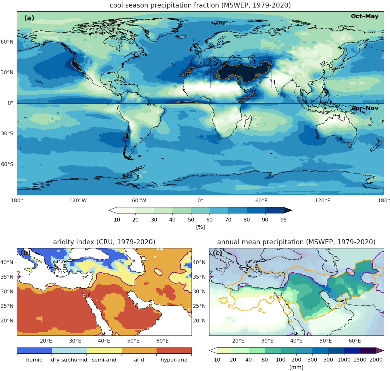
Figure 1. (a) Fractions of cool season precipitation from annual totals in MSWEP (1979-2020) whereby the cool season is defined from October to May in the Northern Hemisphere and from April to November in the Southern Hemisphere; (b) the aridity index across the Middle East region, computed from monthly CRU data (1979-2020) and defined as the ratio of precipitation to potential evapotranspiration; and (c) annual precipitation amounts in MSWEP (1979-2020) in shading, the 95% contour of the cool-season precipitation fraction from the annual total in orange, and the aridity index contour of 0.2, marking an arid to hyper-arid climate, in purple. Opaque shading highlights the target region used for computing spatially aggregated quantities in this study, while areas outside the target region are plotted in semi-transparent colors.
