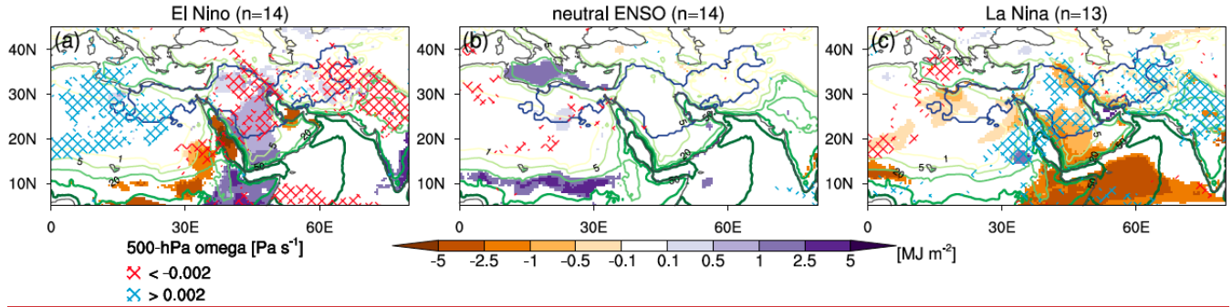
Figure 9. Composites of cool-season anomalies in I_{\max} [ \text{MJ m}^{-2} ] in colors for (a) El-Niño, (b) neutral ENSO, and (c) La Niña events. Hatching denotes regions with significant anomalies at the p < 0.05 level. Yellow-green contours show the climatological distribution of I_{\max} at intervals of 1, 5, 20, 50, and 100 \text{MJ m}^{-2} . Red and blue hatching mark regions with anomalous 500-hPa omega falling below -0.002 Pa s -1 (ascent) and exceeding 0.002 Pa s -1 (descent). Anomalies in I_{\max} and 500-hPa omega are only plotted where significant at the p < 0.05 level. The numbers in the figure title indicate the number of samples for each ENSO phase, and the blue contour highlights the region of interest.
