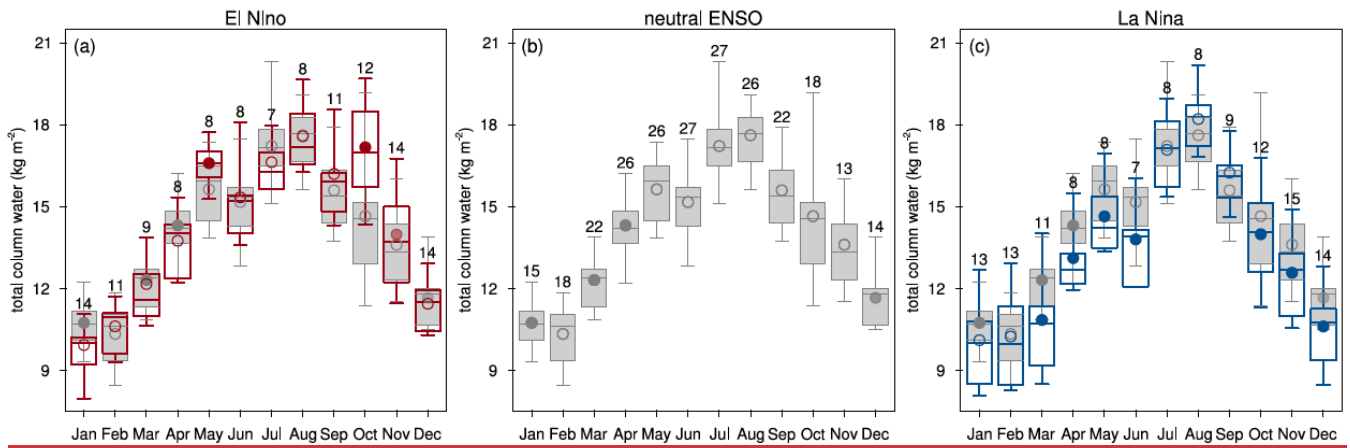
Figure 8. Monthly distribution of spatially aggregated non-detrended total column water for (a) El Niño, (b) neutral ENSO, and (c) La Niña conditions. The boxes denote the lower and upper quartiles, the whiskers the minimum and maximum values, the line in the middle the median, and the circle the mean, filled at the p < 0.05 significance level, semi-transparent at the p < 0.1 level, and open circles for non-significance anomalies relative to climatology. The sample sizes are indicated by the numbers above the boxes. The distribution of neutral ENSO conditions is overlaid in grey for reference for the El Niño and La Niña phases in (a) and (c).
