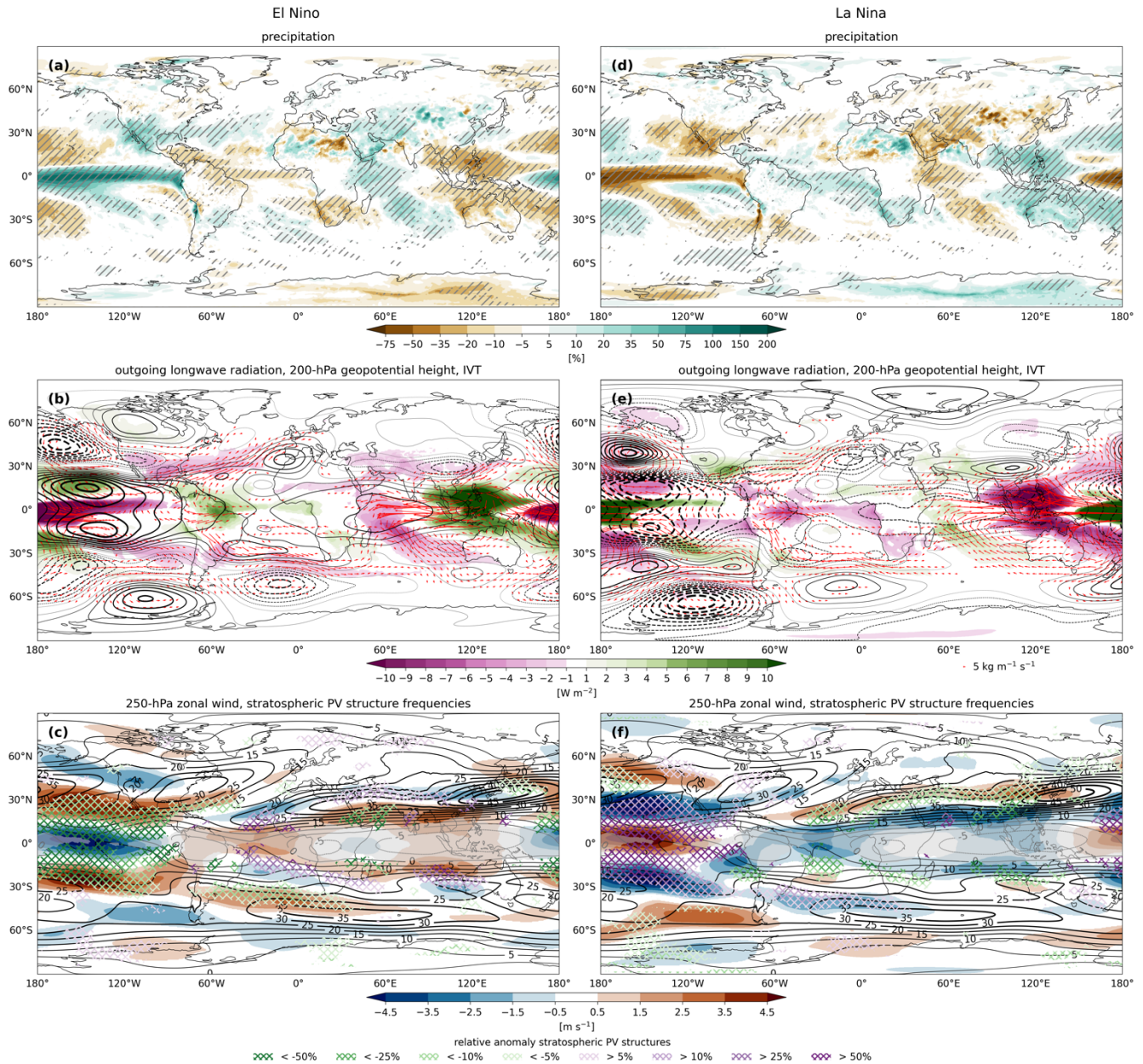
Figure 11. El Niño-e Composites of cool-season anomalies for (a-c) El-Niño and (d-f) La Niña . In (a,d) precipitation (%) in MSWEP, (b,e) top thermal radiation ( \text{W m}^{-2} ) in colors with negative anomalies corresponding to enhanced tropical convection and positive anomalies to reduced convection, 200-hPa geopotential height (m) contours at 4 gpm intervals with positive and negative values in solid and dashed lines, respectively, and vertically integrated horizontal water vapor transport ( \text{kg m}^{-1} \text{s}^{-1} ) in red vectors, and (c,f) 250-hPa zonal wind anomalies ( \text{m s}^{-1} ) in colors, the climatological mean of 250-hPa zonal wind in contours at 5 \text{ m s}^{-1} intervals, and relative anomalies in stratospheric PV structure occurrences, aggregated over 300-350K, in hatching, as indicated by the legend. Anomalies in top thermal radiation are only shown where considered significant at p < 0.05 and in zonal wind and Rossby wave breaking frequencies are shown only where considered significant at p < 0.1 .
