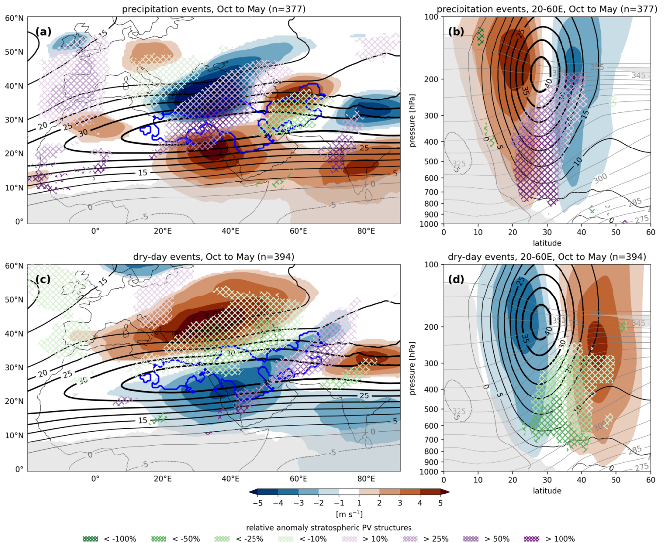
Figure 4. Composites of anomalies in zonal wind and Rossby wave breaking frequencies based on the onset of (a, b) precipitation events and (c, d) dry-day events. (a, c) 250-hPa zonal wind anomalies in colors and relative anomalies of stratospheric PV structure frequencies – aggregated over 300-350K - in hatching, as indicated by the legend. (b, d) The zonal mean (20-60E) zonal wind anomalies in colors and relative anomalies of stratospheric PV structure frequencies in hatching at pressure levels interpolated from data on isentropic surfaces between 275 and 360 K with 5 K intervals. These isentropic surfaces are plotted in grey contours. Zonal wind and Rossby wave breaking anomalies are shown only where considered significant at p < 0.05 based on a Monte Carlo test with 1,000 samples. Gray shading marks regions where climatological frequencies of vertically aggregated PV structure occurrences over 300-350K in (a, c) are below 25 counts and of PV structure occurrences in (b, d) fall below 5 counts. The region of interest is denoted in blue contours in (a, c) for reference. Sample sizes of precipitation and dry-day events are indicated in the figure titles.
