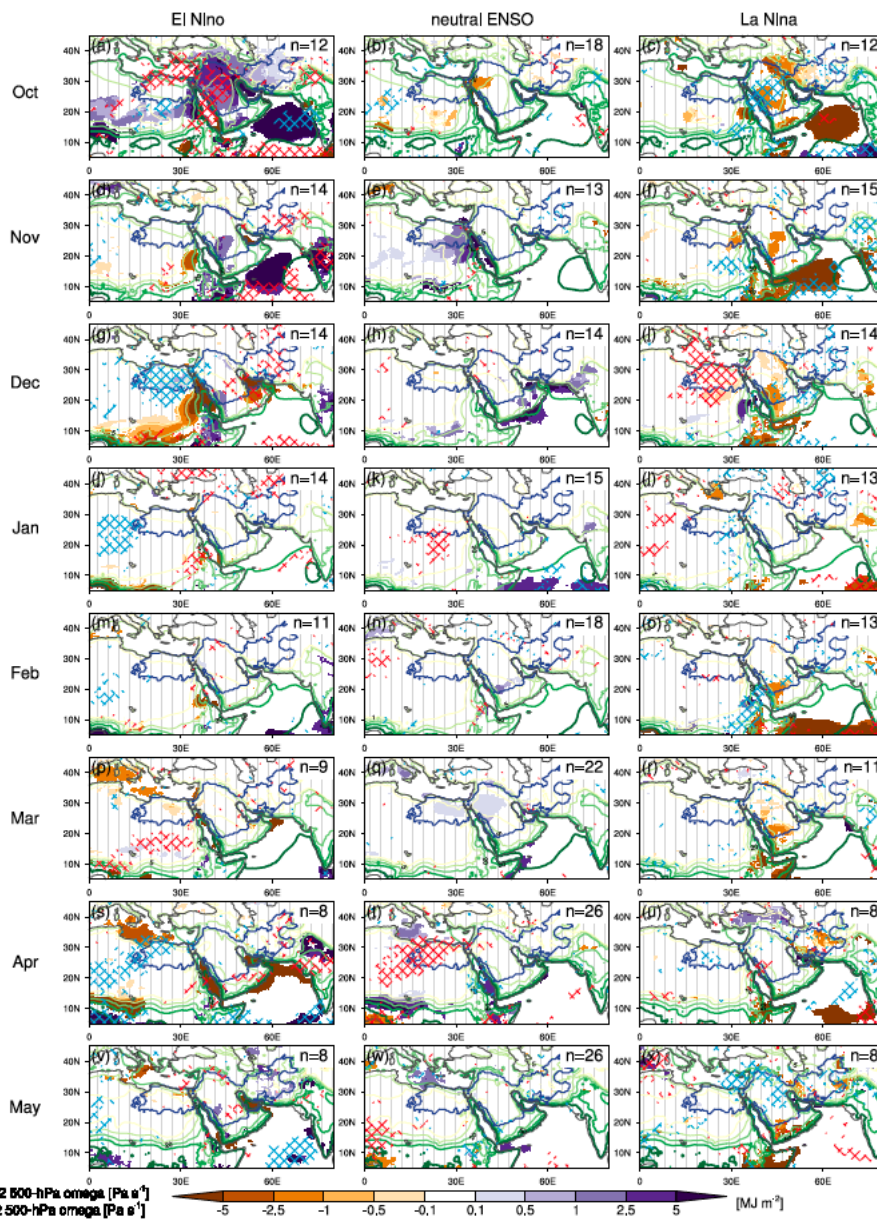
700 Figure A5. As Fig. 9 but for individual months from October to May in rows and the ENSO phases - warm, neutral, and cold - in columns. The ENSO phases are defined based on 3-monthly running mean SST anomalies in the Nino3.4 region. Sample sizes are indicated in text in the top right corner of each panel.
