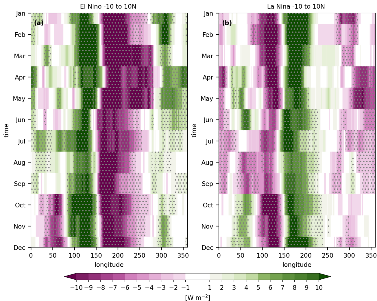
670 Figure 132. Hovmöller diagrams with anomalies in the Equatorial average (10°S-10°N) outgoing longwave radiation as a function of longitude and time for (a) El Niño and (b) La Niña conditions with negative anomalies corresponding to enhanced tropical convection and positive anomalies to reduced convection.
