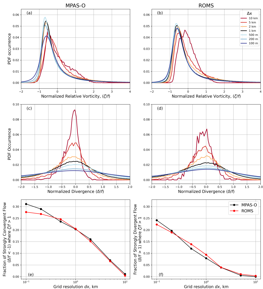
Figure 4. PDFs of surface relative vorticity (a,b) and surface divergence within fronts where \zeta > 1 (c,d) for MPAS-O (a,c) and ROMS (b,d) simulations over a range of spatial resolutions. Negative relative vorticity values correspond to a greater number of eddies, while positive vorticity values indicate a greater number of fronts. Fraction of strongly convergent (e) and strongly divergent (f) flow along fronts at all spatial resolutions for MPAS-O (black) and ROMS (red).
