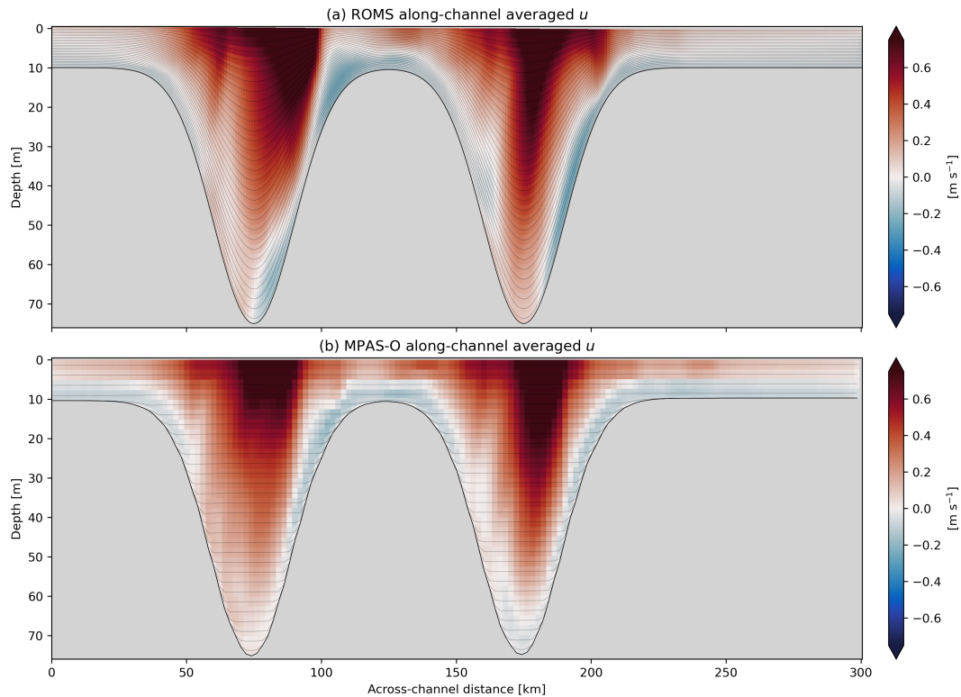
Figure A1. Cross-sections of along-channel averaged u velocity on Day 11 for (a) ROMS and MPAS-O. The thin black lines are the depth of layer centers.
