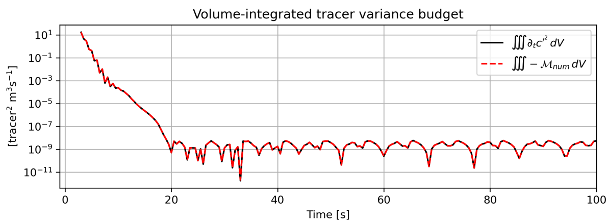
Figure B2. Volume-integrated tracer variance budget for the doubly periodic channel. The first several timesteps are omitted because \mathcal{M}_{num} is undefined at t = 0 and to account for the startup transient and two-step lag associated with the second-order Adams–Bashforth time-stepping scheme.
