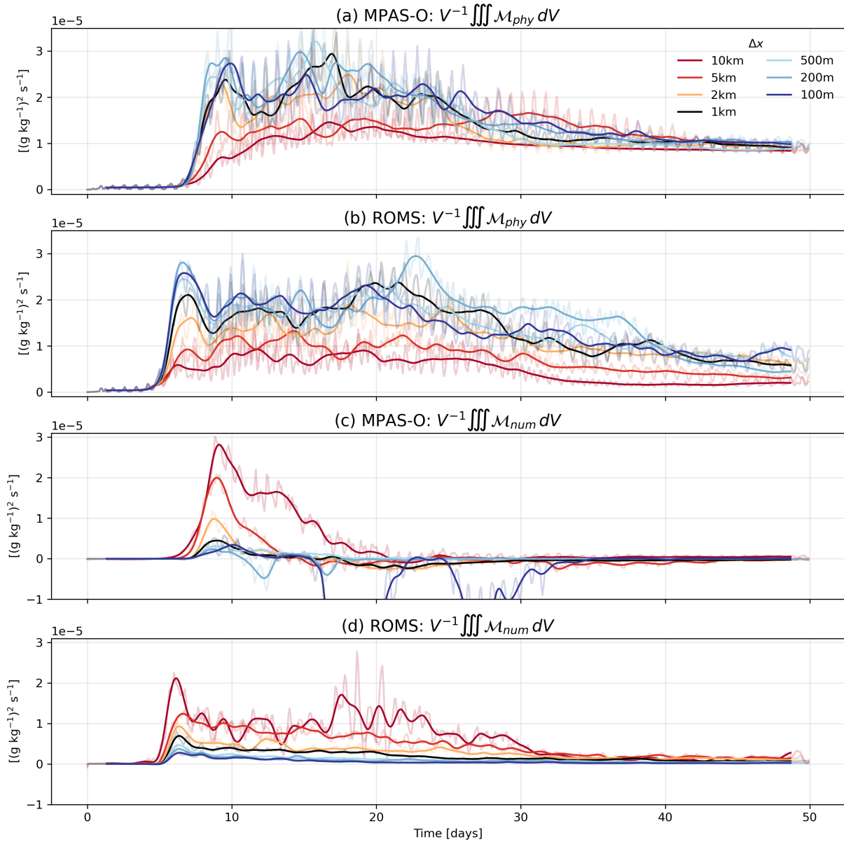
Figure 9. Time series of volume-averaged physical (a-b) and numerical (c-d) mixing for both models across all resolutions. Thicker lines are smoothed with a PL33 filter; thinner, fainter lines are the raw outputs.
