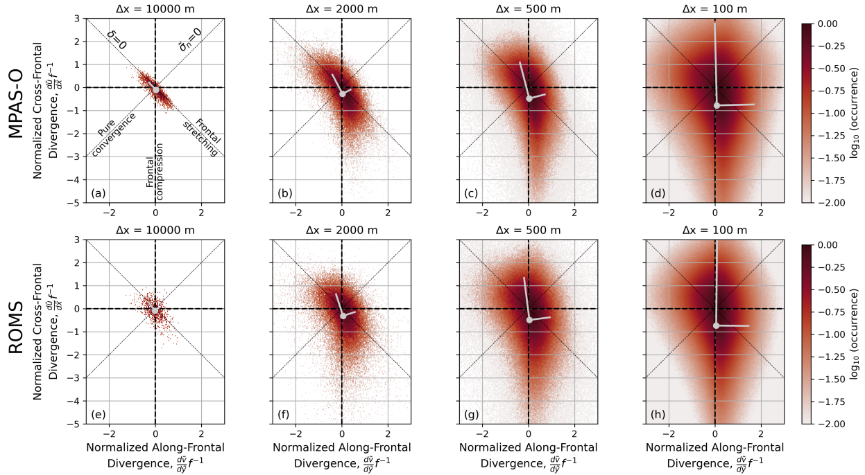
Figure 7. PDFs of normalized cross-frontal ( \frac{\partial \tilde{v}}{\partial x} f^{-1} ) vs along-frontal ( \frac{\partial \tilde{v}}{\partial y} f^{-1} ) surface velocity gradients for MPAS-O (a-d) and ROMS (e-h) simulations over a range of spatial resolutions, for all points associated with frontal regions ( \zeta f^{-1} > 1 ). Colorbar denotes, in log scale, the frequency of occurrence of these relationships. Gray lines emanating from the average of these distributions (gray dots) show the principal components of variability of the distribution. The negatively sloping dashed line corresponds to zero divergence ( \delta = 0 ), while the positively sloping dashed line corresponds to zero effective strain ( \tilde{\sigma}_n = 0 ).
