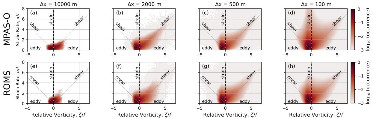
Figure 5. Joint PDFs of surface strain vs surface relative vorticity for MPAS-O (a-d) and ROMS (e-h) simulations over a range of spatial resolutions. Colorbar denotes, in log scale, the frequency of occurrence of these relationships. Diagonal gray lines emanating at 45^\circ to the left and right of the origin denote regions of shear while the vertical line identified at x=0 corresponds to pure strain. Regions below these diagonal lines correspond to eddies in the simulations.
