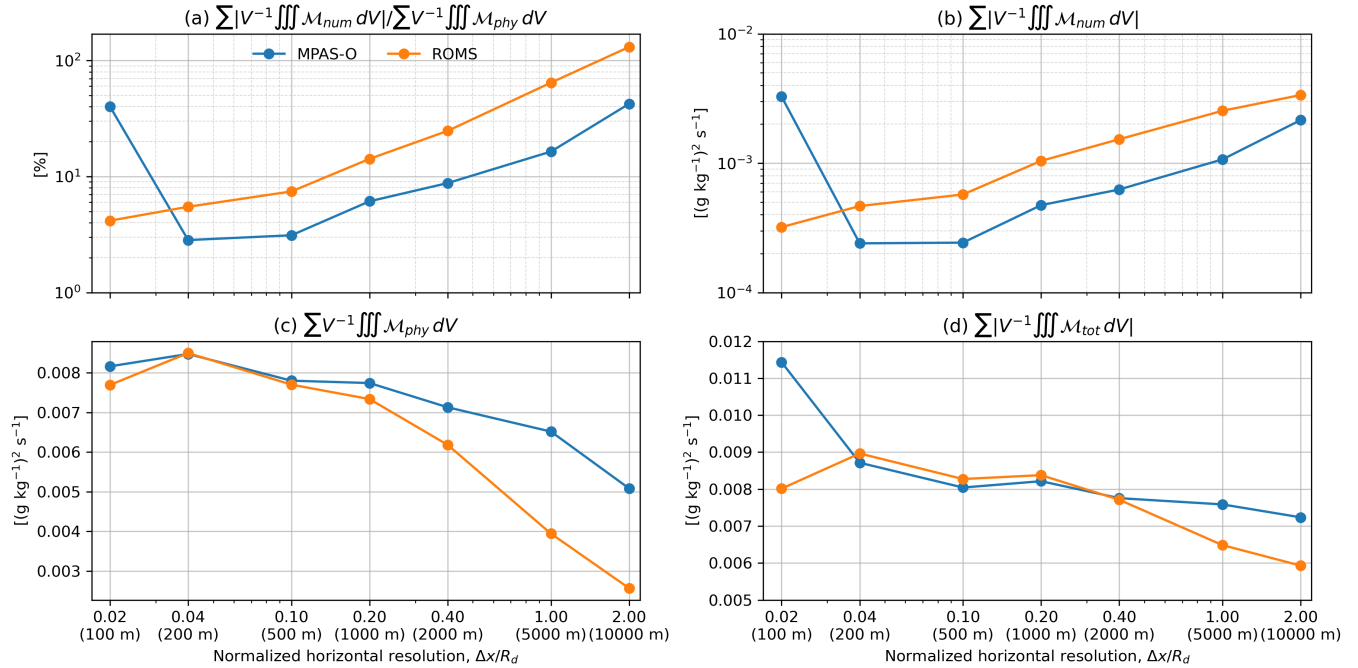
Figure 10. Time-summed volume-averaged mixing as a function of horizontal resolution normalized by the deformation radius (5 km). (a) Bulk ratio of numerical to physical mixing, (b) bulk numerical mixing, (c) bulk physical mixing, and (d) bulk total mixing. Absolute values are used for numerical and total mixing to account for strong anti-diffusion in MPAS-O.
