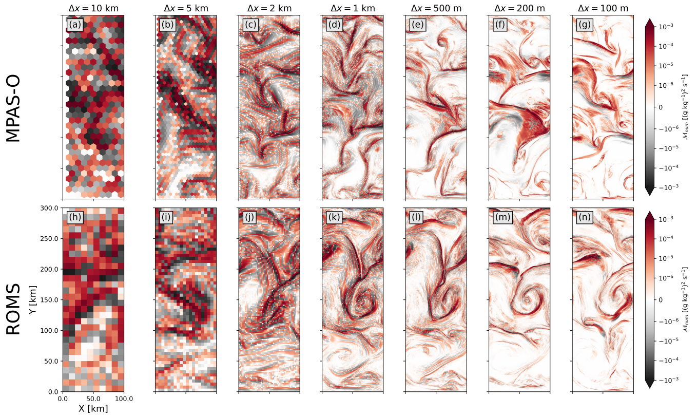
Figure 8. Surface numerical salinity mixing for MPAS-O (a-g) and ROMS (h-n) at the same time as Fig. 2.
