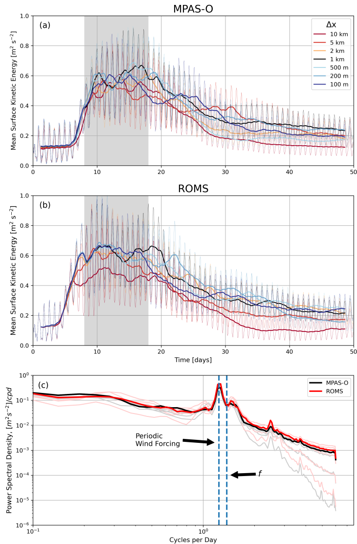
Figure 3. Time series of mean surface KE for MPAS-O (a) and ROMS (b) simulations over a range of spatial resolutions. Thicker lines show the KE time series smoothed with a PL33 filter while the lighter lines show the unfiltered data. Gray shaded regions in both (a) and (b) correspond to the average maximum 10-day period (Day 8-18) that is analyzed in the following histogram plots. Panel (c) shows the corresponding power density spectra of the time series for MPAS-O (black lines) and ROMS (red lines) where the thicker lines for both models show the 1 km spatial resolution spectra and thinner lines represent all other spatial resolutions. Dashed lines correspond to the frequencies of the periodic wind forcing and Coriolis term.
