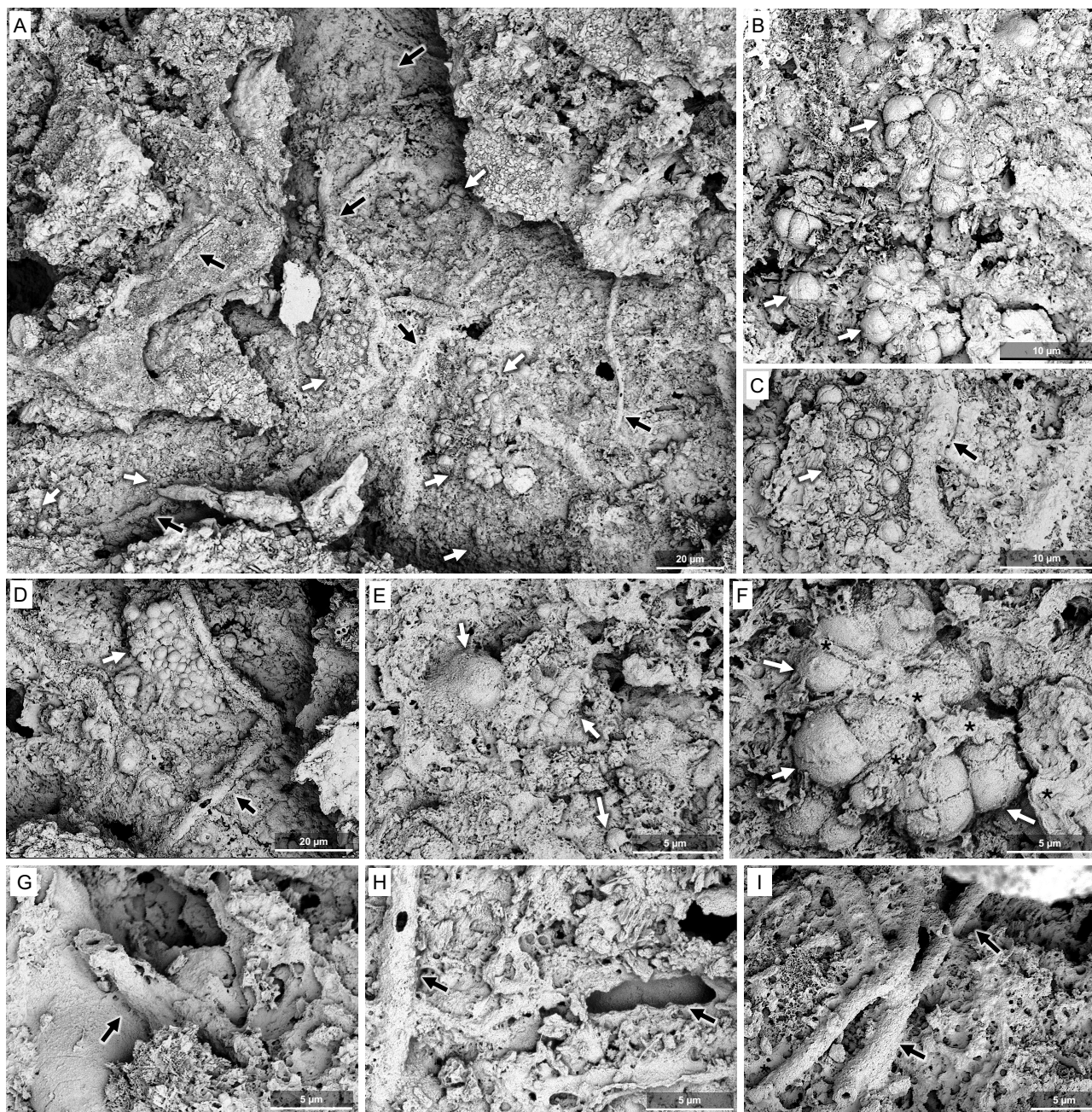
255 Figure 7: SEM images of the microbial biofilm (Layer 2) observed on the surface sample from the humid side of the Island of 260 Hawai'i. (A) General view of the crack within the surface layer exposing the biofilm; white arrows indicate coccid biomorphs and black arrows filamentous biomorphs. (B) Details of a group of coccoid biomorphs (white arrows) emerging from copious EPS matrix. (C, D) Details of a group of coccoid structures (white arrow) showing calcified EPS septa (black asterisks) and a filamentous biomorph (black arrow) in two different locations of the biofilm area. The quadrilobed biomorphs are similar to the modern colonial genus Gleocapsa . (E) Details of a group of coccoid biomorphs (white arrows) and hollow filaments (black arrow). (F) Details of a group of coccoid biomorphs (white arrows) and abundant EPS in a different spot of the biofilm area. (G-I) Mineralised hollow structures compatible with calcified sheaths of filamentous bacteria (black arrows). All images from Site M0104A, core 12.
