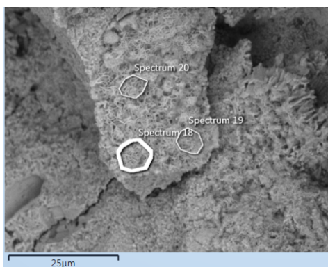
Fig. C2: EDX spectra of flaky minerals, sample M0104A-012R-1, 146-150 cm.
