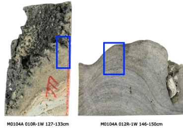
205 Figure 4: Samples studied by SEM; blue quadrangles indicate the two subsamples prepared for SEM microscopy.
