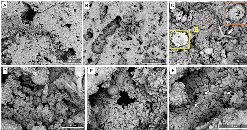
480 Figure 8: SEM images of samples from the Kawaihae site, i.e., the dry side of the Island of Hawai'i. (A, B) Low magnification 485 micrographs of the vertically cut sample. (C) Assemblage of structures of possible biological origin found on the surface of the sample; torn sheet-like matrices compatible with desiccated EPS (black asterisks), a spherical hollow structure consistent with a lithified coccolith microorganism (orange square), a calcareous sponge spicule (white arrow) and a coccolith flowery plate possibly affiliated to Discoasteraceae (yellow square). (D) Peloidal texture with abundant spheroidal structures coated in fine crystals. (E) Cavity exposed by the cut, covered in a microcrystalline coat. (F) Filaments consistent with EPS strings, indicated by white arrows (F). All images from Site M0097B, core 7.
