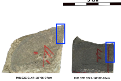
205 Figure 4: Samples studied by SEM; blue quadrangles indicate the two subsamples prepared for SEM microscopy.
