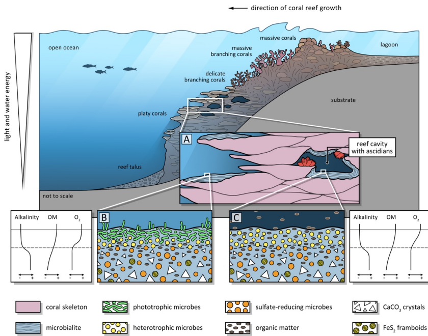
600 Figure 9: Schematic diagram of loci of microbialite formation in a coral reef under slightly shaded euphotic versus oligophotic cryptic conditions. Section through a coral reef, (A) euphotic versus cryptic setting in a cavity, (B) close-up of euphotic setting with cyanobacterial mat at the surface of the microbialite, (C) close-up of detrital organic matter-driven microbial mat in a cavity. Diagrams illustrating gradients in alkalinity, organic matter, and oxygen throughout the upper layers of the microbial mats.
