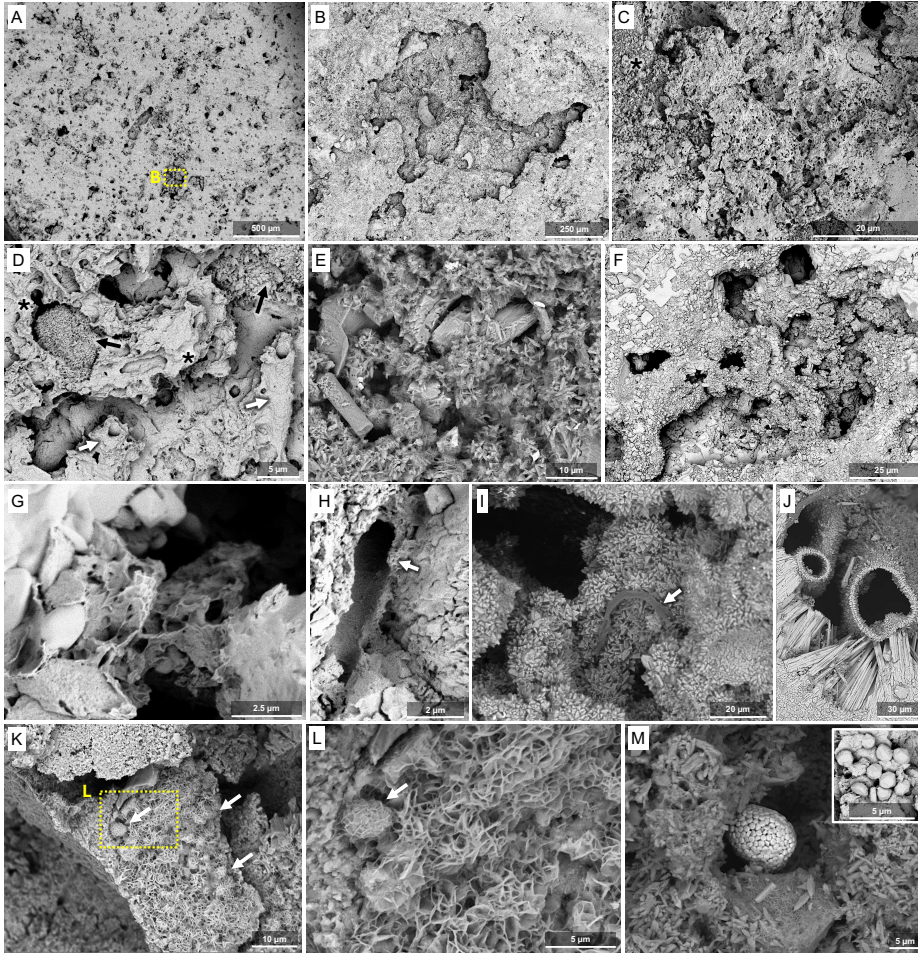
275 Figure 6: SEM images of samples from the humid side of the Island of Hawai'i. (A) Low magnification image of cross-section of the fine-crystalline surface. (B) Surface sample showing a collapsed area on the sample surface, revealing underlying Layer 2. (C) Higher magnification of the fine-crystalline surface layer material consistent with torn, desiccated, and mineralised EPS. (D) Mineralised EPS matrix (black asterisks) with mineralised filamentous microbial structures emerging from deeper layers as hollow tubes (white 280 arrows), and residual embedded grains (black arrows). (E) Acicular microcrystals. (F) Porous spaces coated by microcrystals. (G) Details of torn, laminated matrix-like material consistent with fossilized EPS residues. (H) Hollow calcified sheaths of filamentous
