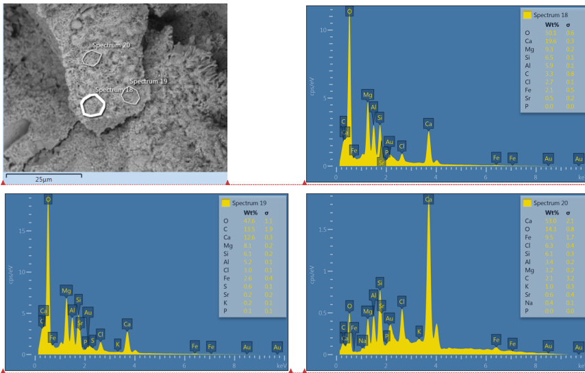
Fig. C2: EDX spectra of flaky minerals, sample M0104A-012R-1, 146-150 cm.
