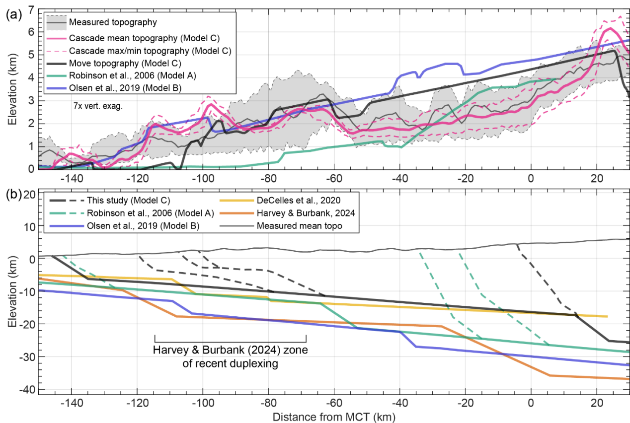
Figure 78: Models of the Simikot transect in western Nepal. (a) Topographic swath (grey) and predicted topographies generated by the different models. (b) Comparison between proposed geometries of the MHT. Dashed lines show the young (<1 Ma) out-of-sequence faults of Models A and C.
