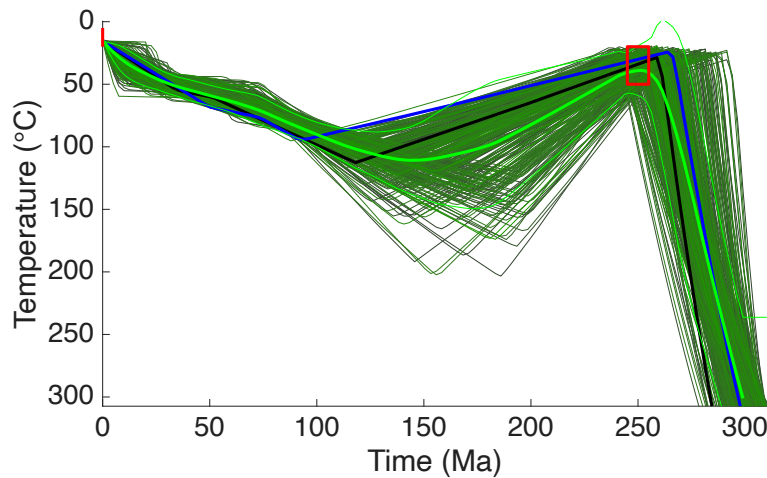
Figure 7. Modelled tT-path of sample 22BGE055T using apatite fission track and in-situ (U-Th)/He data. Paths are color-ranked according to their fit from black to light green with the thick green line is the weighted mean cooling paths with 95% CI (thin green lines). The tT-path that fit best the data is shown in blue (highest summed GOF) and black (most input data fitted with GOF>0.05). The red box is constraining the cooling paths to represent late Permian exhumation to near surface temperatures.
