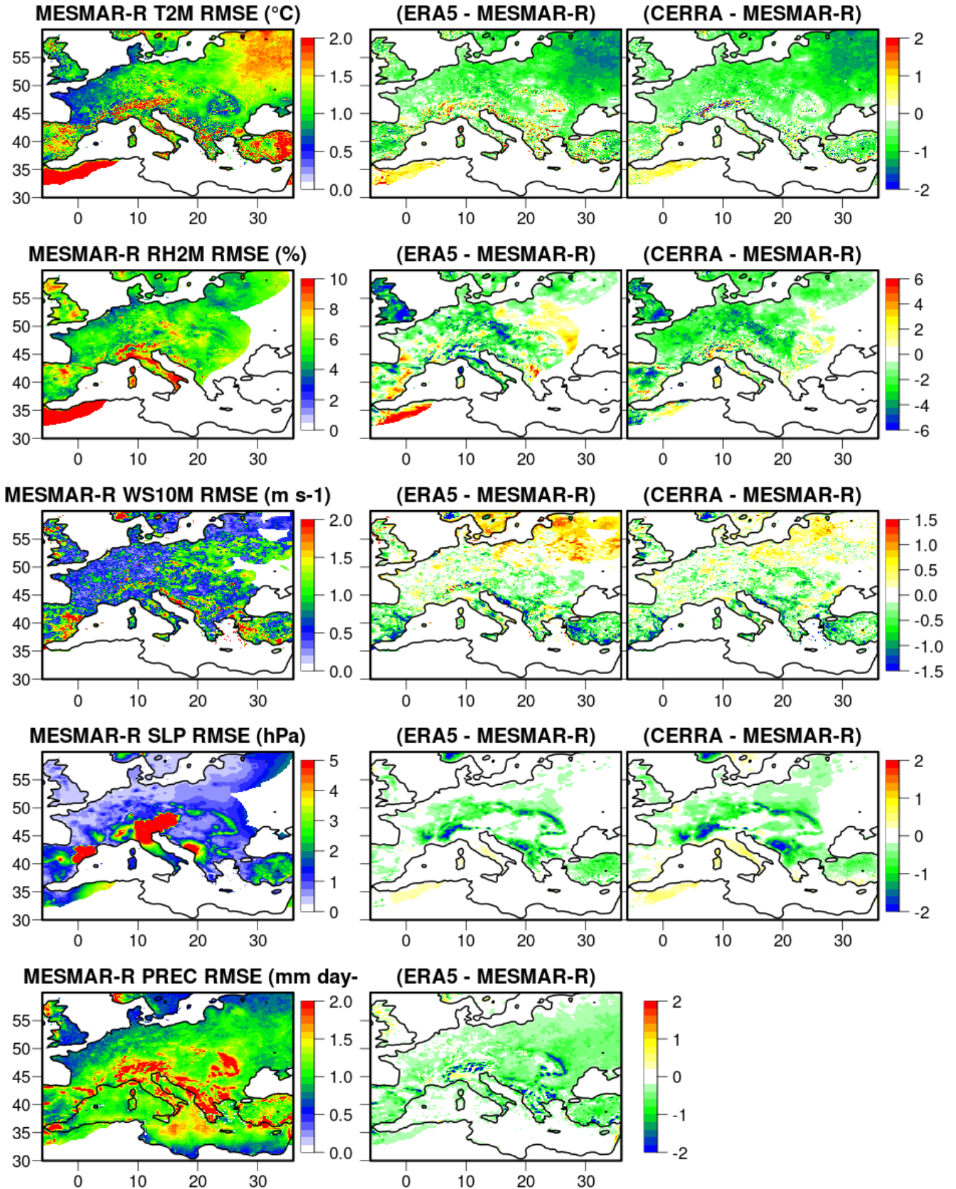
Figure 3. Maps of RMSE against atmospheric near-surface gridded observations (T2M in °C, RH2M in %, WS10M in m s -1 , SLP in hPa, and PREC in mm day -1 ), in comparison with other state-of-the-art reanalyses. Left panels show the MESMAR-R RMSE, while middle and right panels show the RMSE difference between either ERA5 or CERRA and MESMAR-R (where positive, MESMAR-R provides the smallest RMSE). The calculation covers the period 2000-2020.
