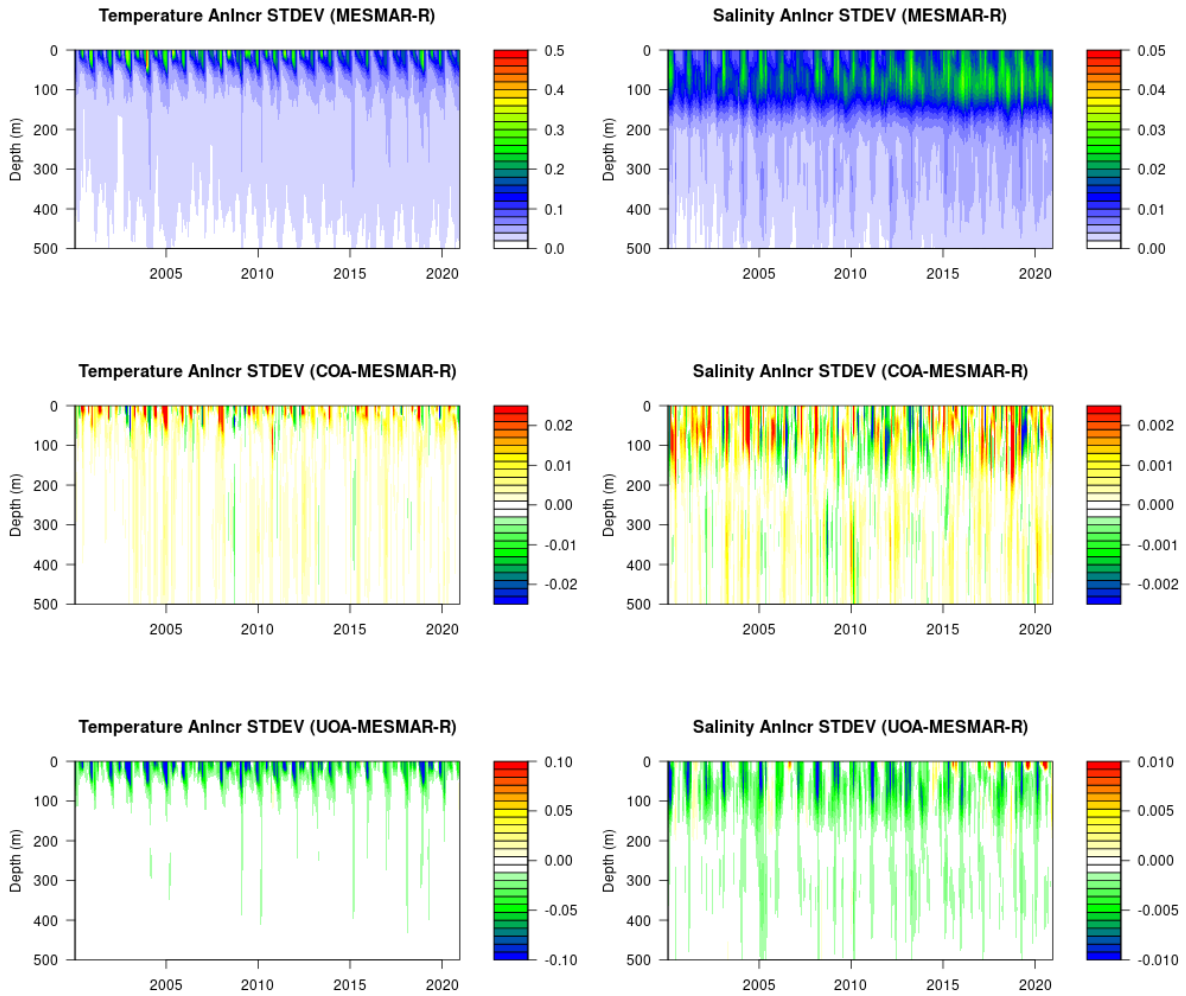
Figure 12. Hovmöller diagram (time-depth) of the analysis increment spatial standard deviation for MESMAR-R and the other two experiments with ocean data assimilation enabled. The period is 2000-2020.
