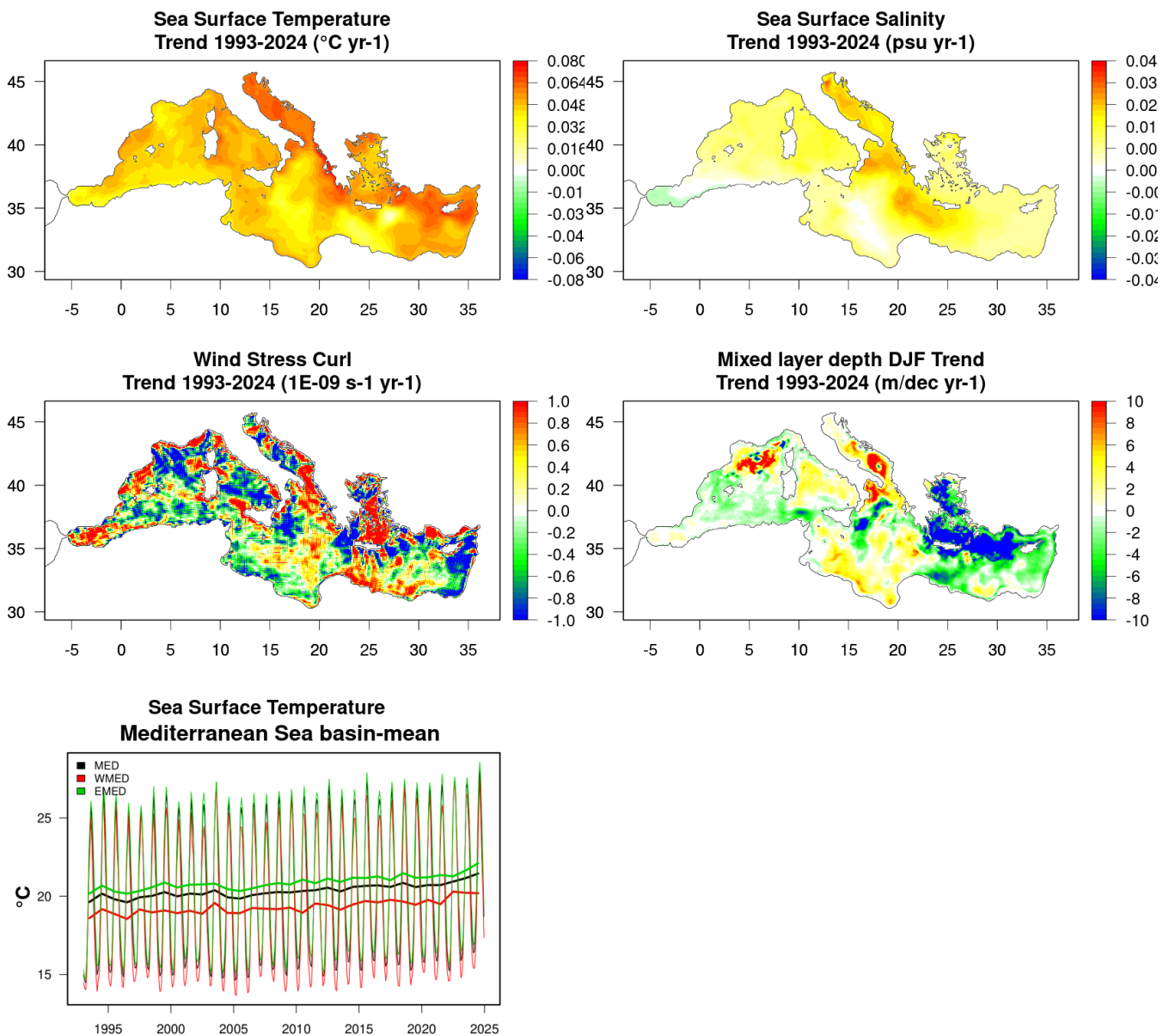
538 Figure 15. Maps of linear trends (1993-2024) for selected variables, and time series of SST, from MESMAR-R.
