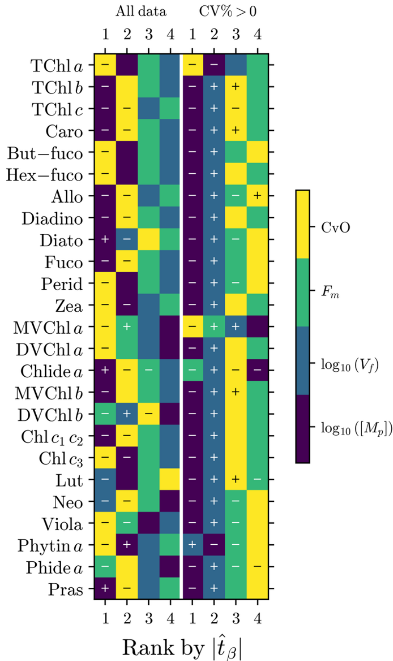
705 Figure B1. Variable importance rankings from multivariate regressions predicting pigment precision for full dataset (left) and censored data excluding invariant replicates (right). Rankings (1–4) based on absolute t -statistics ( \hat{t}_\beta ). Symbols indicate effect direction: '+' increases CV %, '-' decreases CV %, blank = non-significant ( \alpha = 0.05 ). Variables: \log_{10}(M_p) = pigment mass, \log_{10}(V_f) = filtered volume, F_m = microplankton fraction, CvO = coastal (0) vs. oceanic (1). Colors denote variables as per the colorbar.
