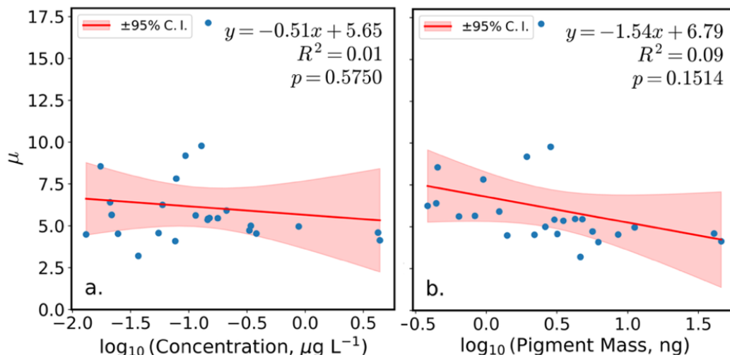
Figure 4: Mean coefficient of variation percentage (CV %) precision versus (a.) mean log 10 -transformed pigment concentration, and (b.) log 10 -transformed mean pigment mass. The adjusted R^2 quantifies goodness of fit, while the p -value tests significance of the slope.
