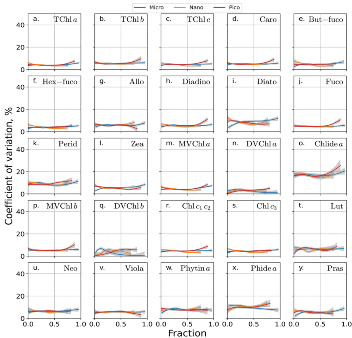
Figure A1. LOESS regression fits of sample precision (all data) versus estimated phytoplankton size fraction: micro (>20 \mu\text{m} ), nano (2-20 \mu\text{m} ), and picoplankton (<2 \mu\text{m} ) eqs. 2-4. Shaded area contains 95 % confidence bands.
