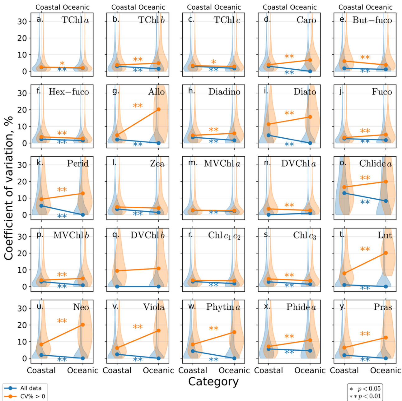
Figure 9: Lines depict the median sample precision (CV %) for phytoplankton pigments from coastal (<200km from shore) versus oceanic (>200km). Differences assessed using Mann-Whitney U test on full dataset (blue) and subset with CV > 0 only (orange). Violin plots depict CV% distribution per category. Comparisons marked “*” and “**” indicate statistically significant precision differences between coastal and oceanic at \alpha=0.05 and \alpha=0.01 , respectively.
