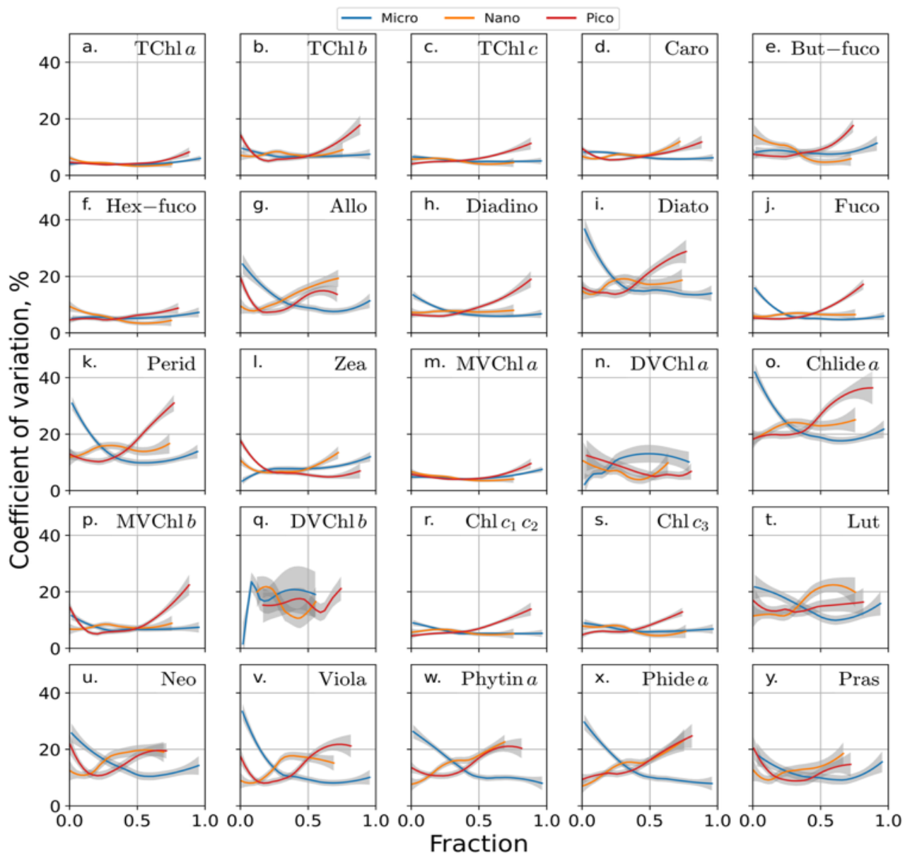
Figure 8: LOESS regression fits of replicate sample precision (CV % > 0) versus estimated phytoplankton size fraction: micro (>20 \mu\text{m} ), nano (2-20 \mu\text{m} ), and picoplankton (<2 \mu\text{m} ) eqs. 2-4. Shaded area contains 95 % confidence bands.
