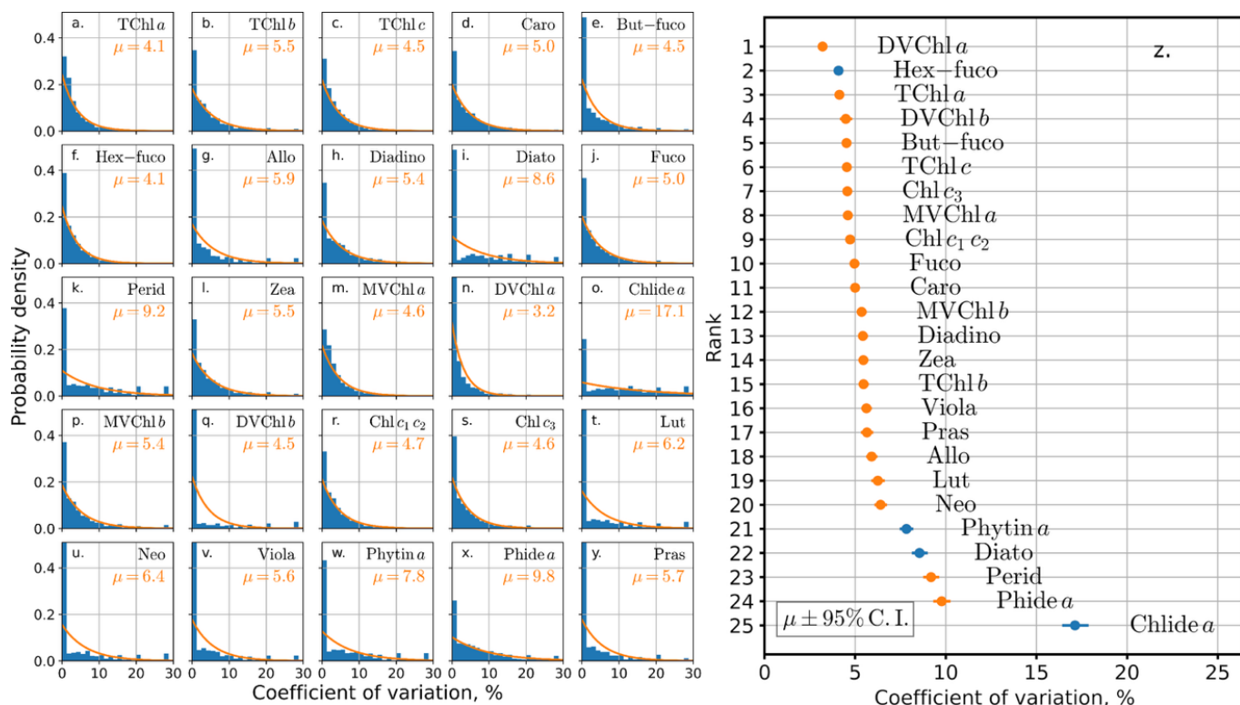
Figure 3: a-y) Histograms of replicate sample precision (CV %) calculated for each phytoplankton pigment analyzed by HPLC from 2011-2022. Overlaid in orange is the exponential probability density function for each pigment, and \mu is mean precision. Panel (z.) shows pigments ranked by precision. Blue symbols mark instances of non-overlapping confidence intervals with the next-lowest pigment.
