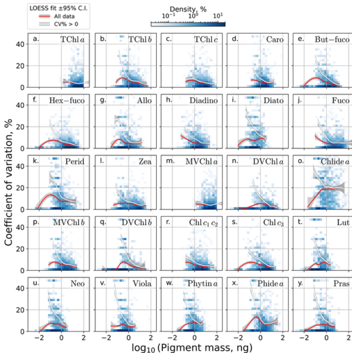
395 Figure 6. Replicate sample precision (CV %) versus \log_{10} -transformed pigment mass injected for each phytoplankton pigment. LOESS regression fits on all data (red line) and CV % > 0 only data (white line), with 95 % CIs shaded. 2D histograms display CV % sample density, with color bar showing percent sample density.
